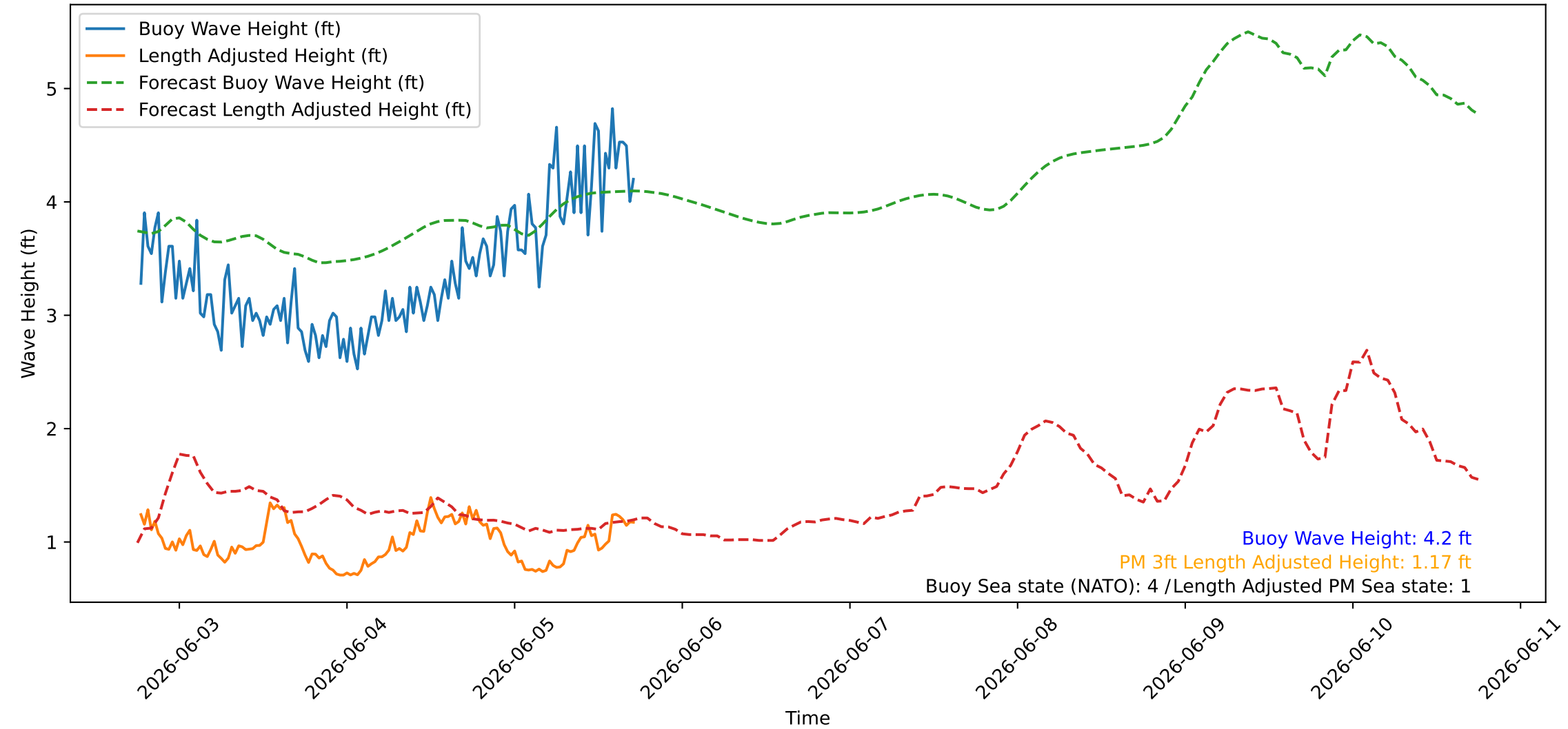
Wave Heights over Time for Red Beach at 2026-06-05 18:00:46
