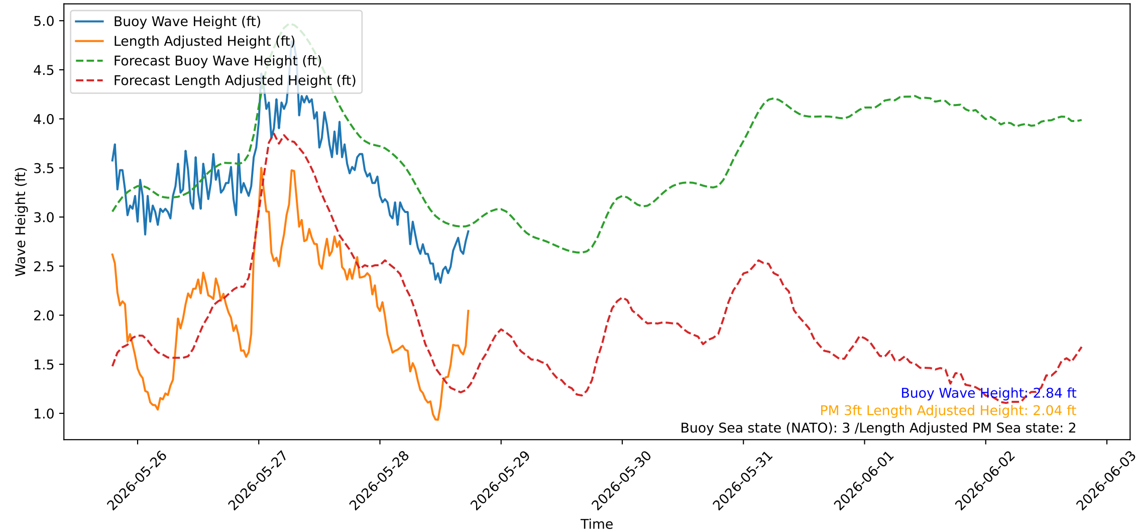
Wave Heights over Time for Red Beach at 2026-05-28 18:30:38
