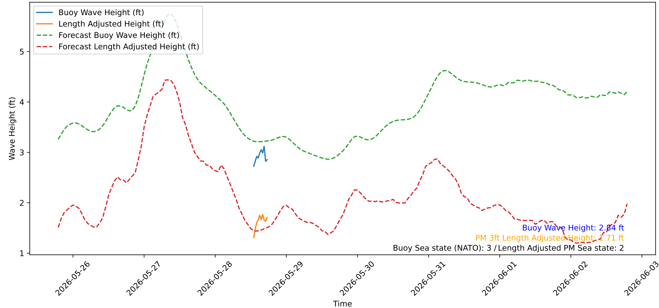
Wave Heights over Time for Oceanside Harbor at 2026-05-28 18:30:19
