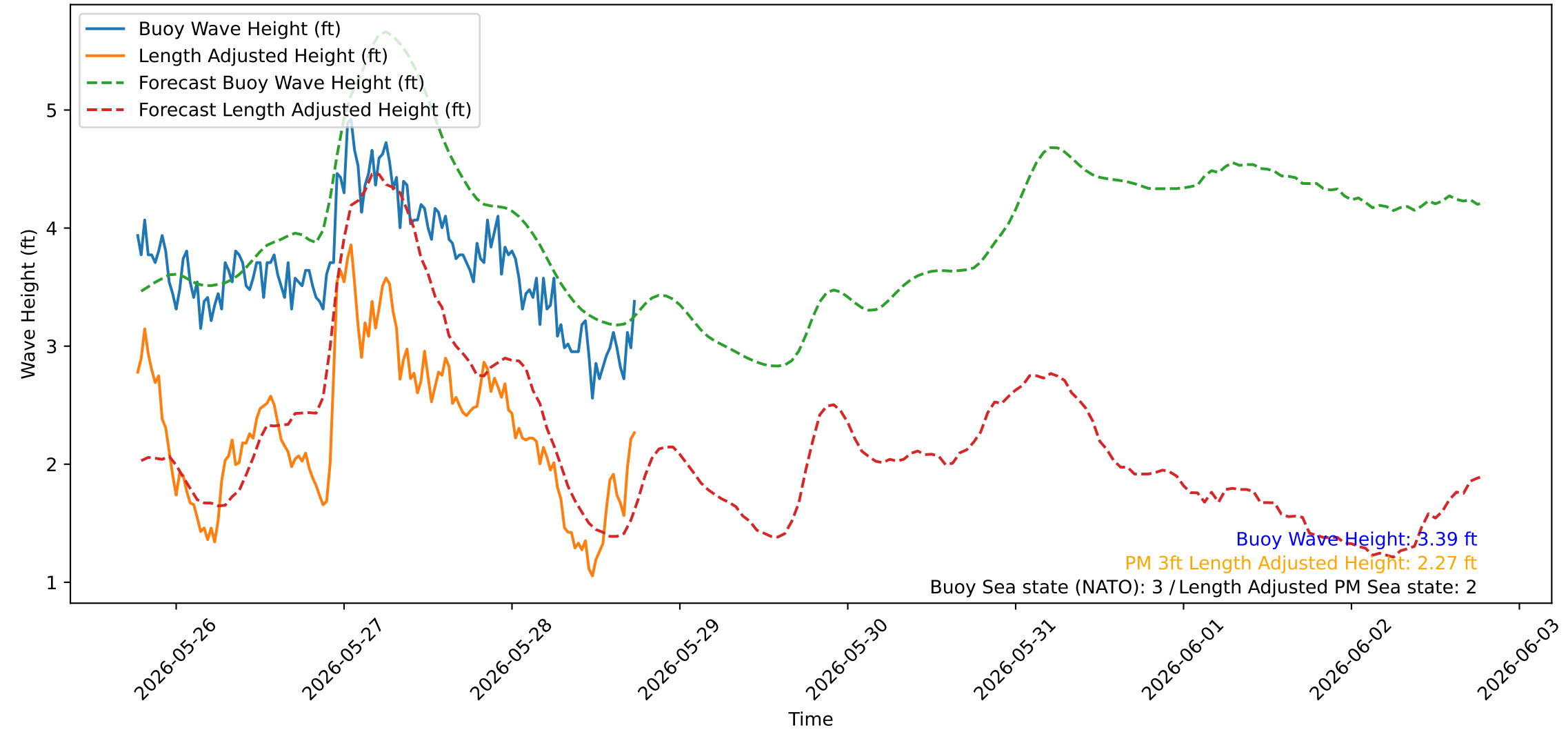
Wave Heights over Time for Green Beach at 2026-05-28 18:31:00
