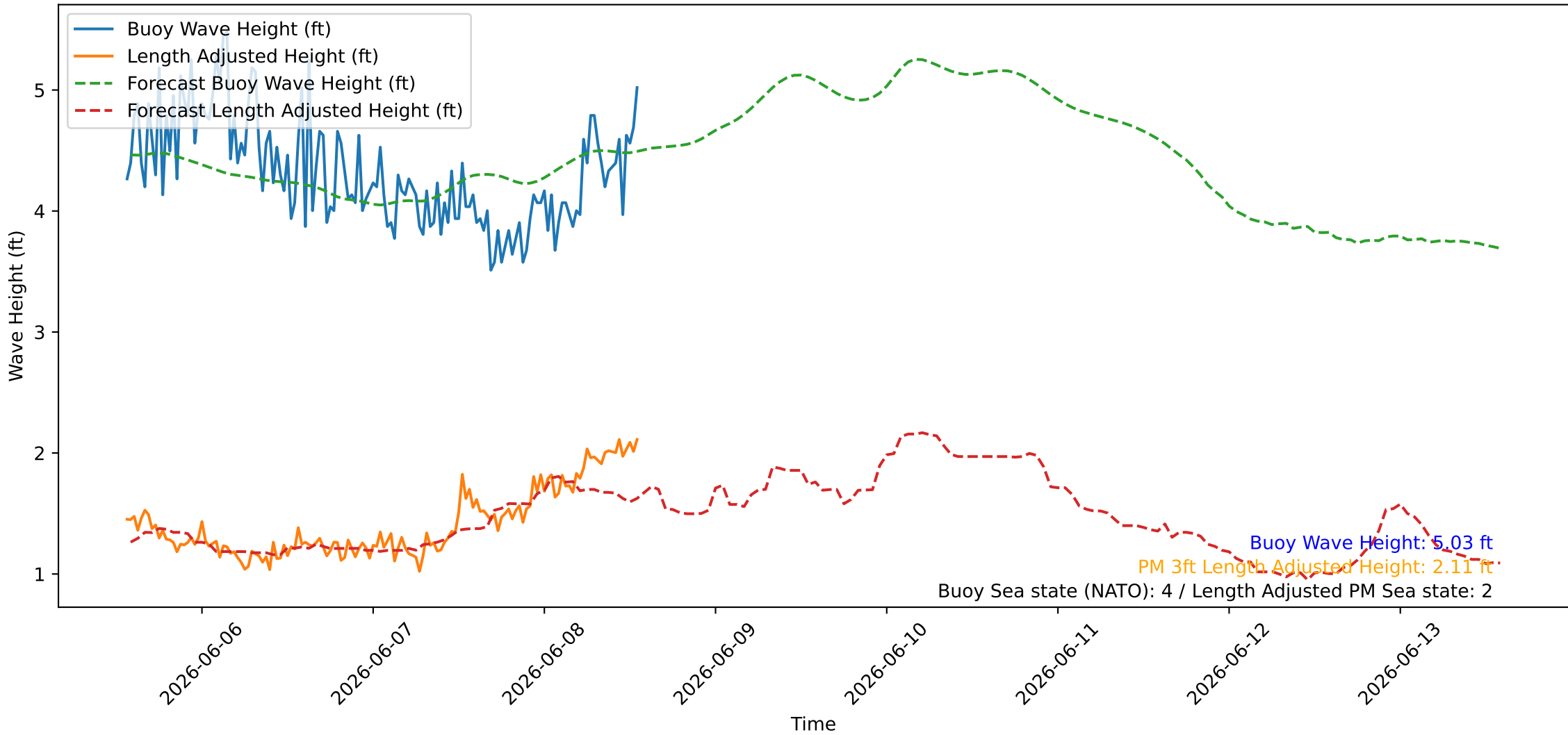
Wave Heights over Time for Oceanside Harbor at 2026-06-08 13:30:26
