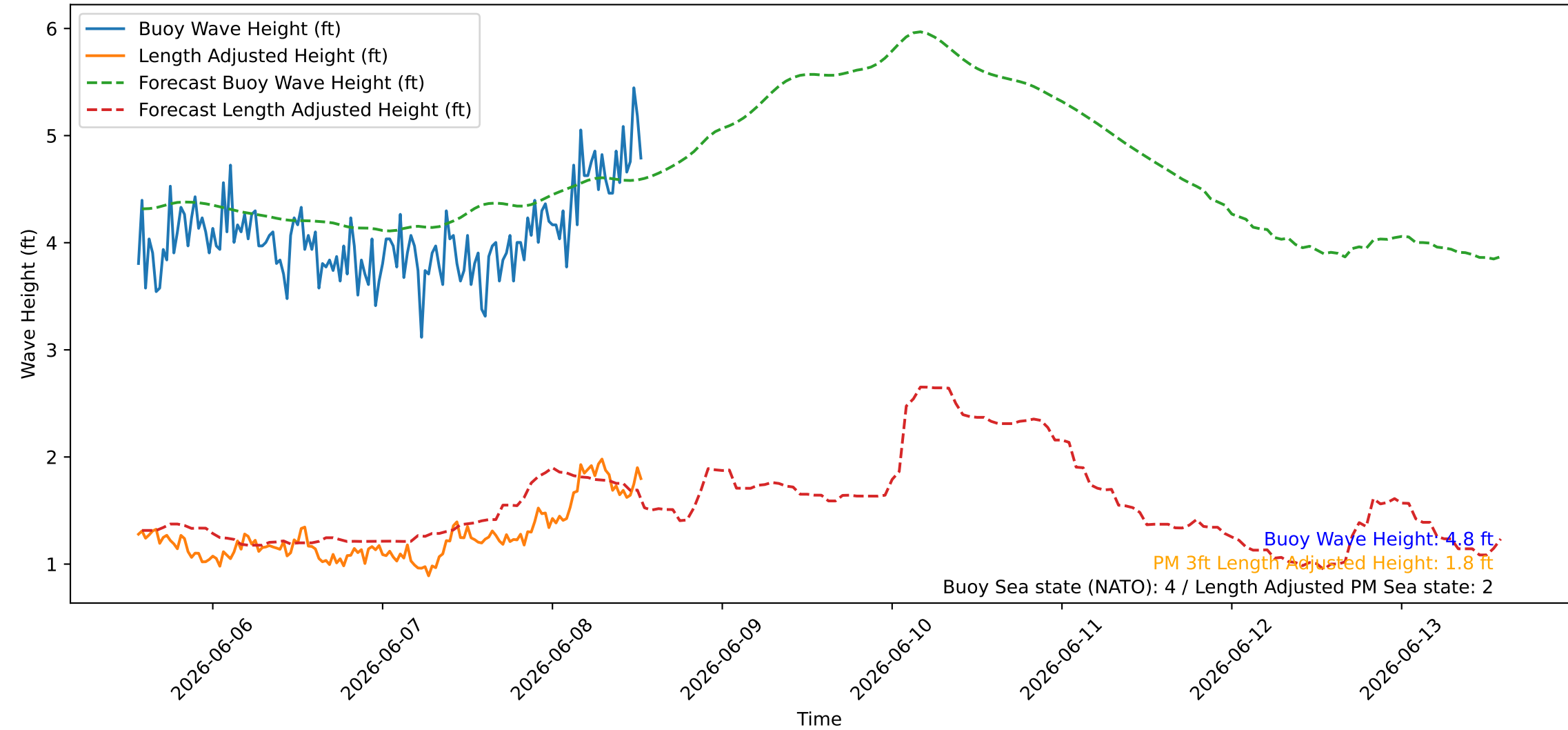
Wave Heights over Time for Green Beach at 2026-06-08 13:31:08
