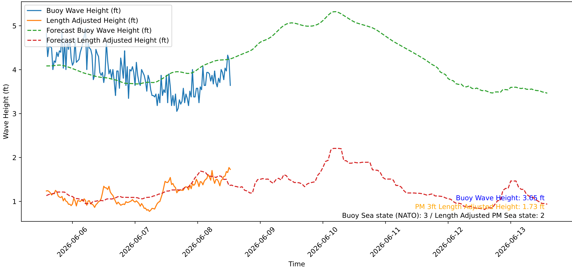
Wave Heights over Time for Red Beach at 2026-06-08 13:30:46
