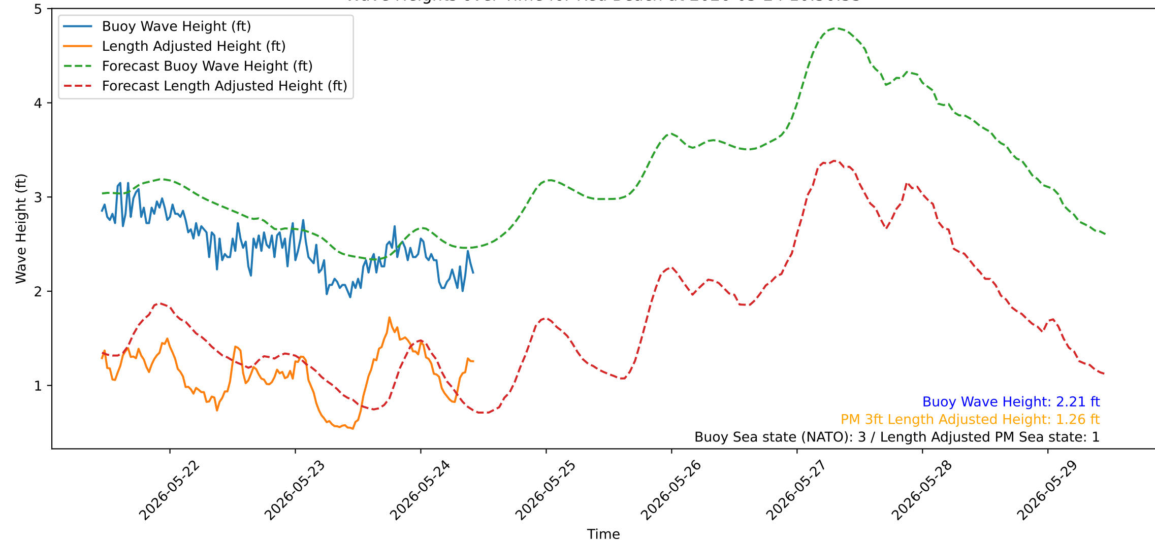
Wave Heights over Time for Red Beach at 2026-05-24 10:50:53
