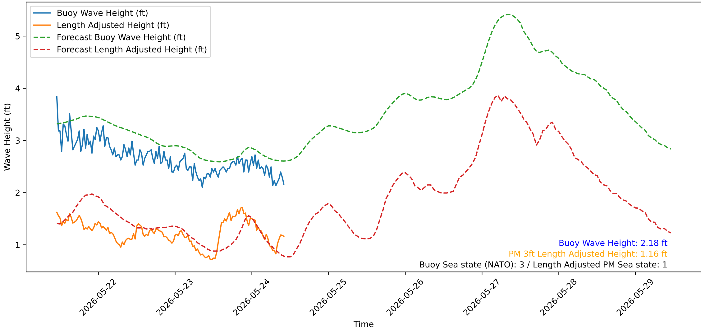
Wave Heights over Time for Oceanside Harbor at 2026-05-24 10:50:32
