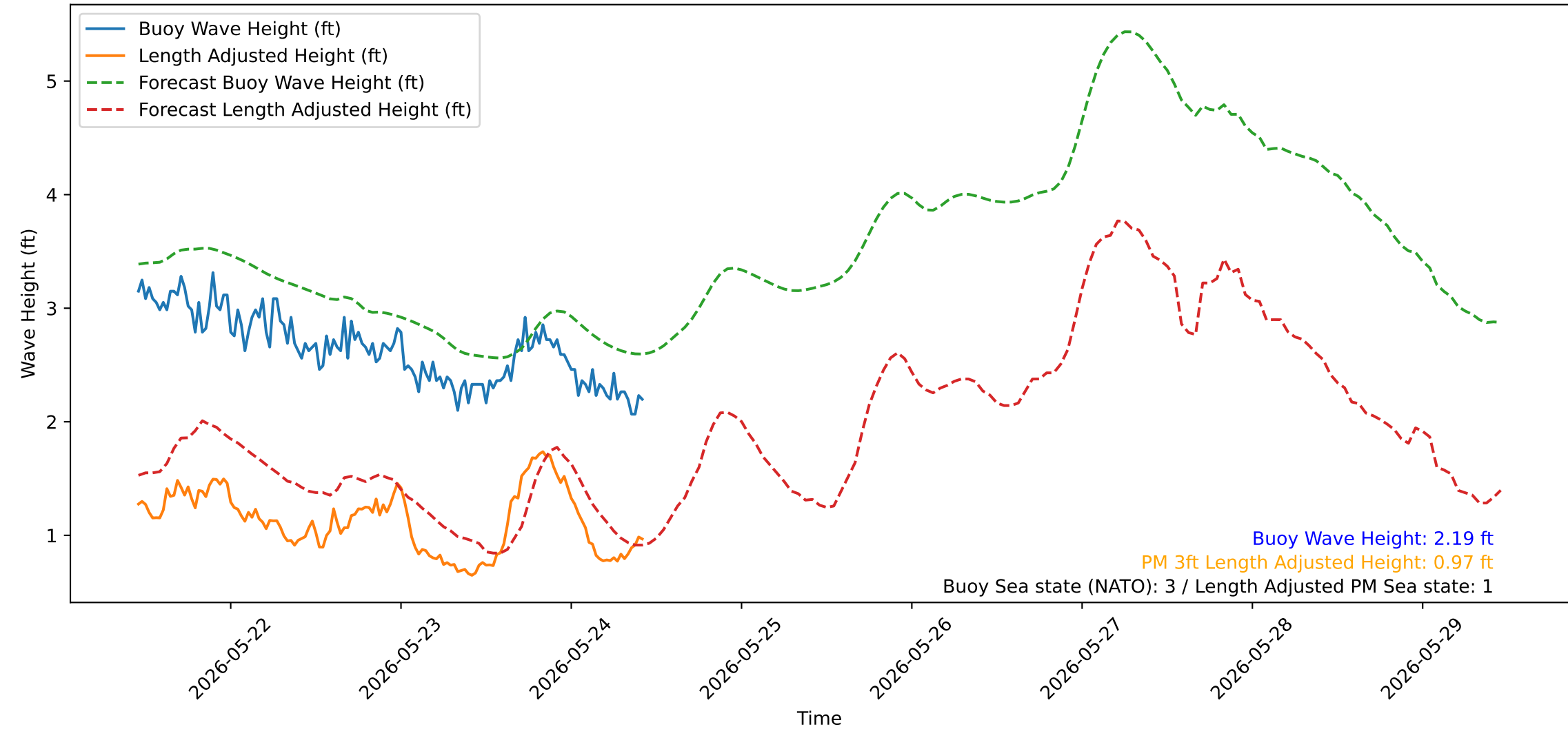
Wave Heights over Time for Green Beach at 2026-05-24 10:51:15
