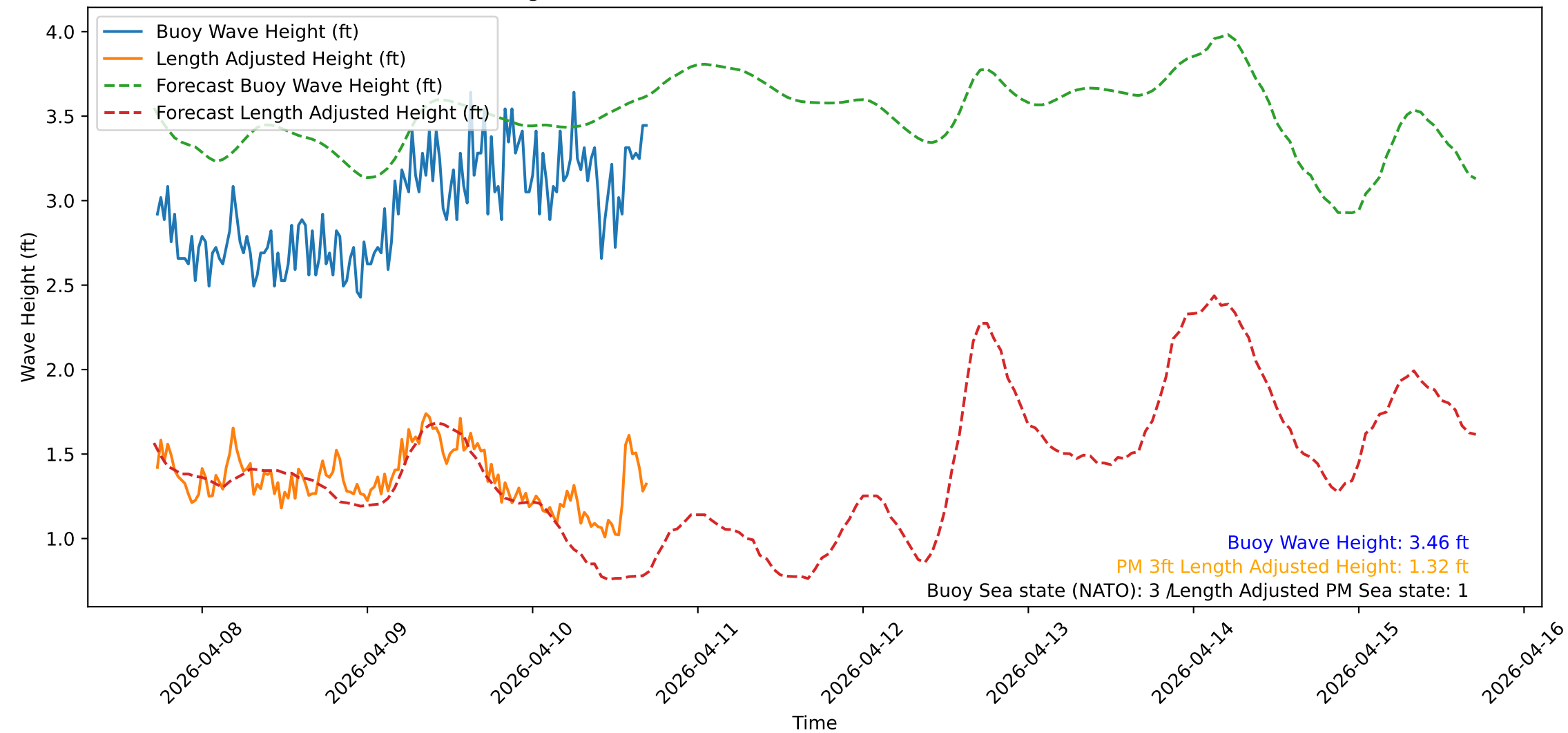
Wave Heights over Time for Oceanside Harbor at 2026-04-10 17:20:31
