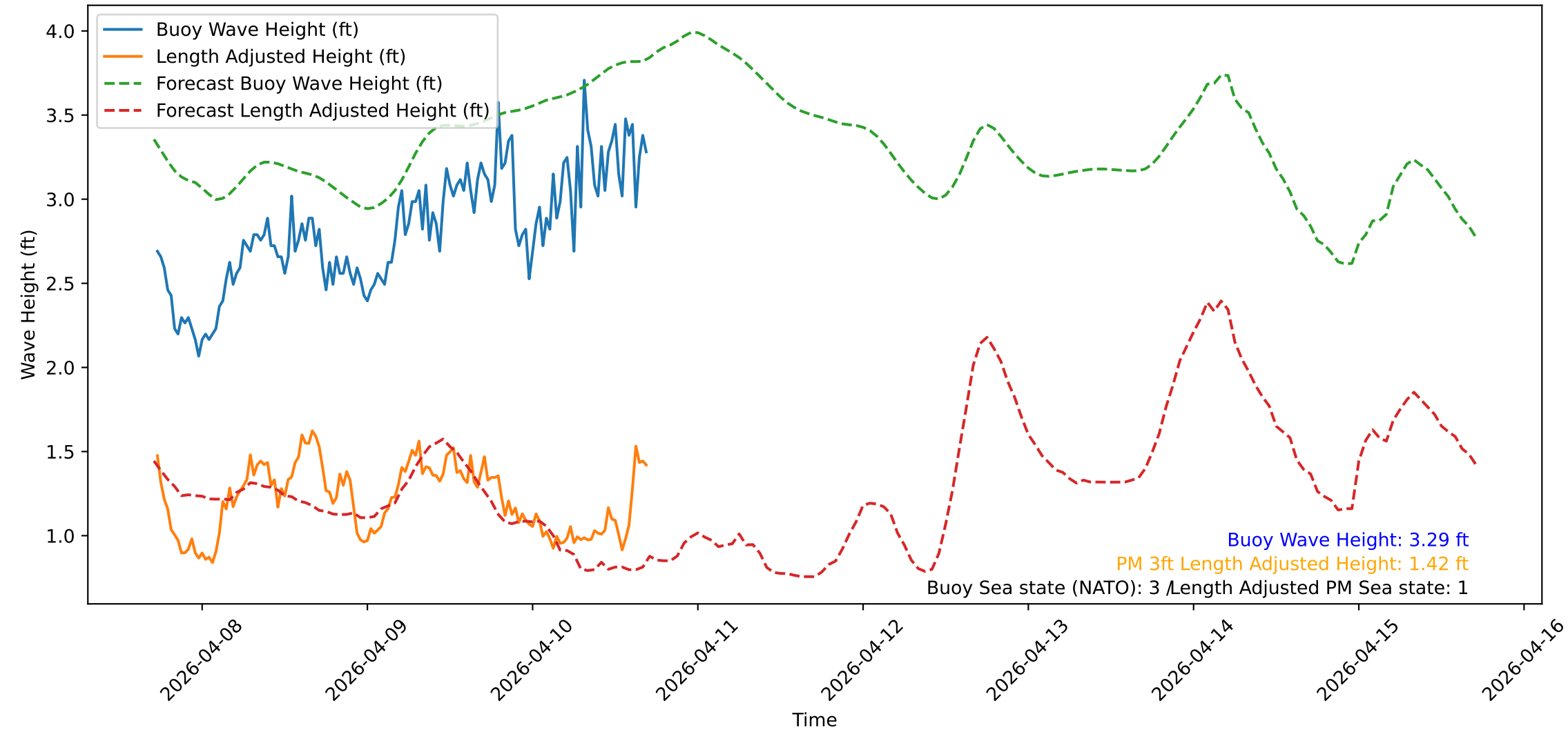
Wave Heights over Time for Red Beach at 2026-04-10 17:20:51
