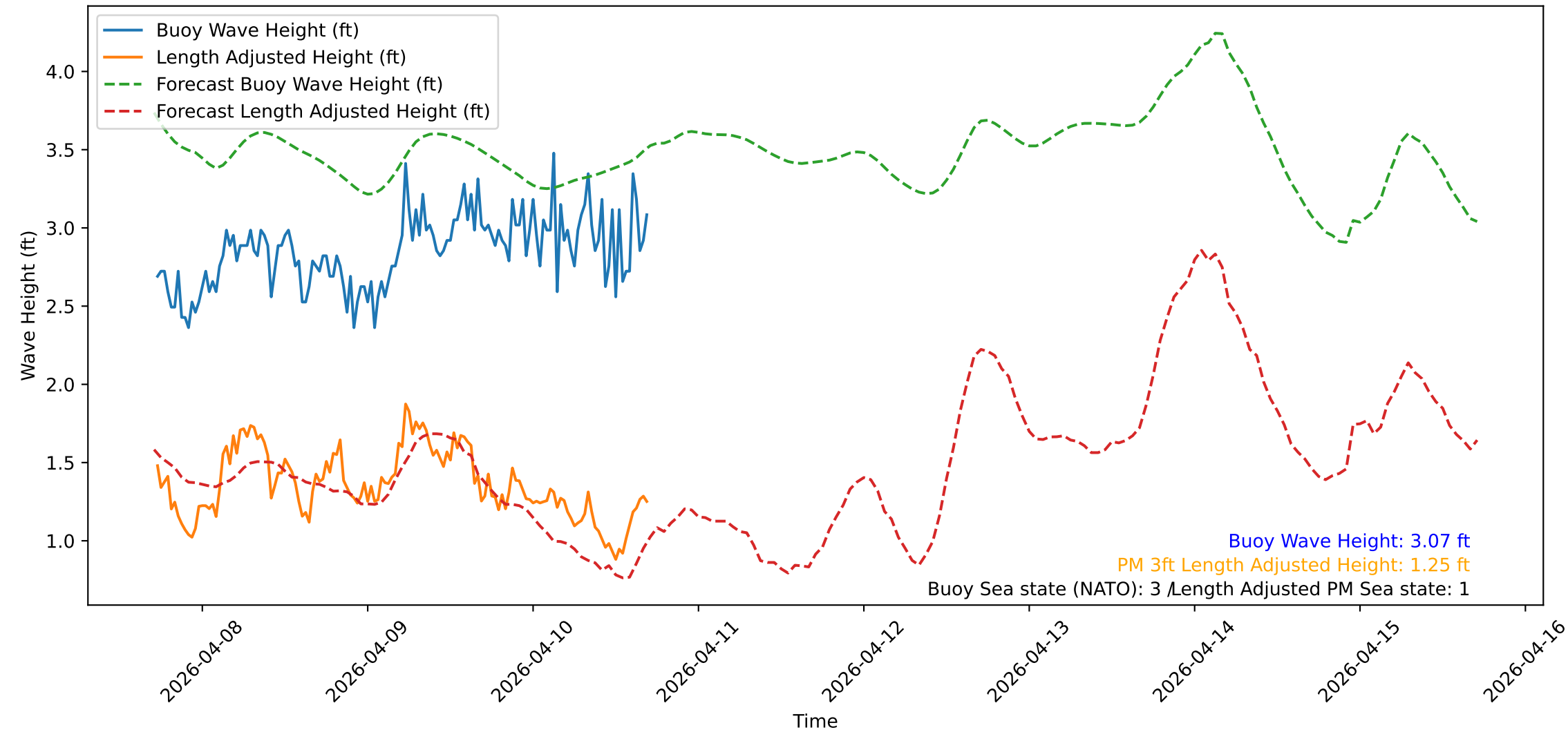
Wave Heights over Time for Green Beach at 2026-04-10 17:21:14
