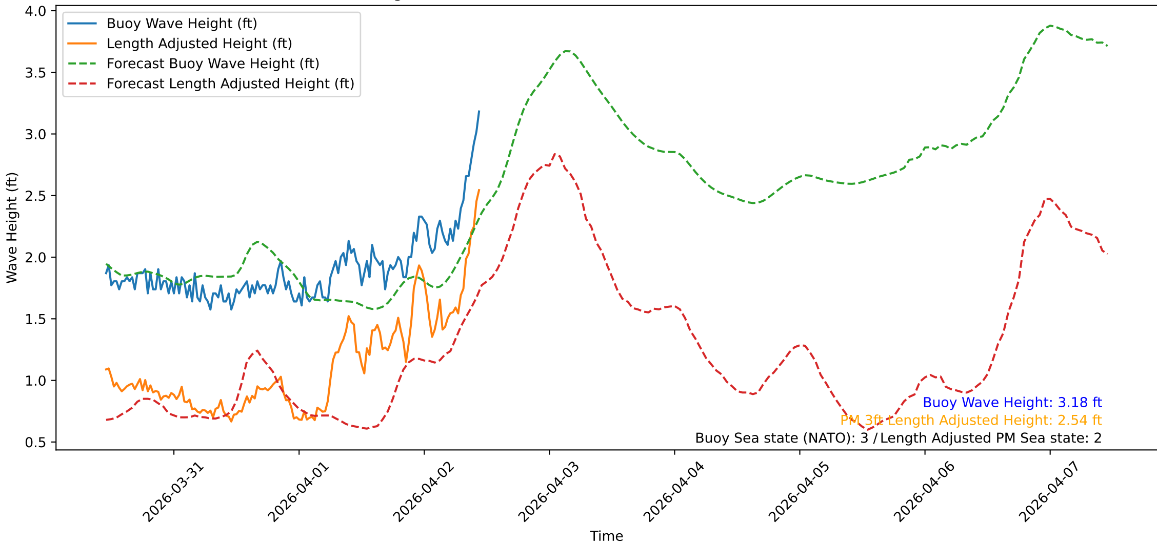
Wave Heights over Time for Oceanside Harbor at 2026-04-02 11:10:31
