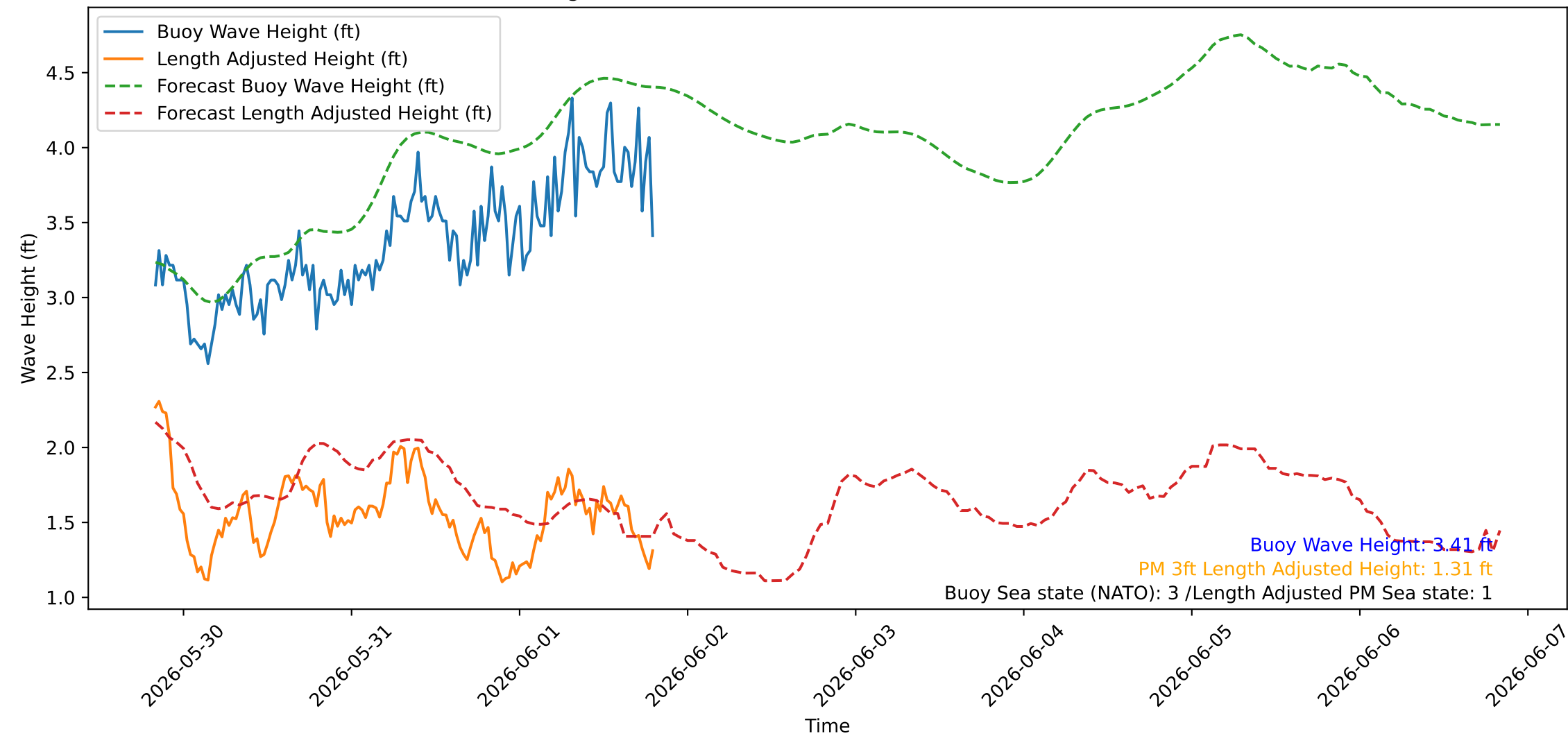
Wave Heights over Time for Green Beach at 2026-06-01 19:51:09
