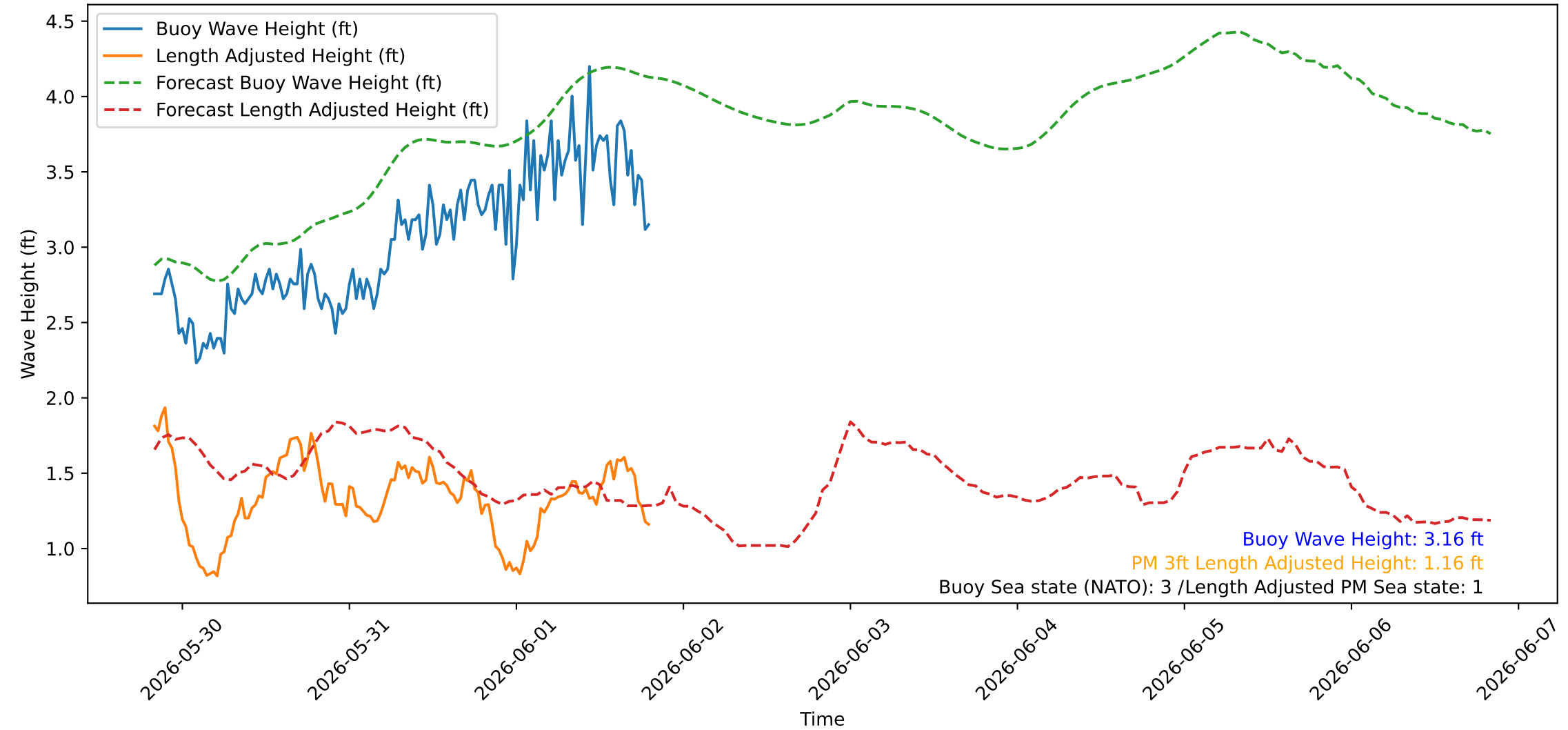
Wave Heights over Time for Red Beach at 2026-06-01 19:50:47
