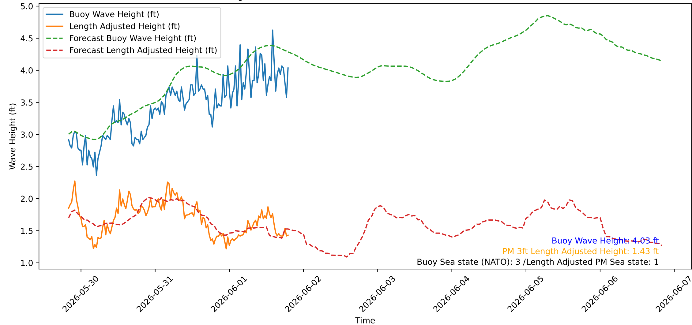
Wave Heights over Time for Oceanside Harbor at 2026-06-01 19:50:26
