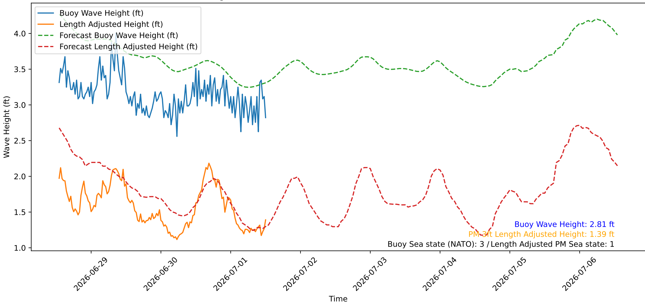
Wave Heights over Time for Oceanside Harbor at 2026-07-01 13:00:26
