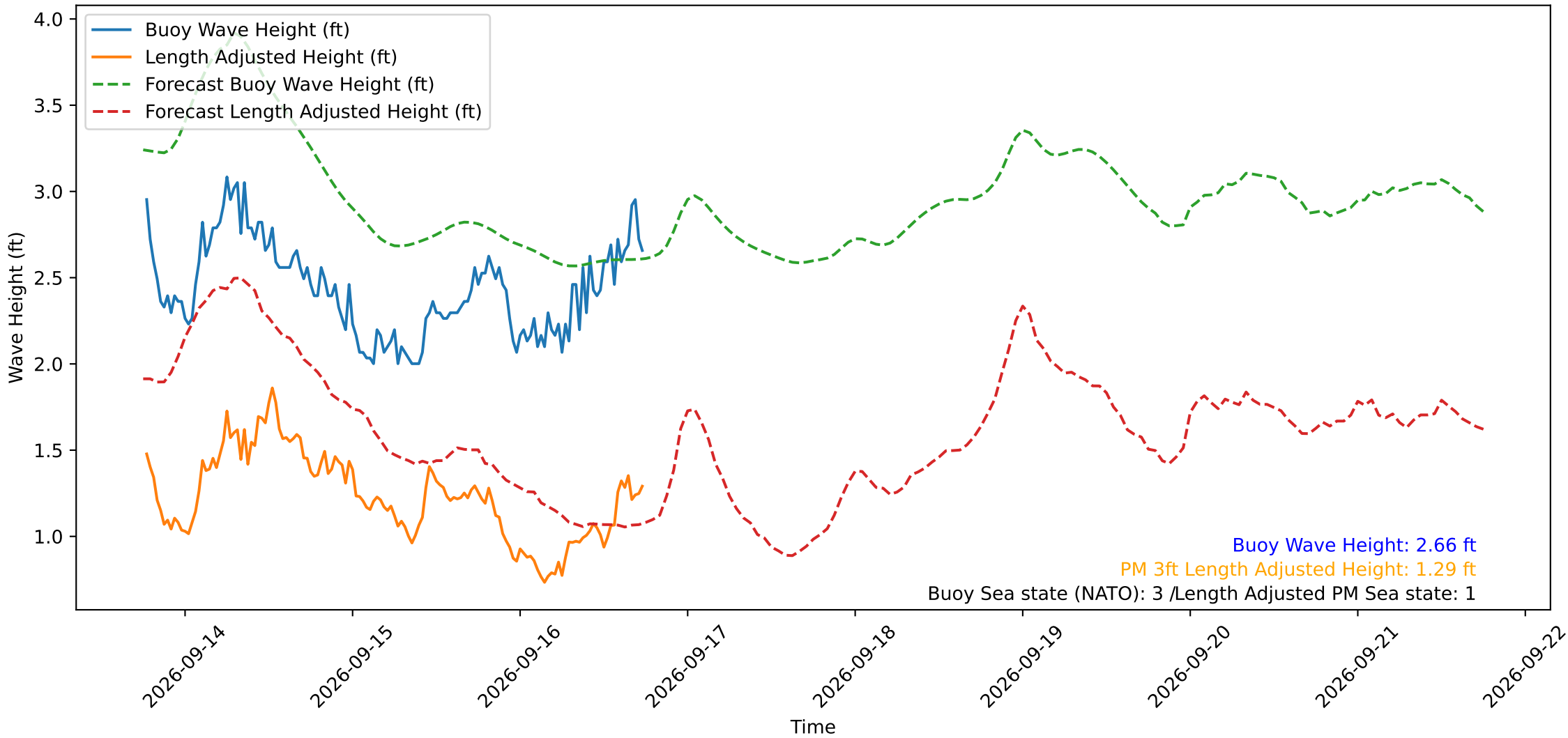
Wave Heights over Time for Red Beach at 2026-09-16 18:20:50
