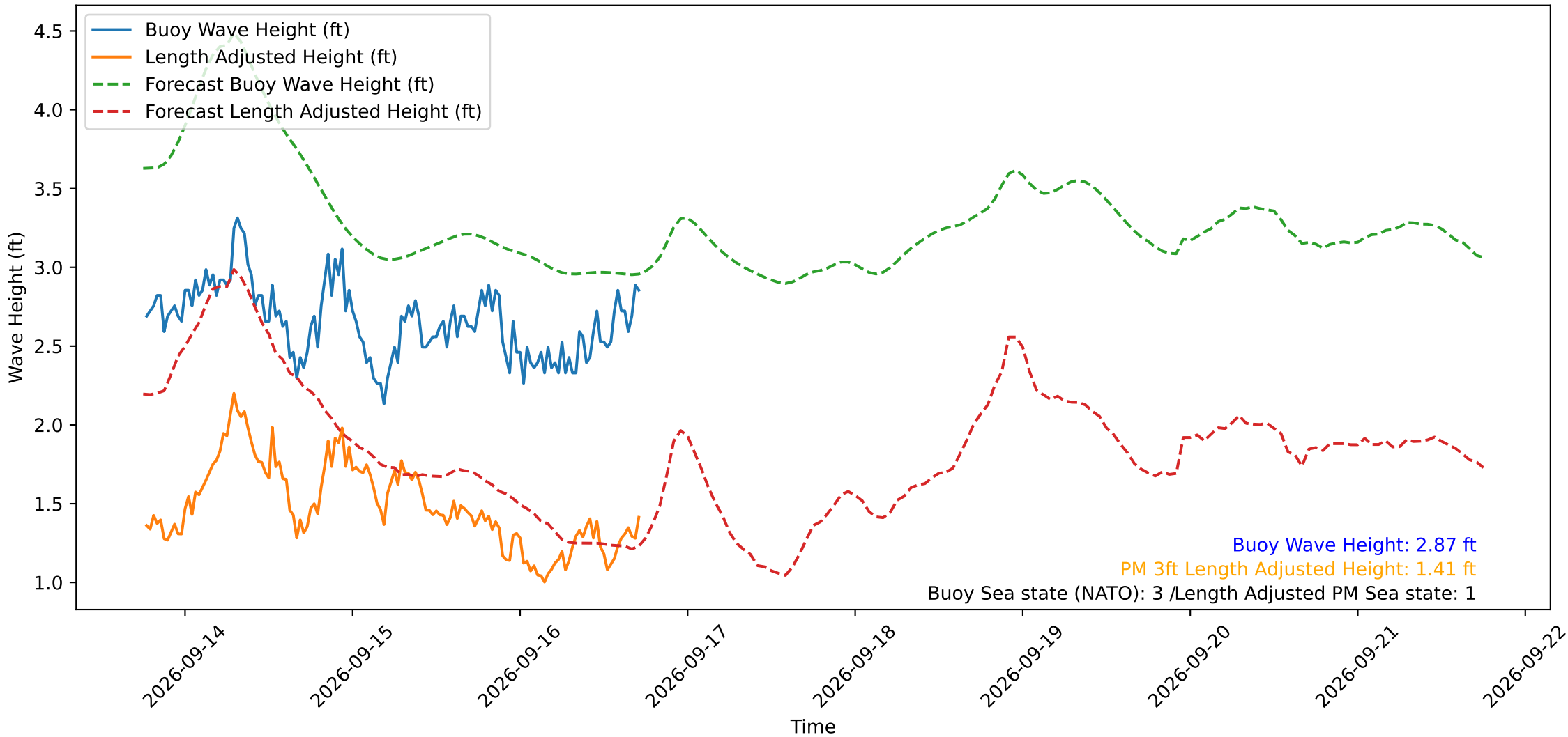
Wave Heights over Time for Green Beach at 2026-09-16 18:21:14
