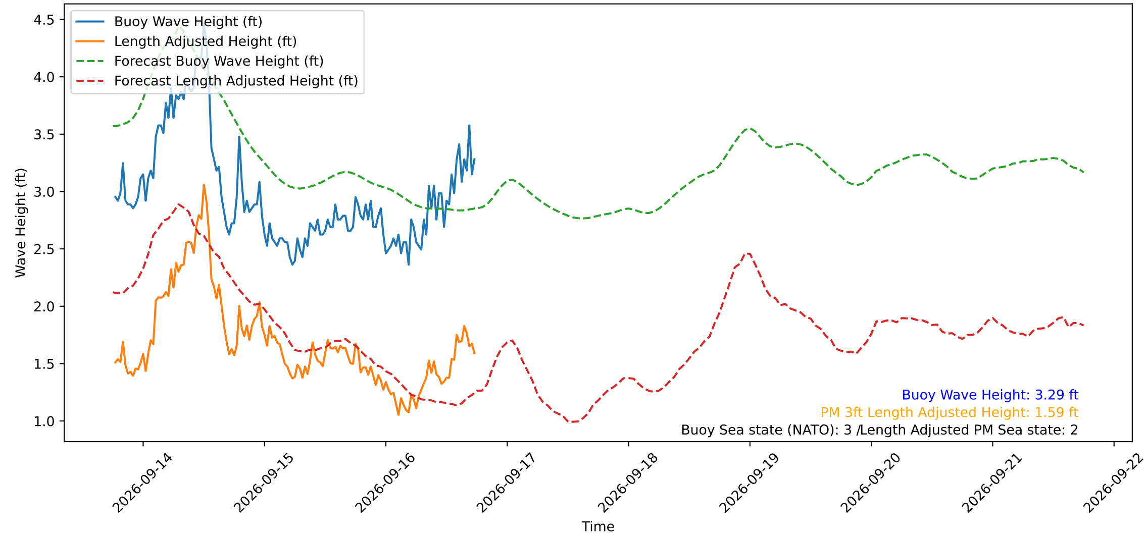
Wave Heights over Time for Oceanside Harbor at 2026-09-16 18:20:29
