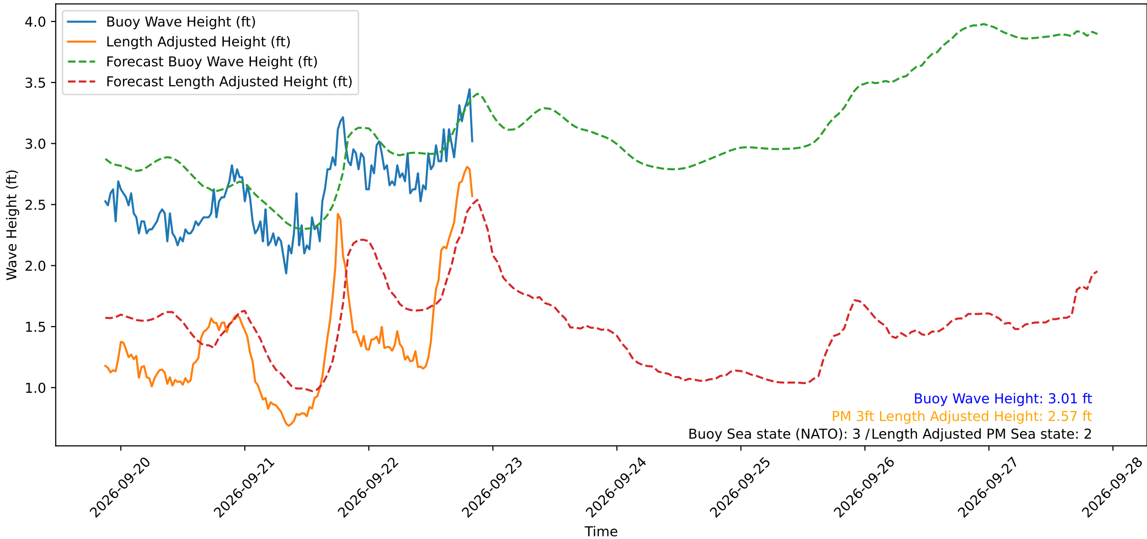
Wave Heights over Time for Green Beach at 2026-09-22 20:41:11
