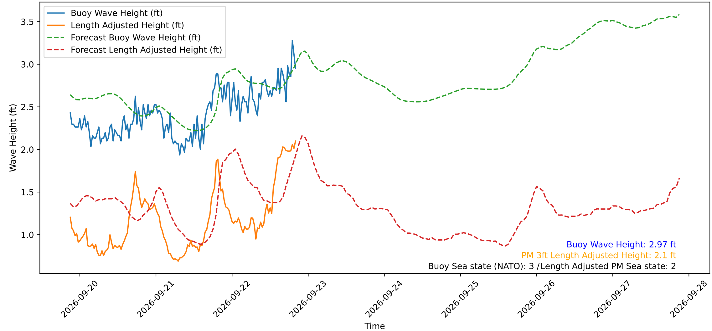
Wave Heights over Time for Red Beach at 2026-09-22 20:40:49
