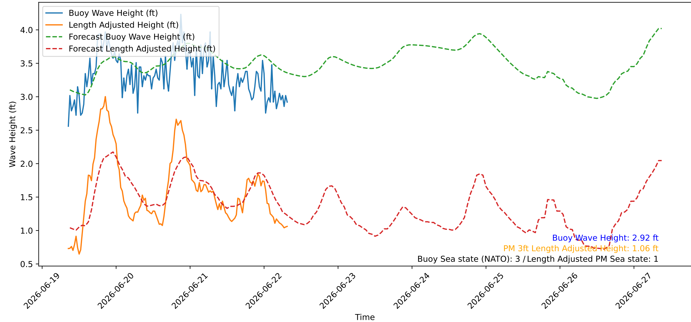
Wave Heights over Time for Green Beach at 2026-06-22 08:31:07
