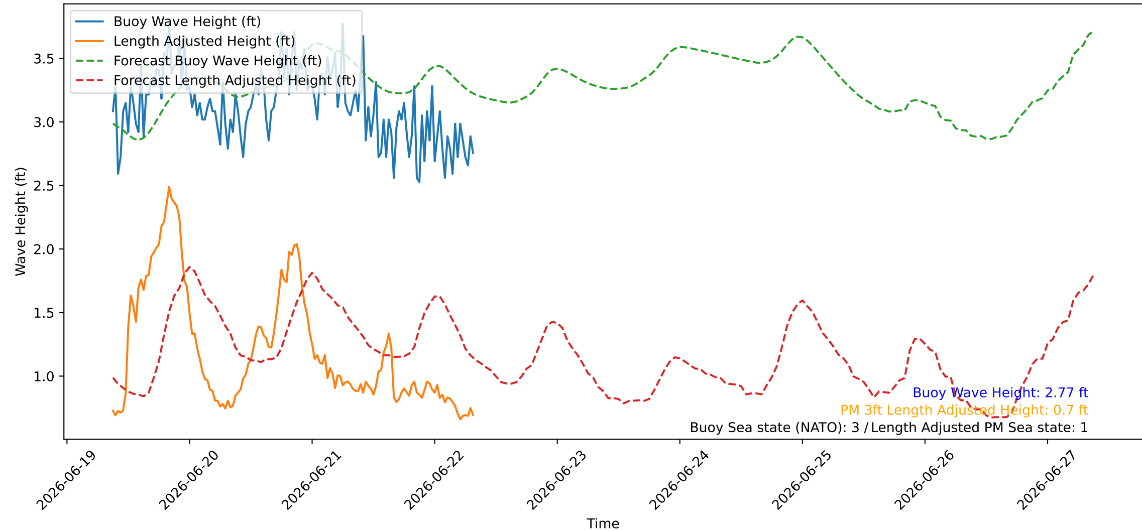
Wave Heights over Time for Red Beach at 2026-06-22 08:30:45
