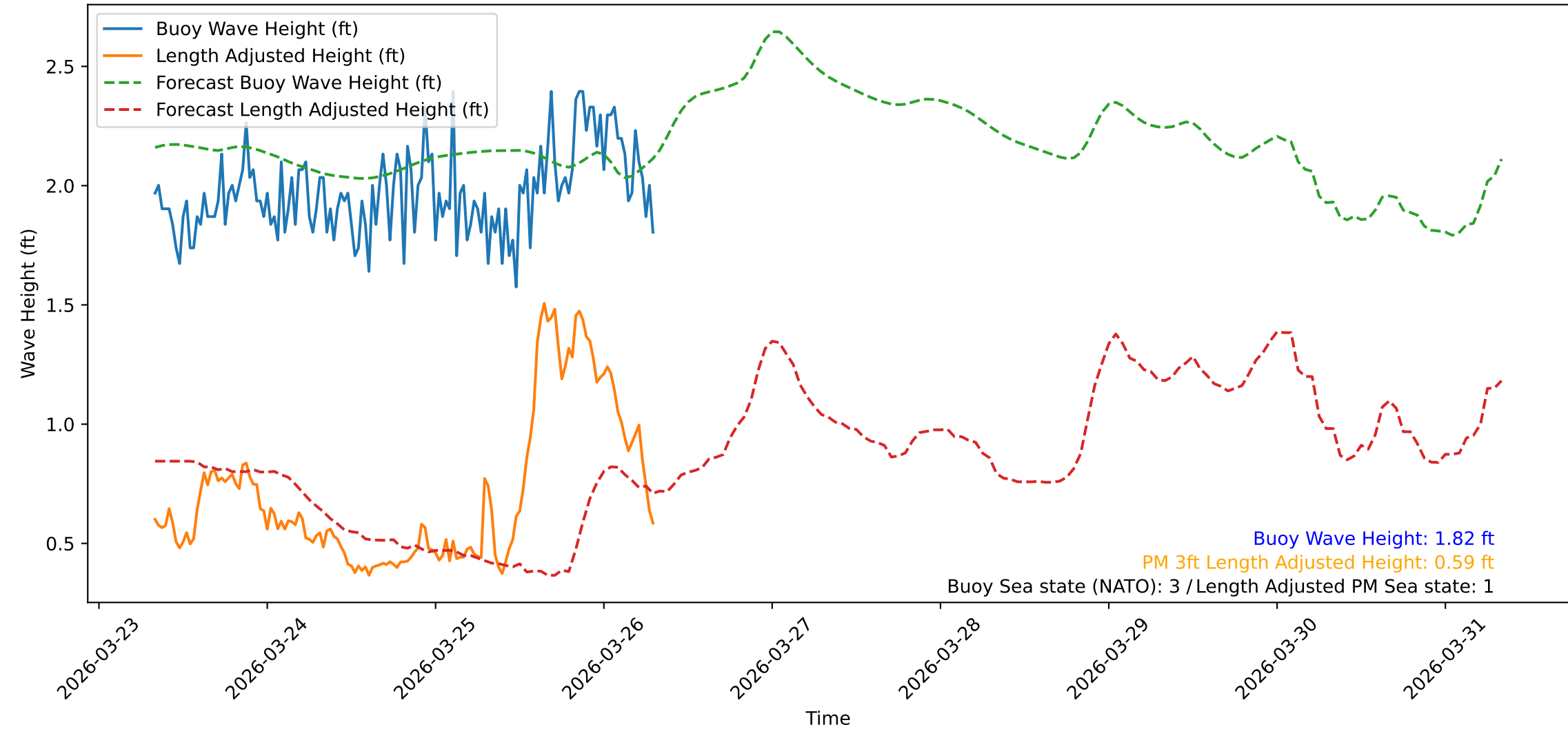
Wave Heights over Time for Red Beach at 2026-03-26 07:50:47
