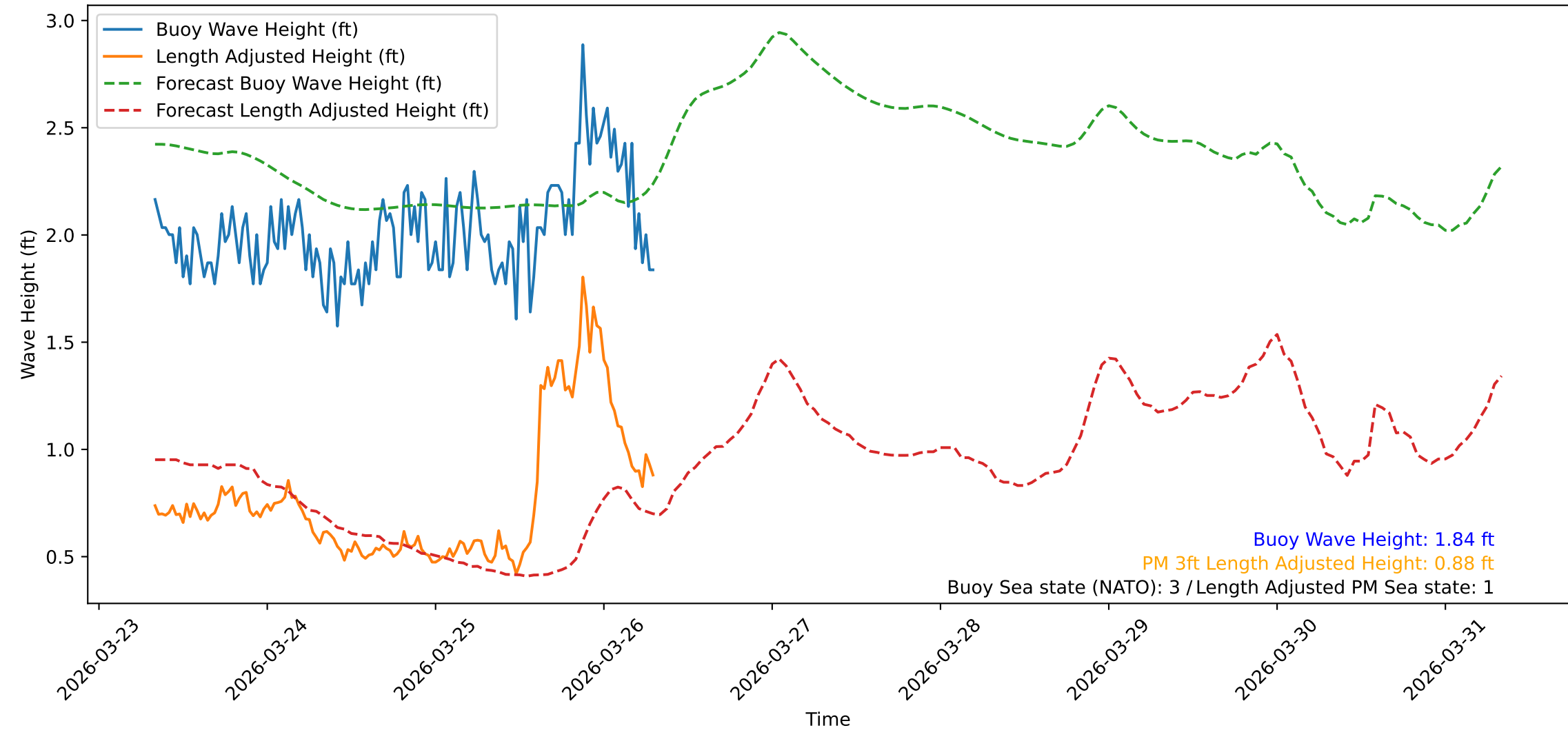
Wave Heights over Time for Oceanside Harbor at 2026-03-26 07:50:31
