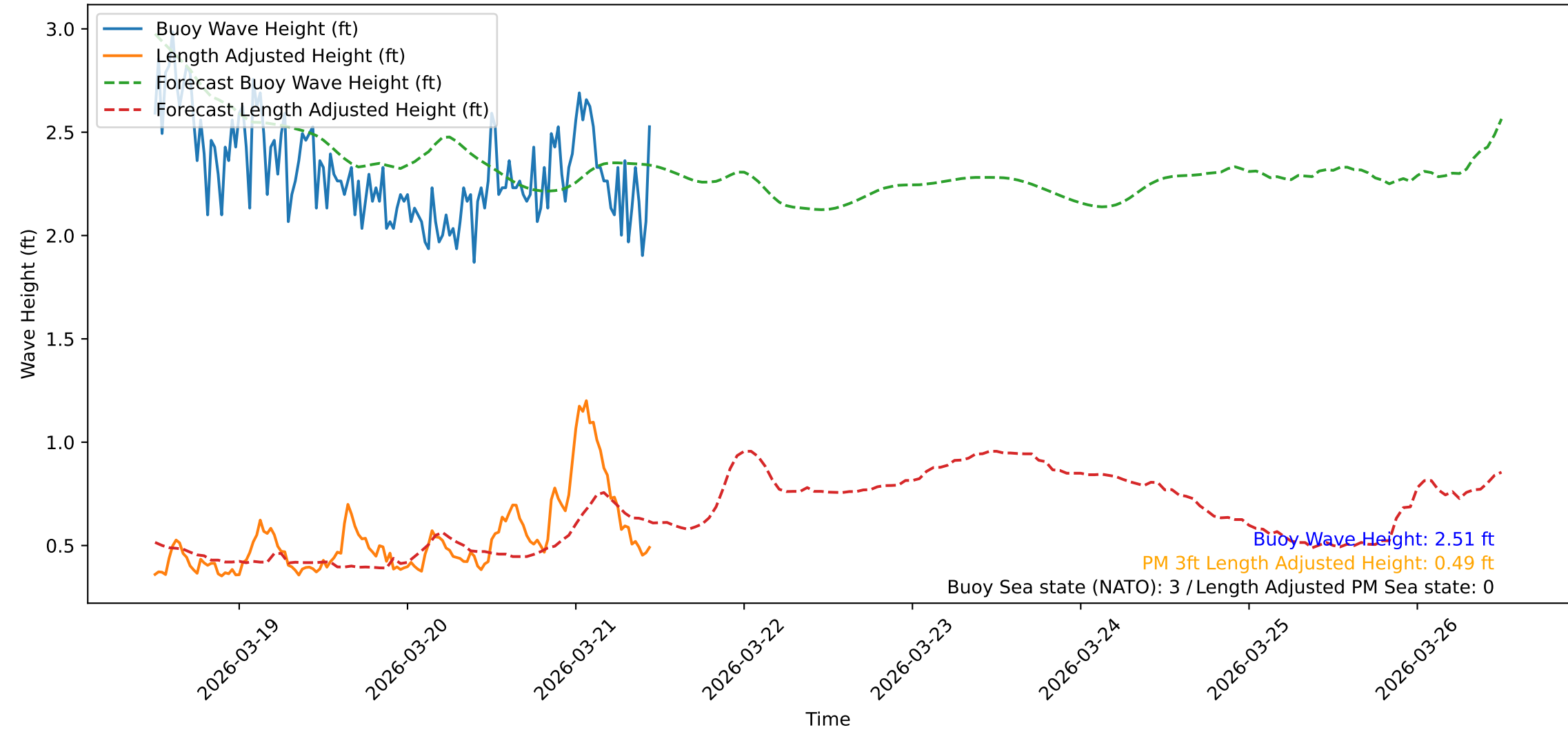
Wave Heights over Time for Red Beach at 2026-03-21 11:50:48
