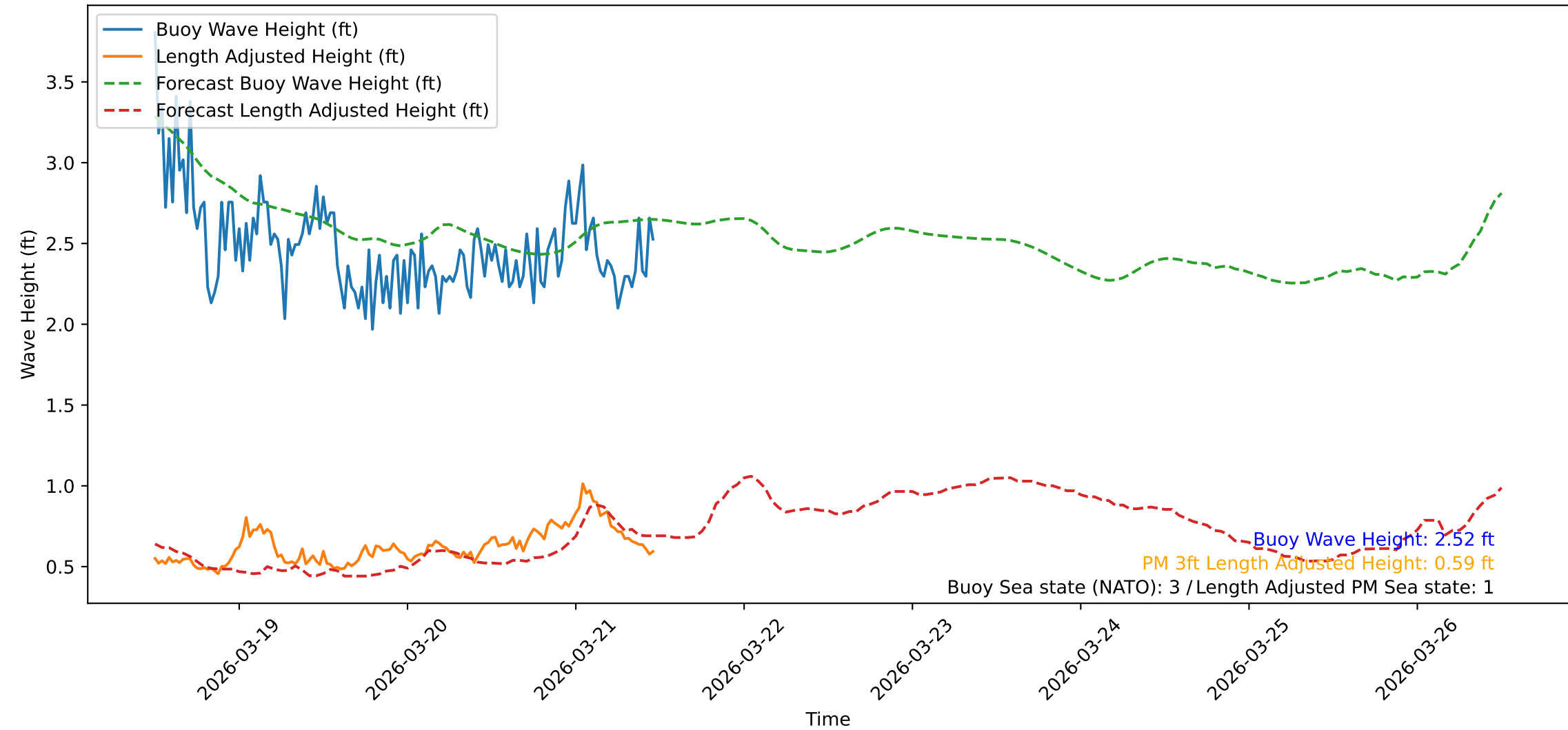
Wave Heights over Time for Oceanside Harbor at 2026-03-21 11:50:32
