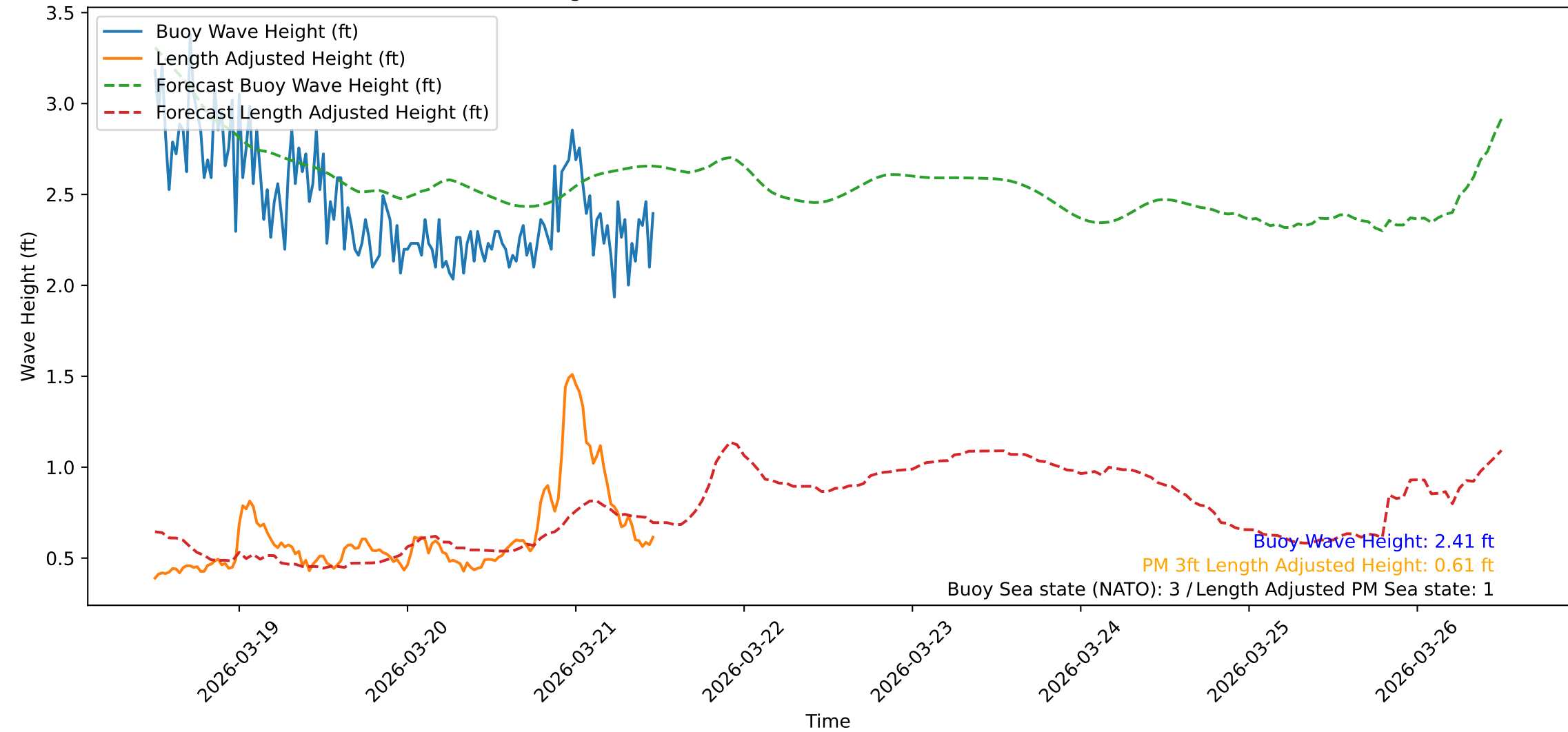
Wave Heights over Time for Green Beach at 2026-03-21 11:51:11
