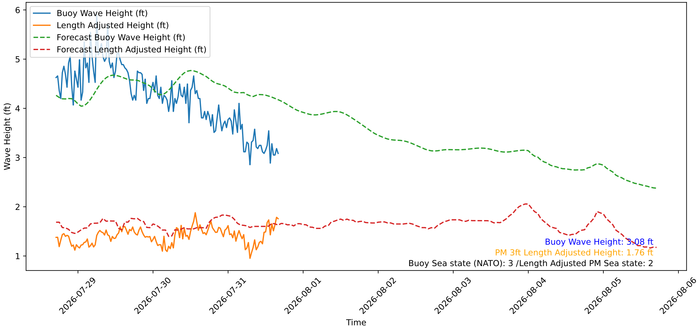
Wave Heights over Time for Oceanside Harbor at 2026-07-31 17:00:27
