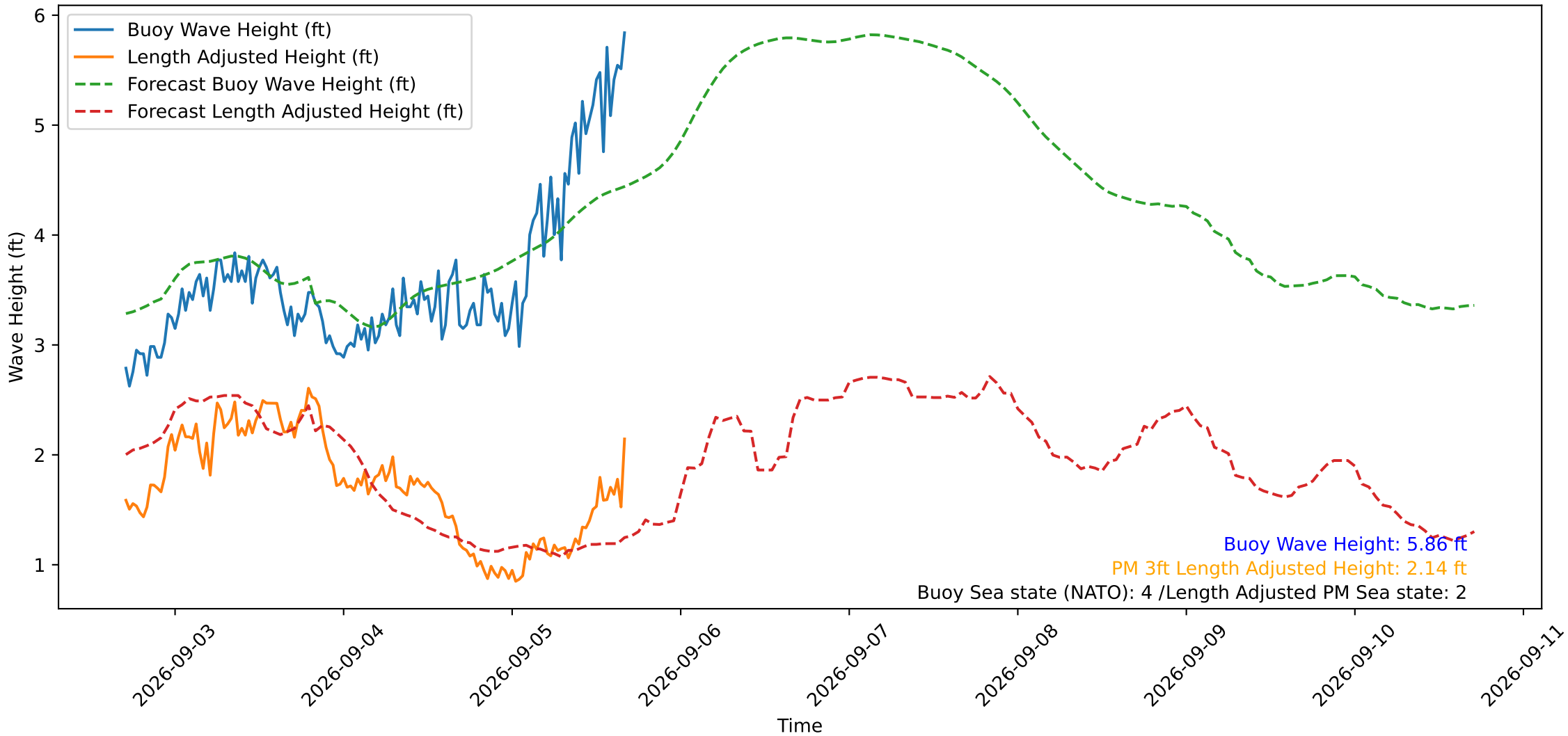
Wave Heights over Time for Oceanside Harbor at 2026-09-05 17:00:30
