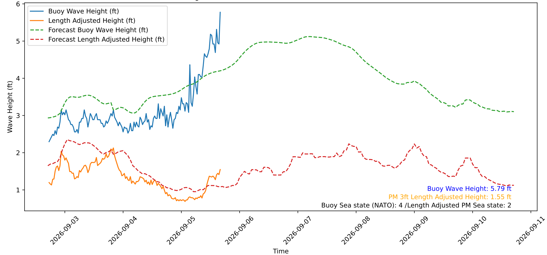
Wave Heights over Time for Red Beach at 2026-09-05 17:00:50
