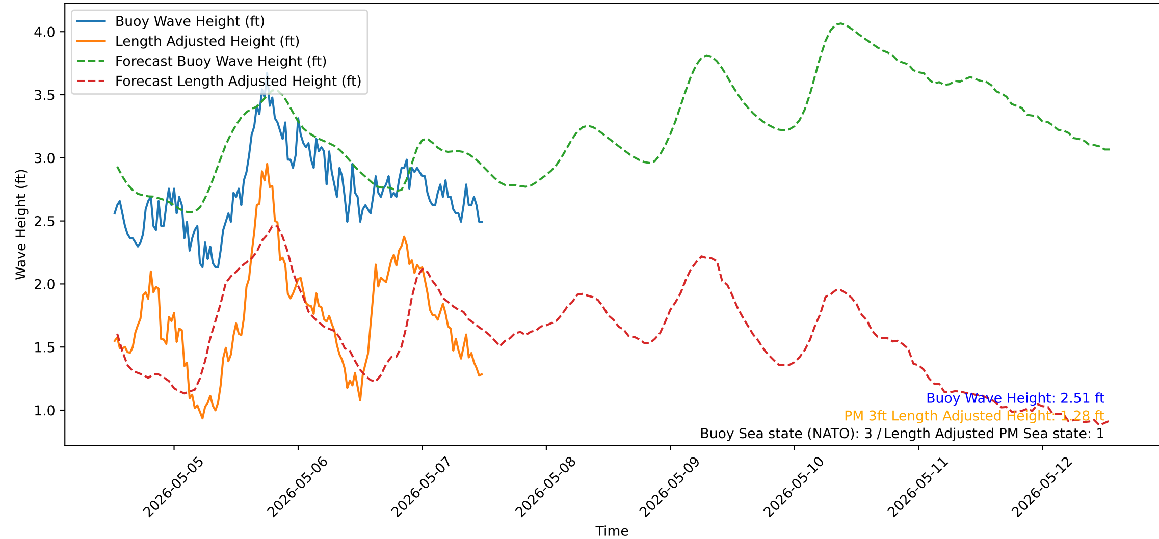
Wave Heights over Time for Green Beach at 2026-05-07 12:31:12
