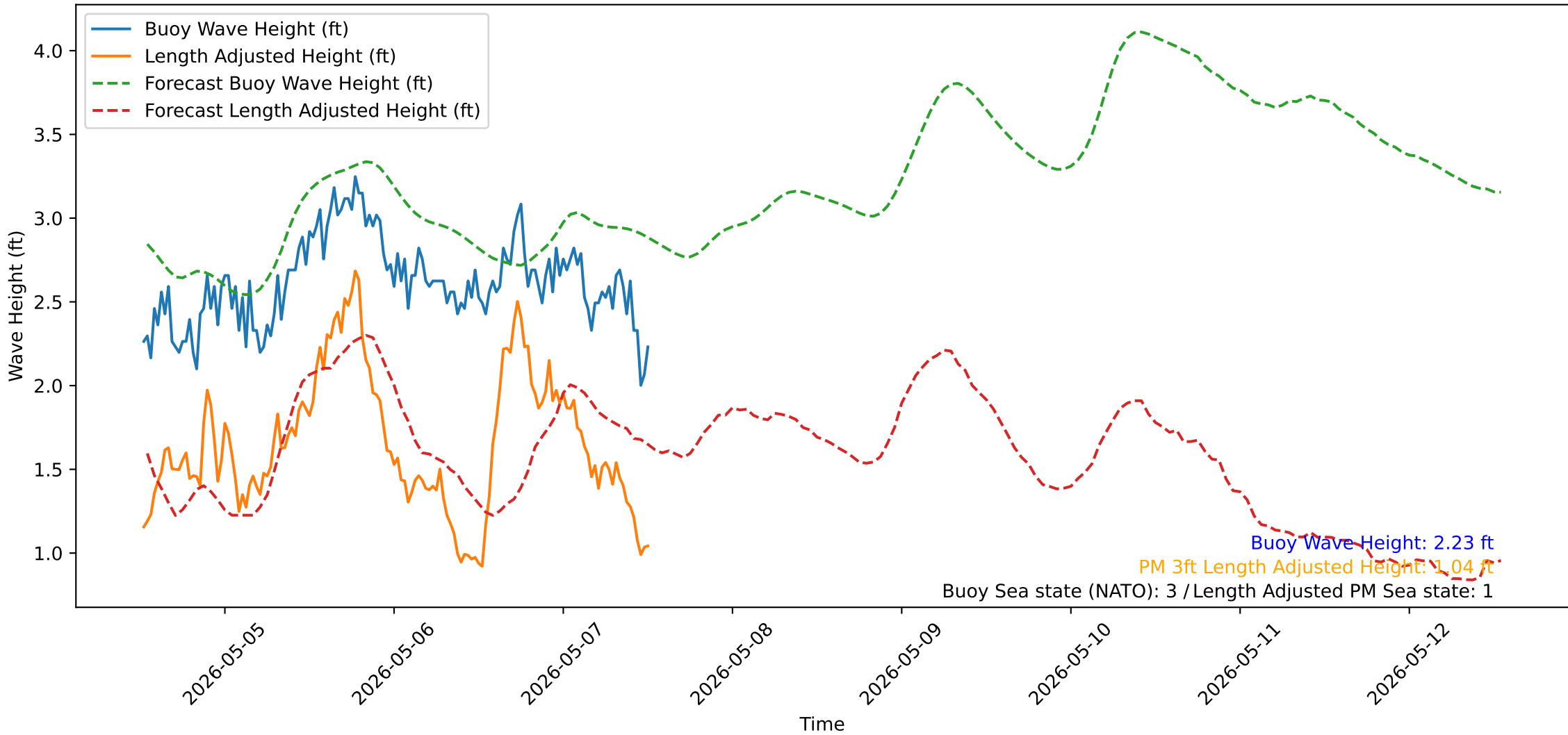
Wave Heights over Time for Oceanside Harbor at 2026-05-07 12:30:32
