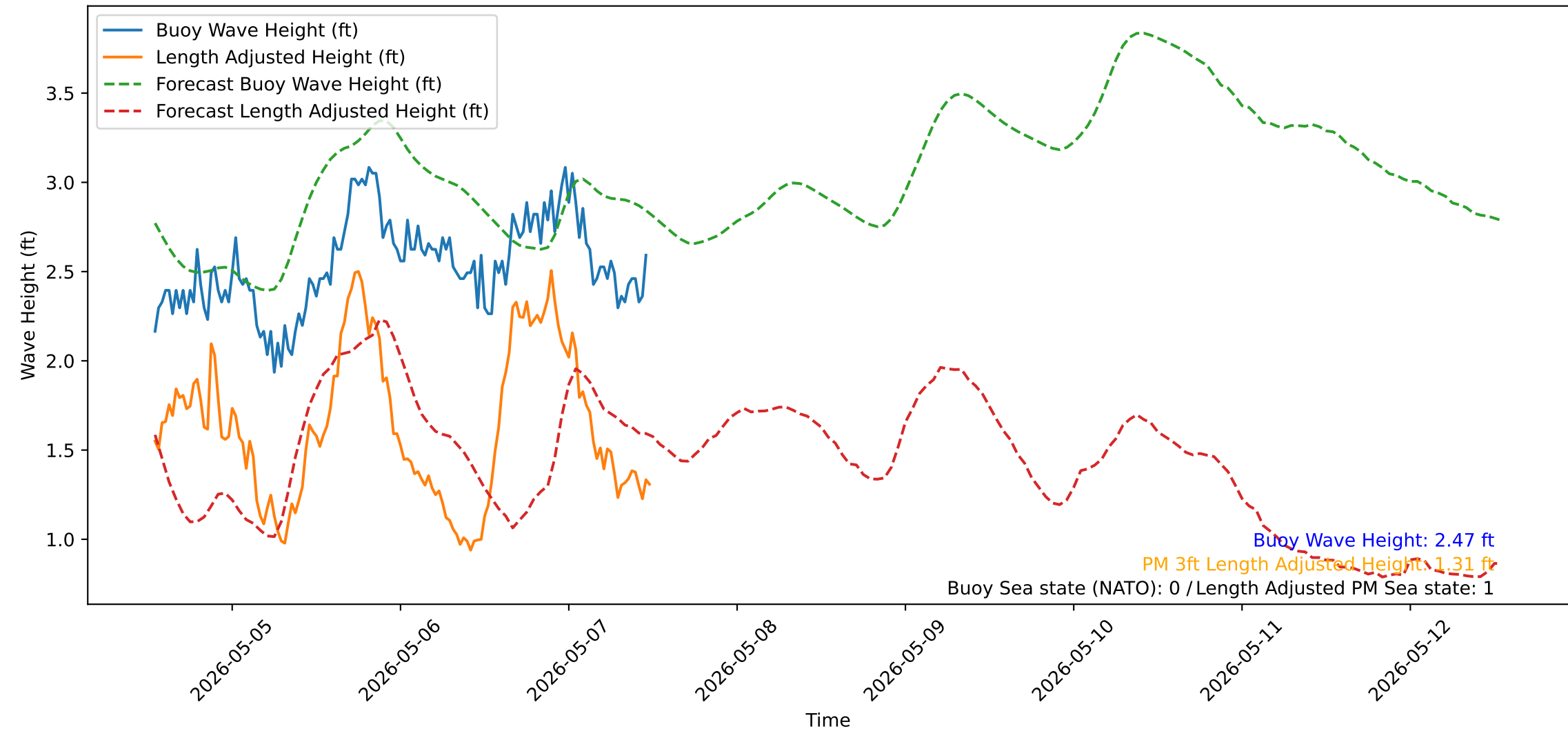
Wave Heights over Time for Red Beach at 2026-05-07 12:30:51
