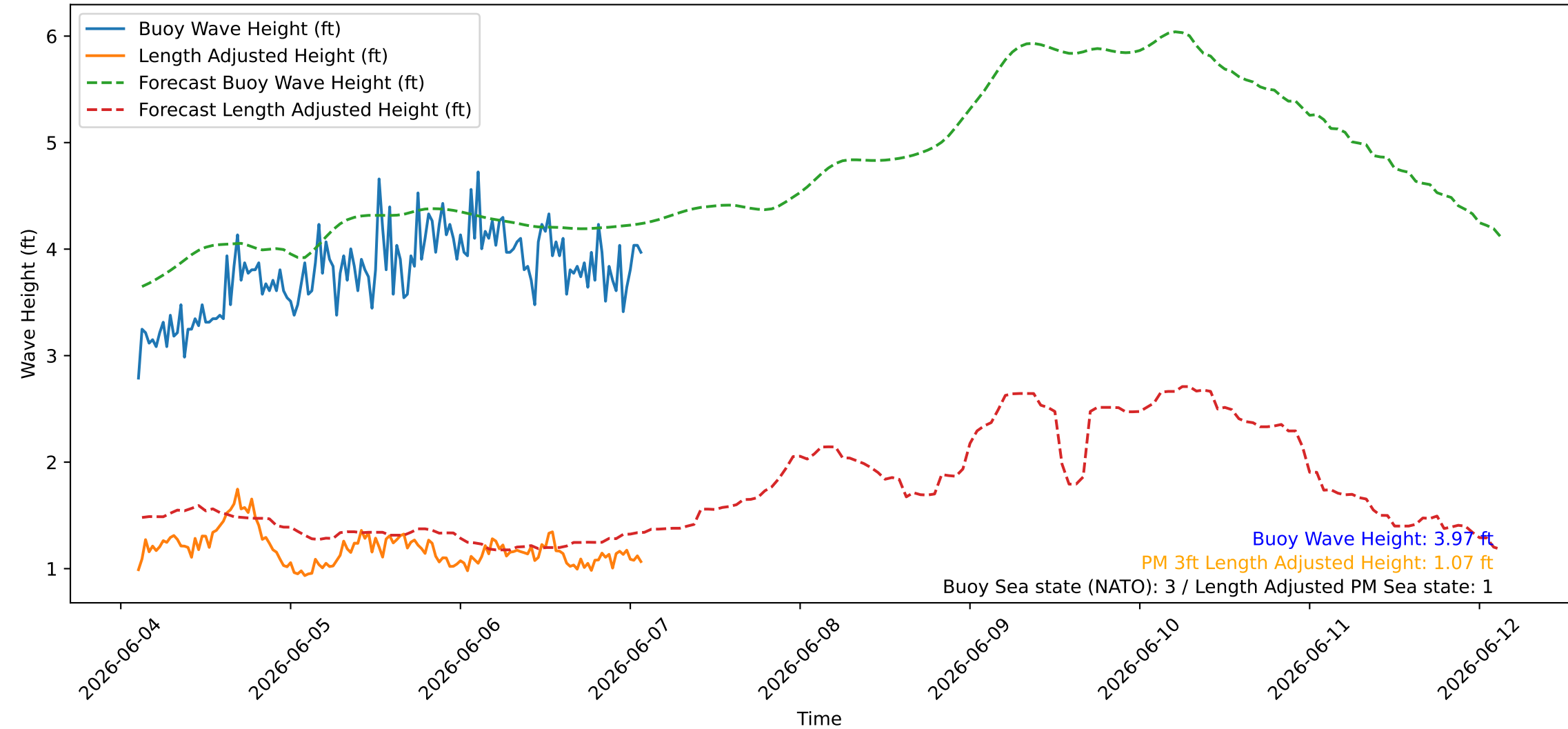
Wave Heights over Time for Green Beach at 2026-06-07 02:31:08
