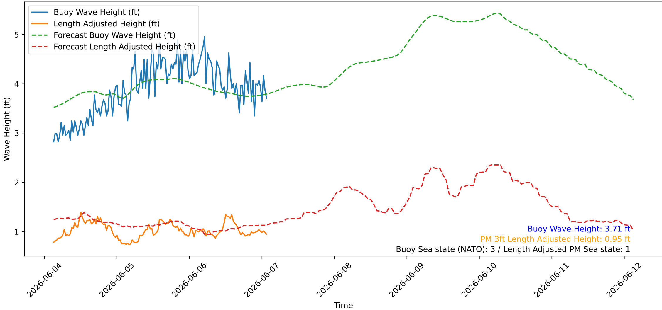
Wave Heights over Time for Red Beach at 2026-06-07 02:30:46
