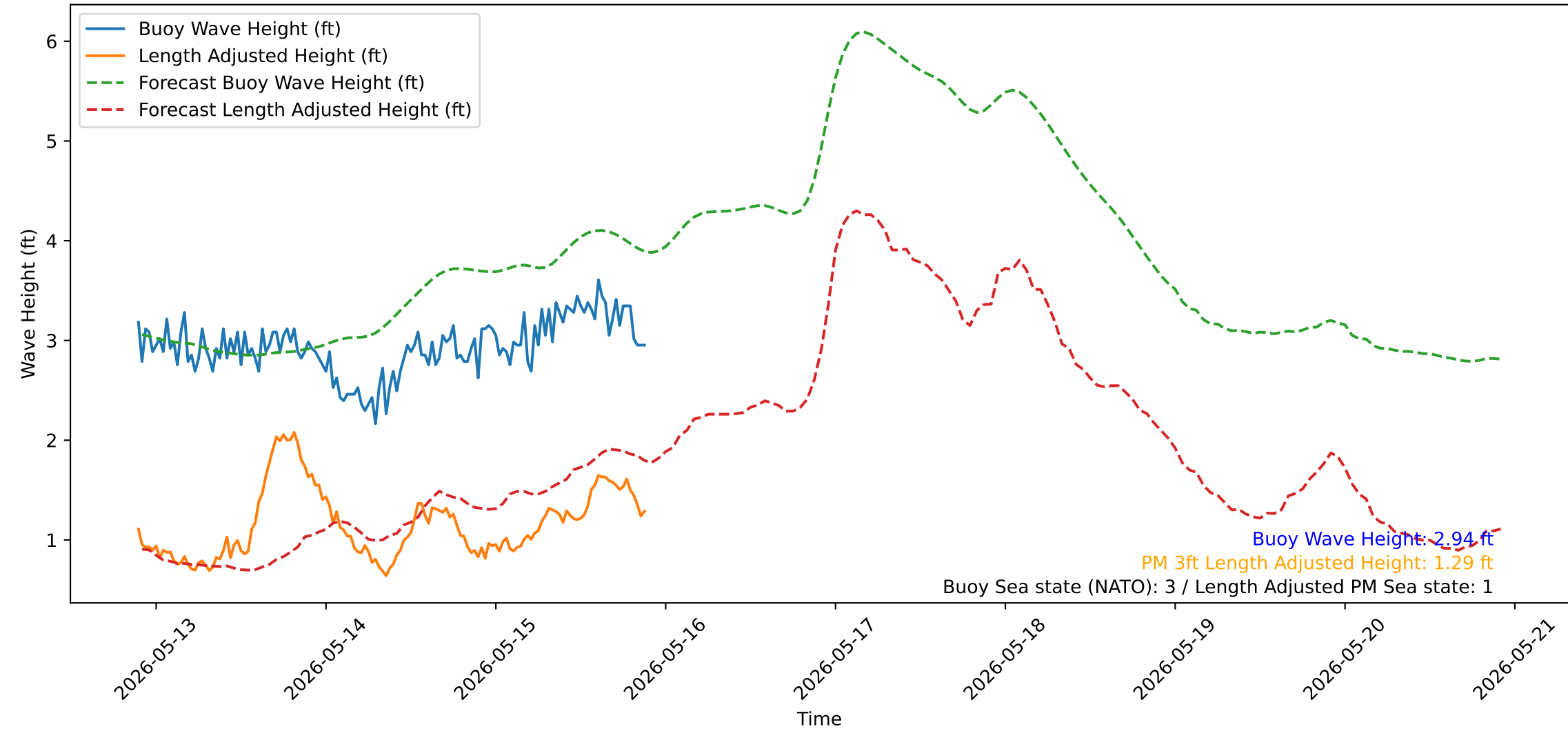
Wave Heights over Time for Oceanside Harbor at 2026-05-15 21:30:32
