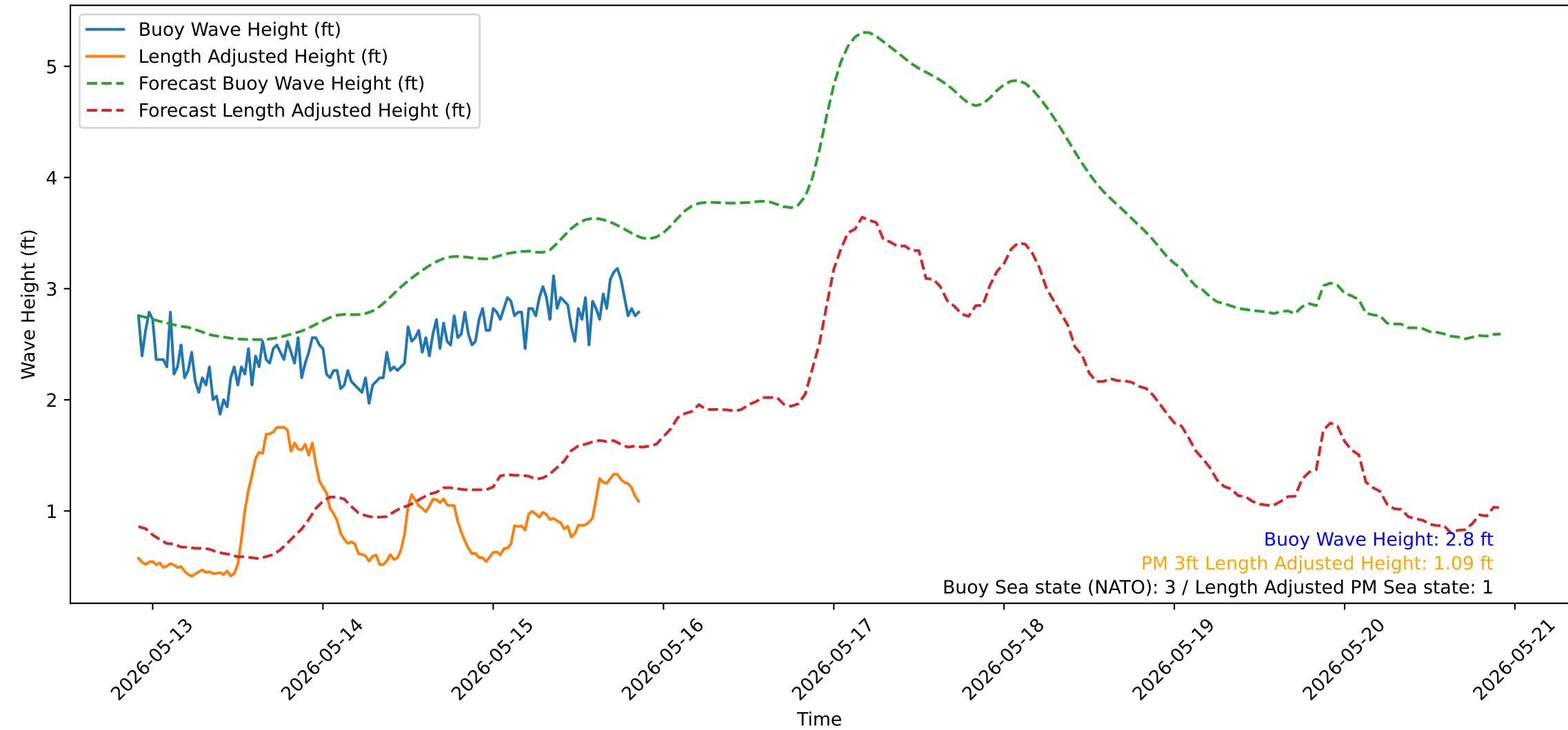
Wave Heights over Time for Red Beach at 2026-05-15 21:30:51
