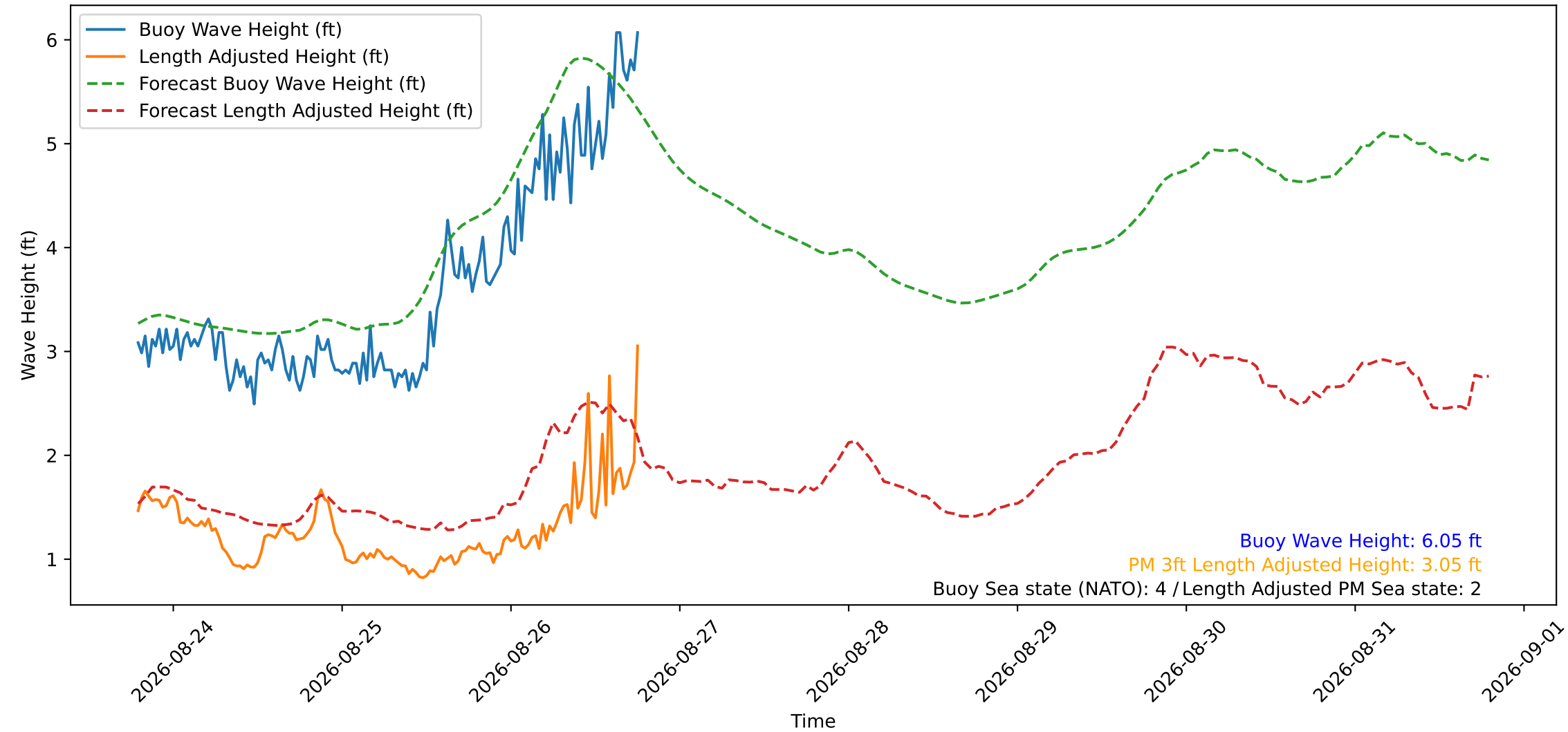
Wave Heights over Time for Green Beach at 2026-08-26 18:51:15
