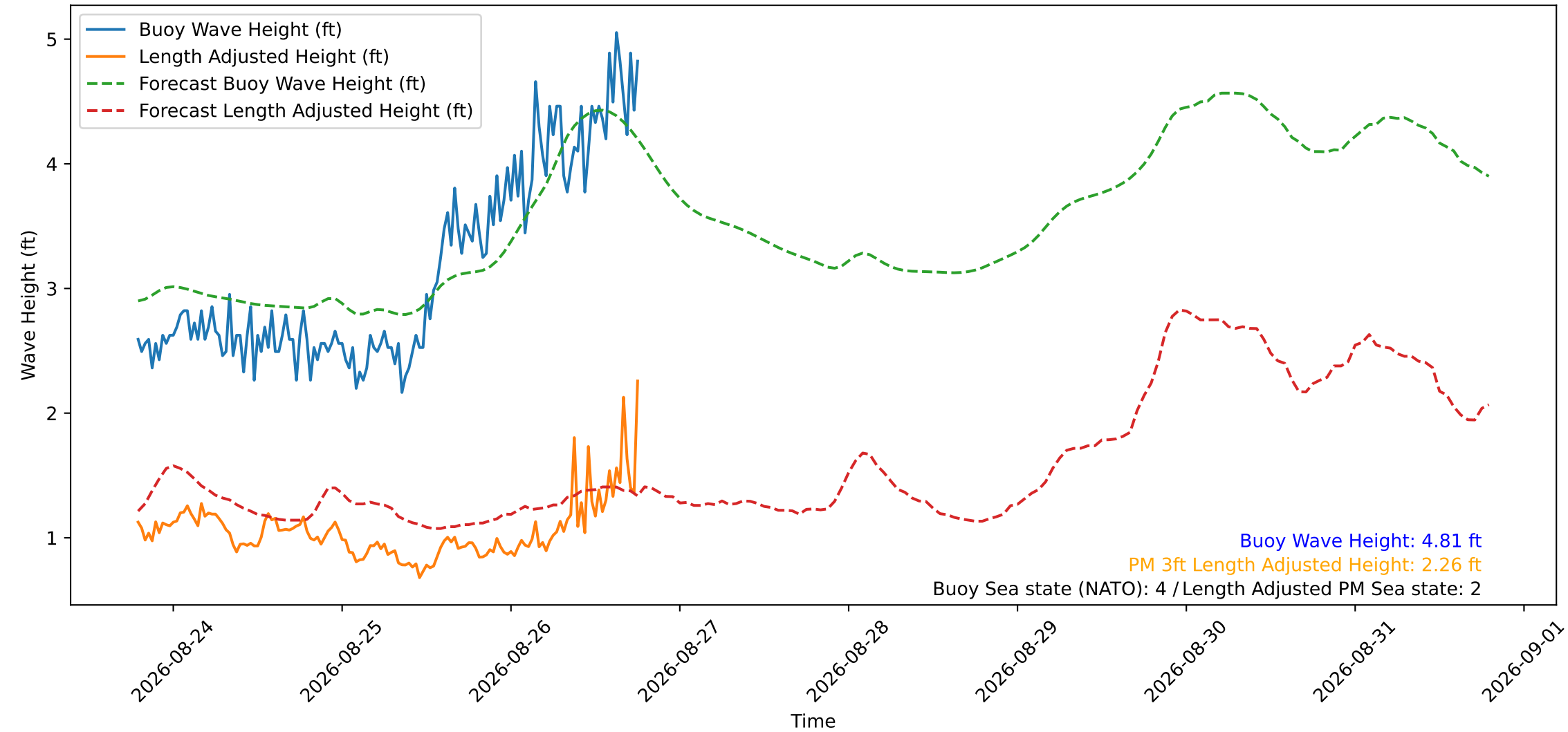
Wave Heights over Time for Red Beach at 2026-08-26 18:50:51
