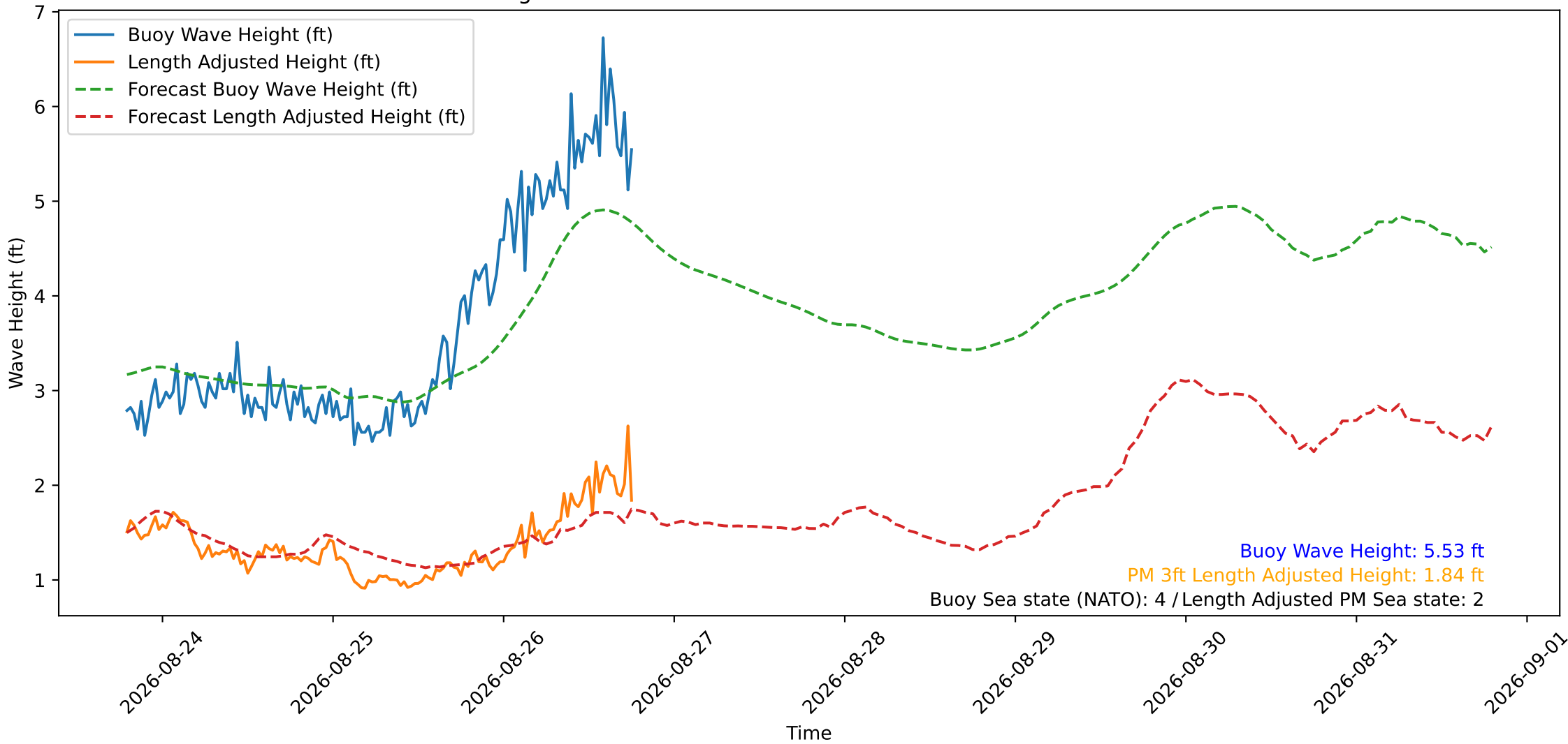
Wave Heights over Time for Oceanside Harbor at 2026-08-26 18:50:29
