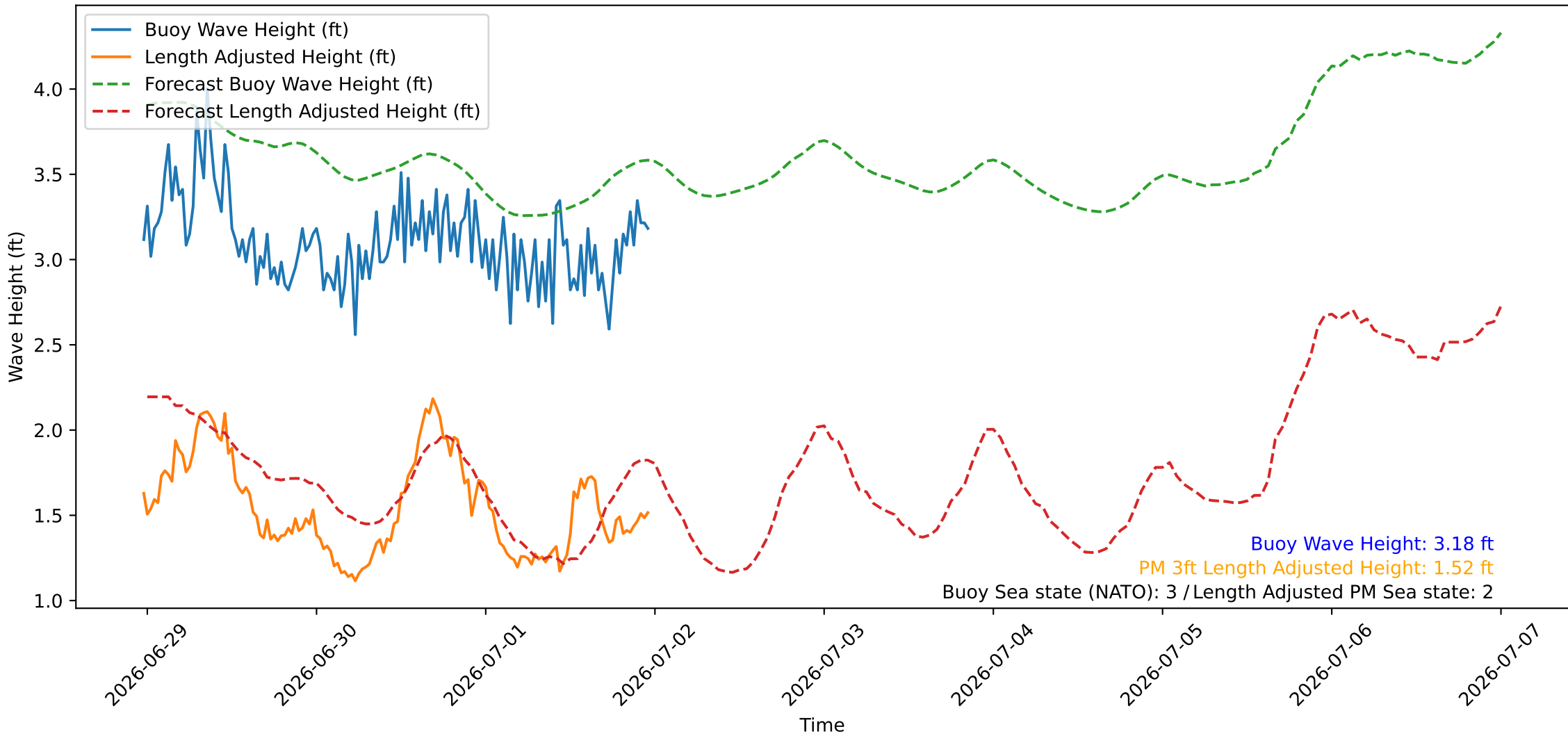
Wave Heights over Time for Oceanside Harbor at 2026-07-01 23:40:26
