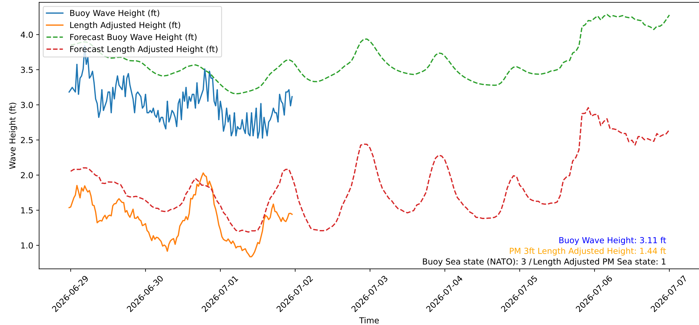
Wave Heights over Time for Green Beach at 2026-07-01 23:41:08
