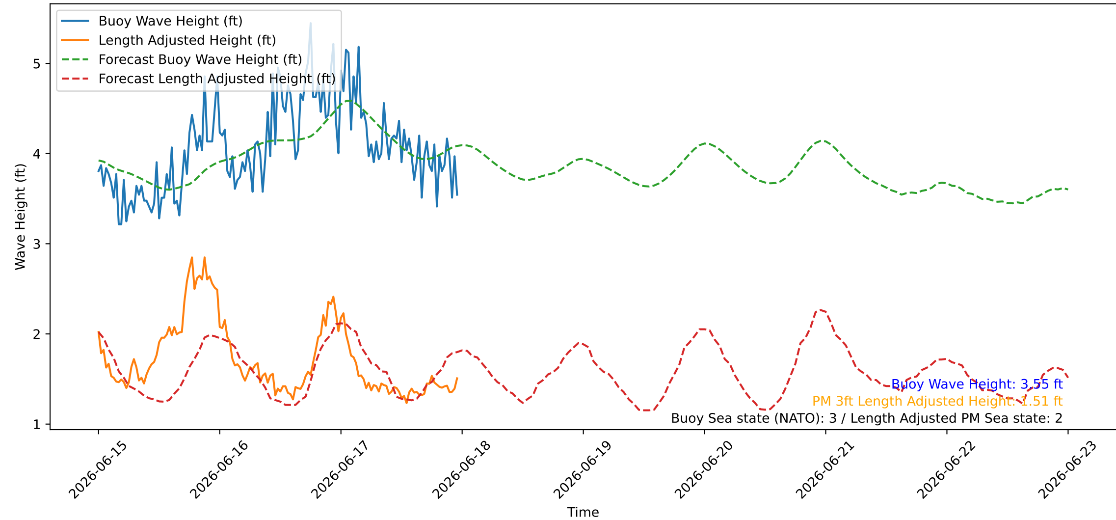
Wave Heights over Time for Oceanside Harbor at 2026-06-18 00:00:26
