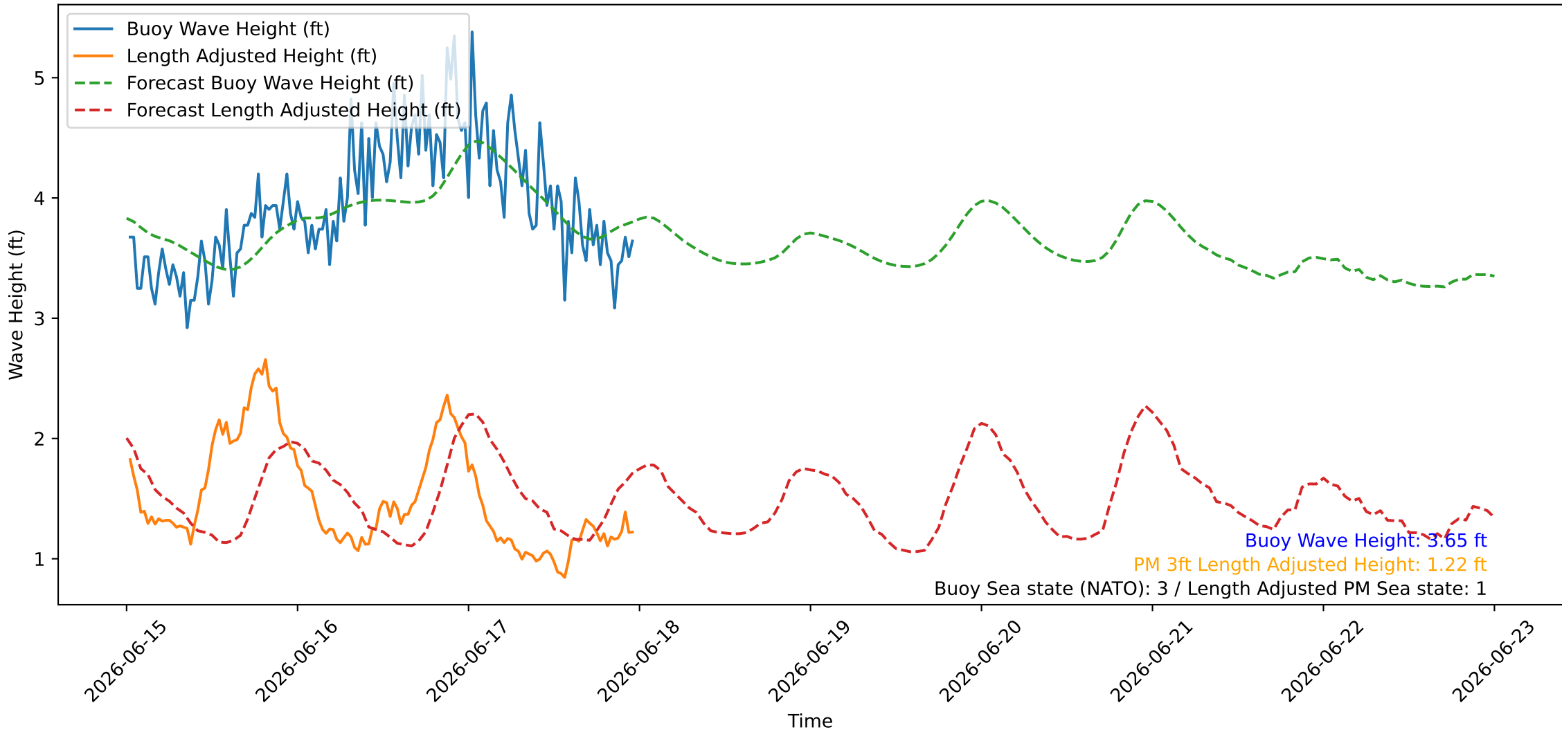
Wave Heights over Time for Red Beach at 2026-06-18 00:00:45
