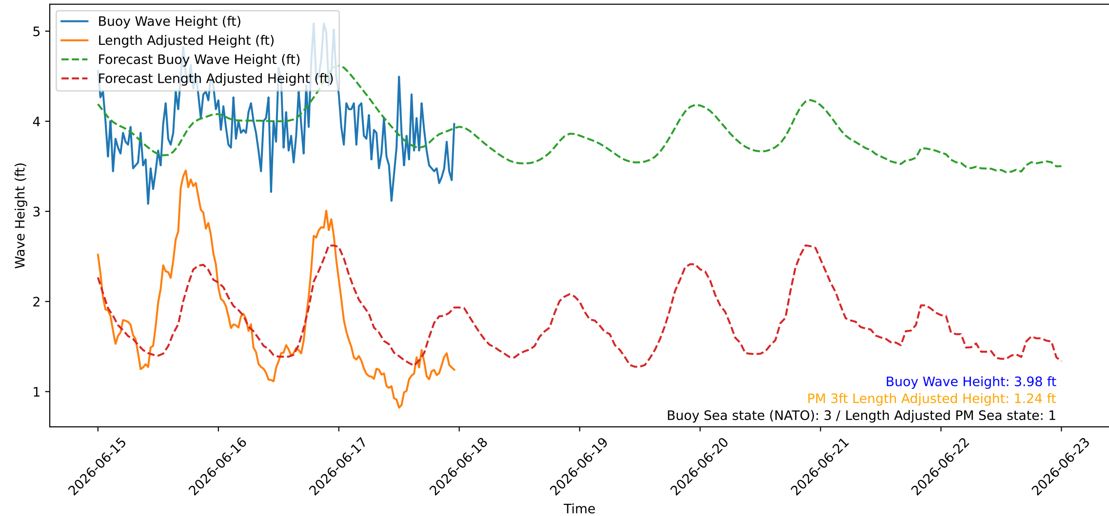
Wave Heights over Time for Green Beach at 2026-06-18 00:01:07
