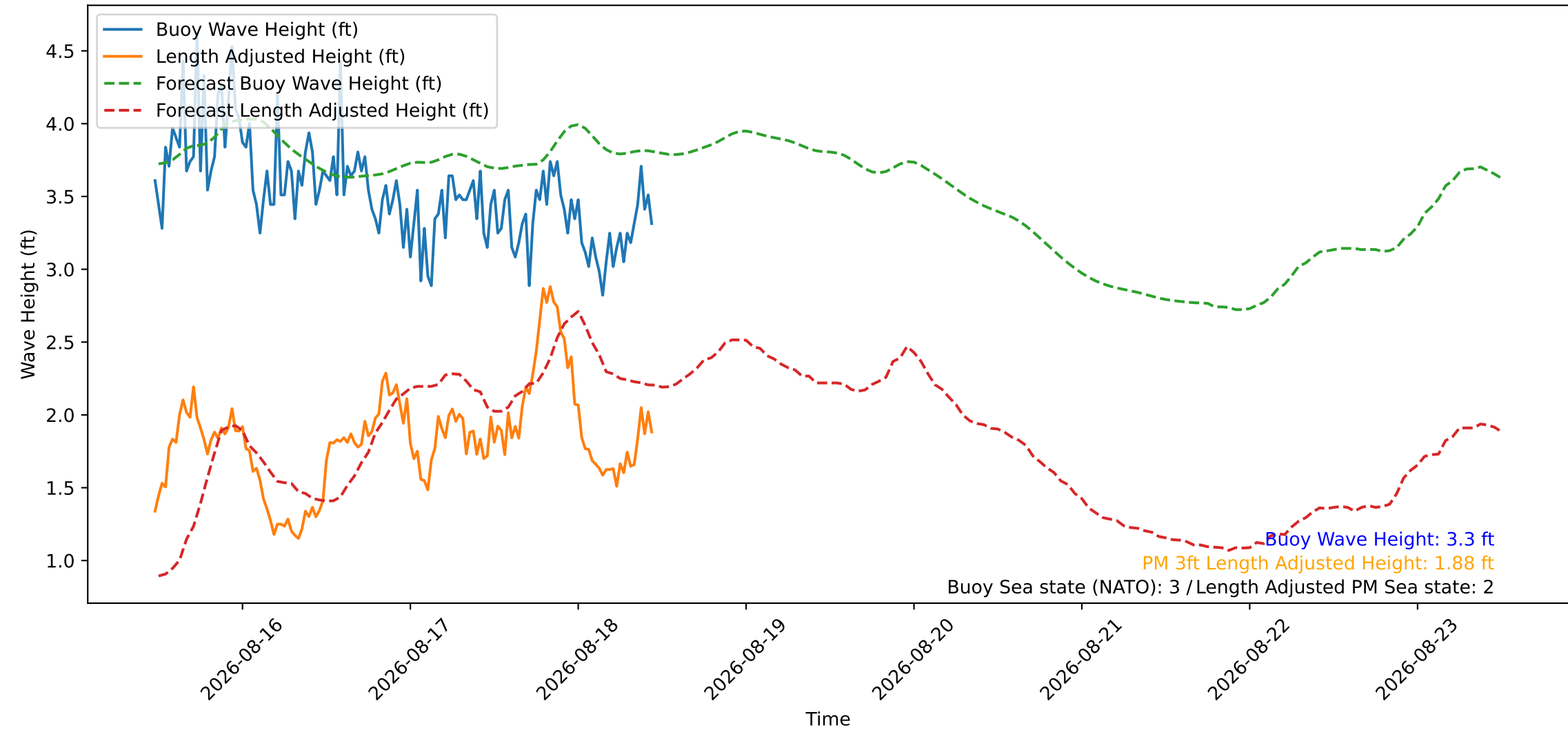
Wave Heights over Time for Oceanside Harbor at 2026-08-18 11:30:26
