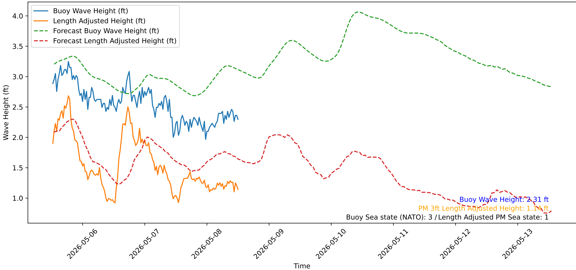
Wave Heights over Time for Oceanside Harbor at 2026-05-08 12:40:31
