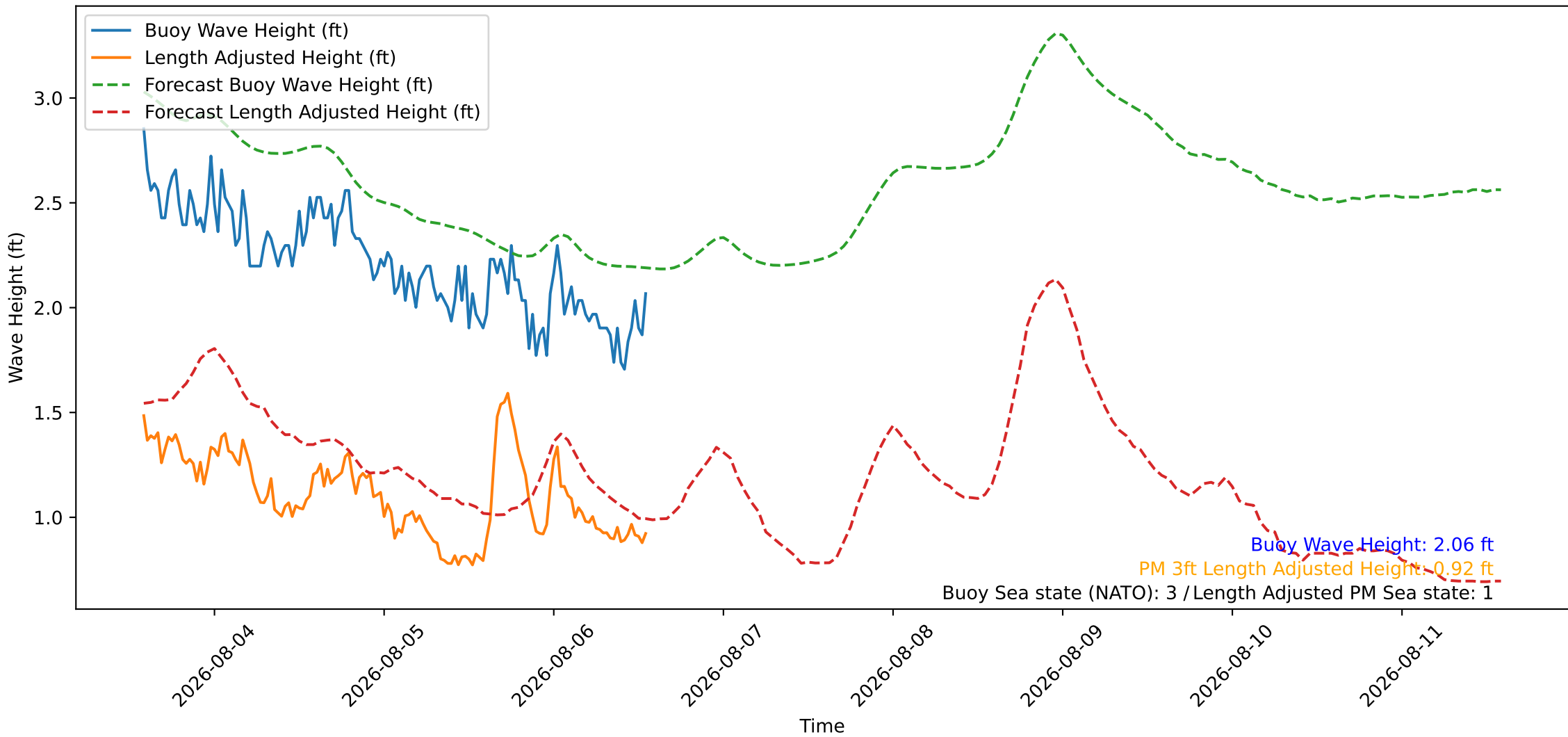
Wave Heights over Time for Oceanside Harbor at 2026-08-06 13:50:26
