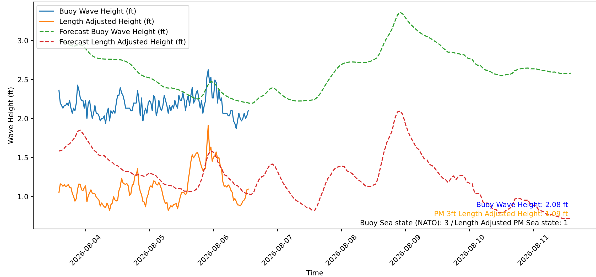
Wave Heights over Time for Green Beach at 2026-08-06 13:51:09
