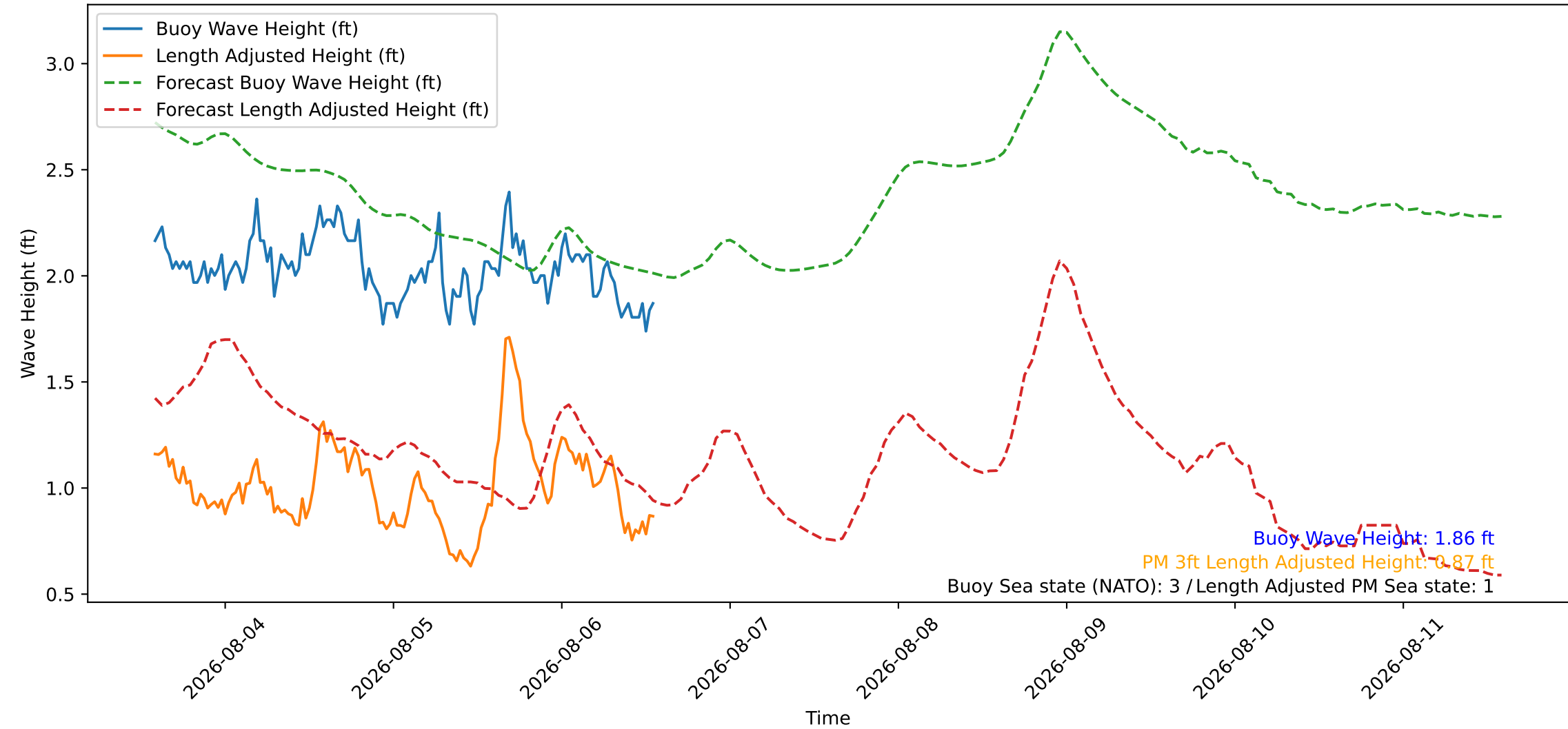
Wave Heights over Time for Red Beach at 2026-08-06 13:50:47
