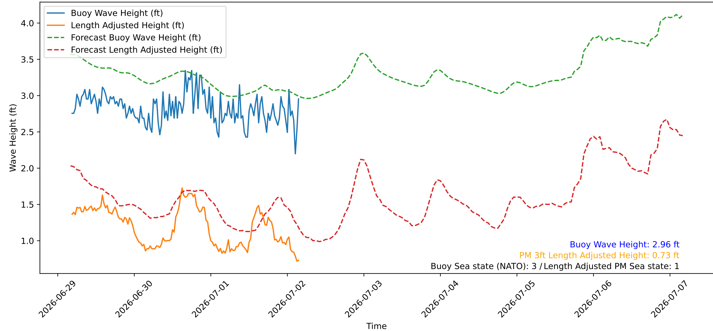
Wave Heights over Time for Red Beach at 2026-07-02 04:10:45
