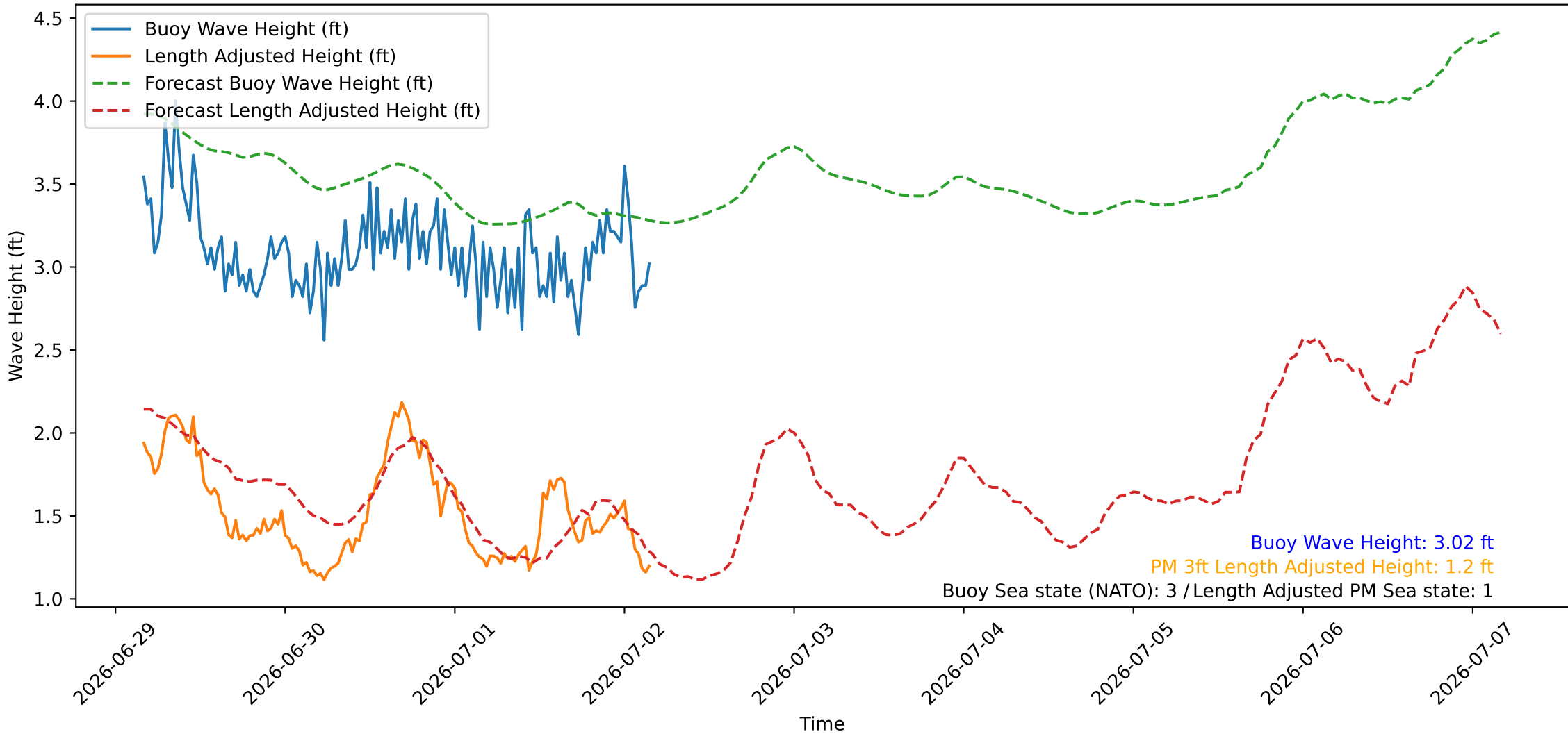
Wave Heights over Time for Oceanside Harbor at 2026-07-02 04:10:26
