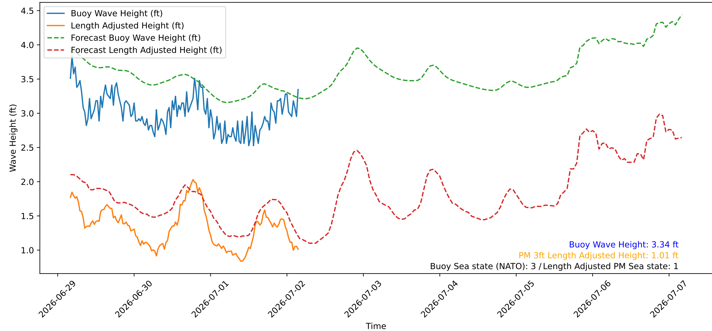
Wave Heights over Time for Green Beach at 2026-07-02 04:11:07
