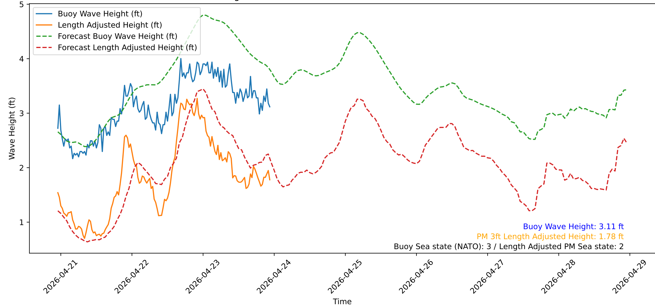
Wave Heights over Time for Green Beach at 2026-04-23 23:11:12
