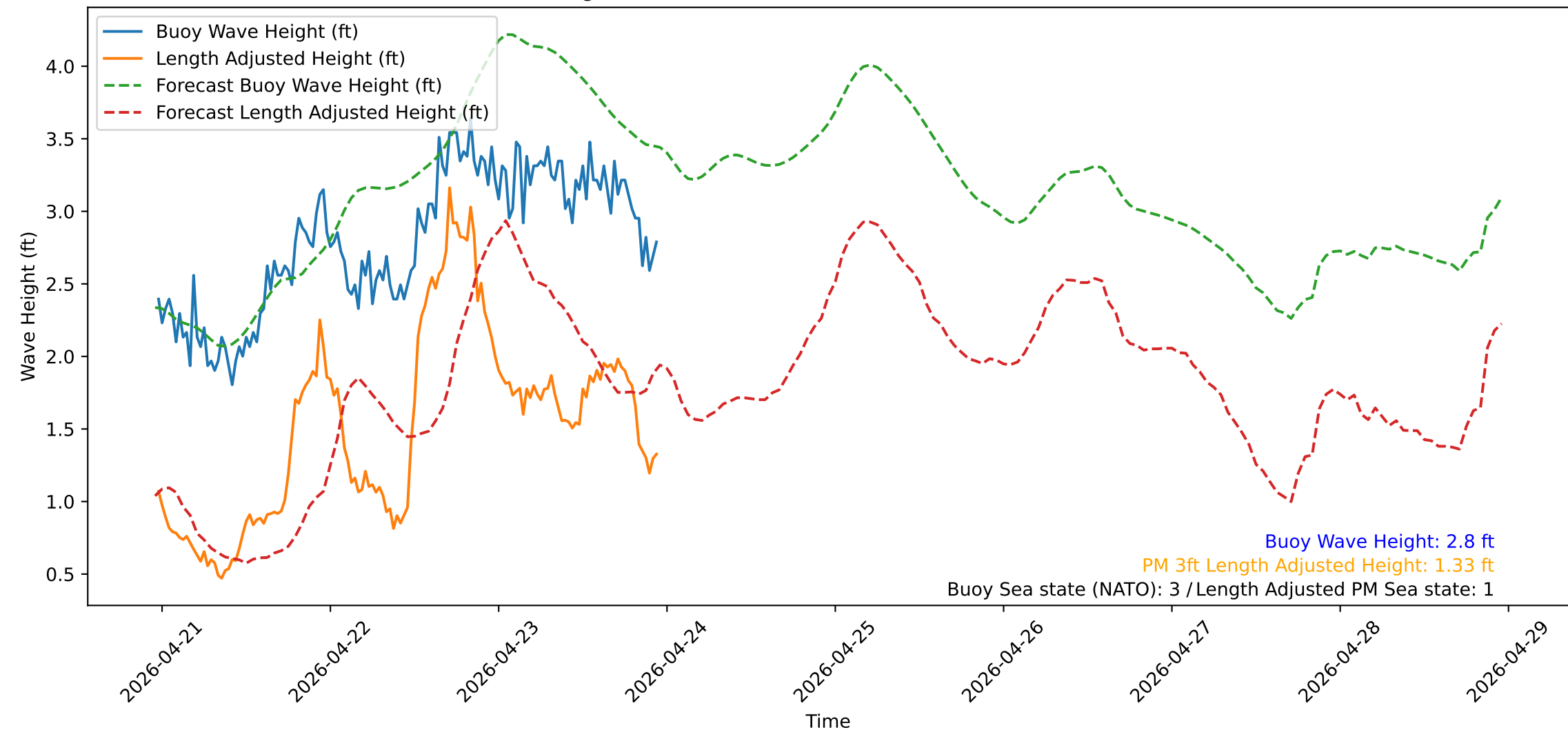
Wave Heights over Time for Red Beach at 2026-04-23 23:10:50
