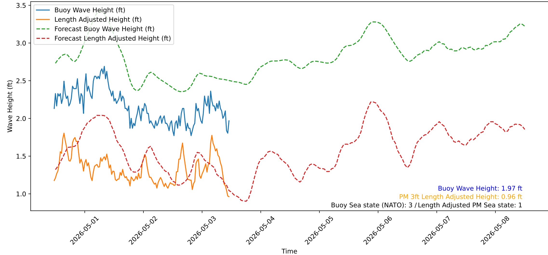
Wave Heights over Time for Oceanside Harbor at 2026-05-03 11:40:31
