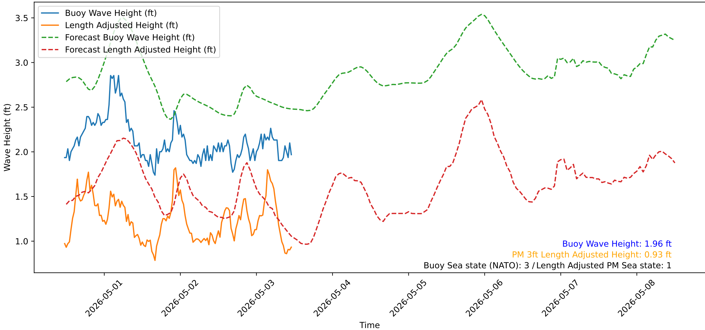
Wave Heights over Time for Green Beach at 2026-05-03 11:41:13
