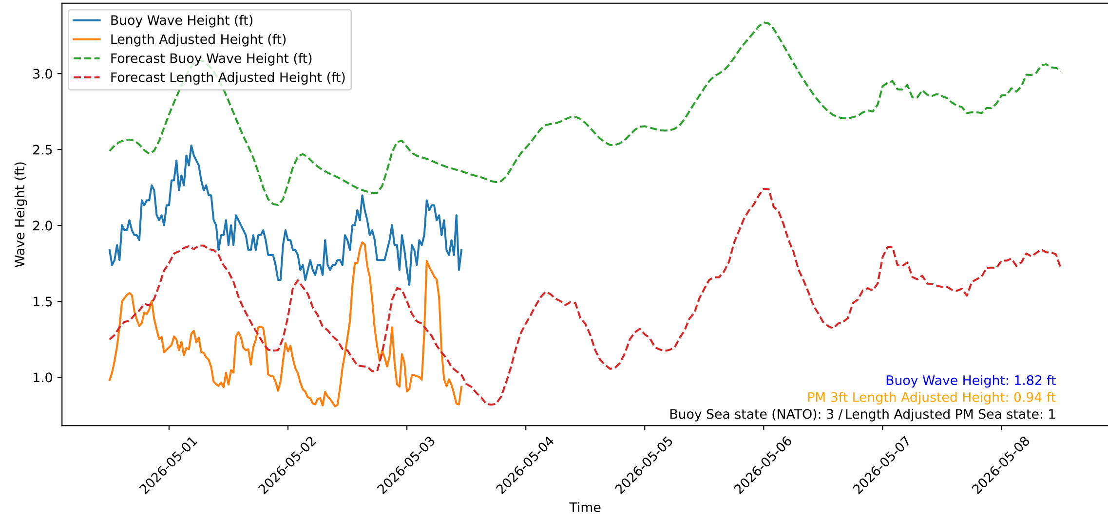
Wave Heights over Time for Red Beach at 2026-05-03 11:40:50
