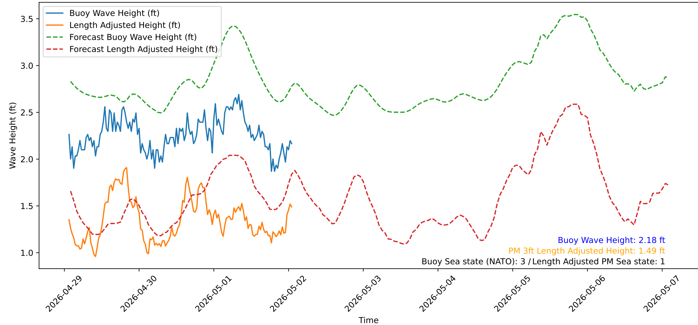
Wave Heights over Time for Oceanside Harbor at 2026-05-02 01:40:32
