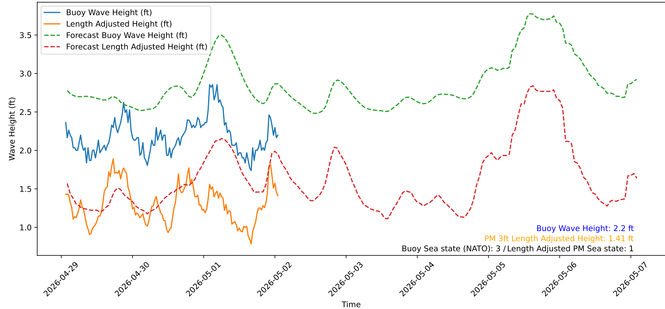
Wave Heights over Time for Green Beach at 2026-05-02 01:41:14
