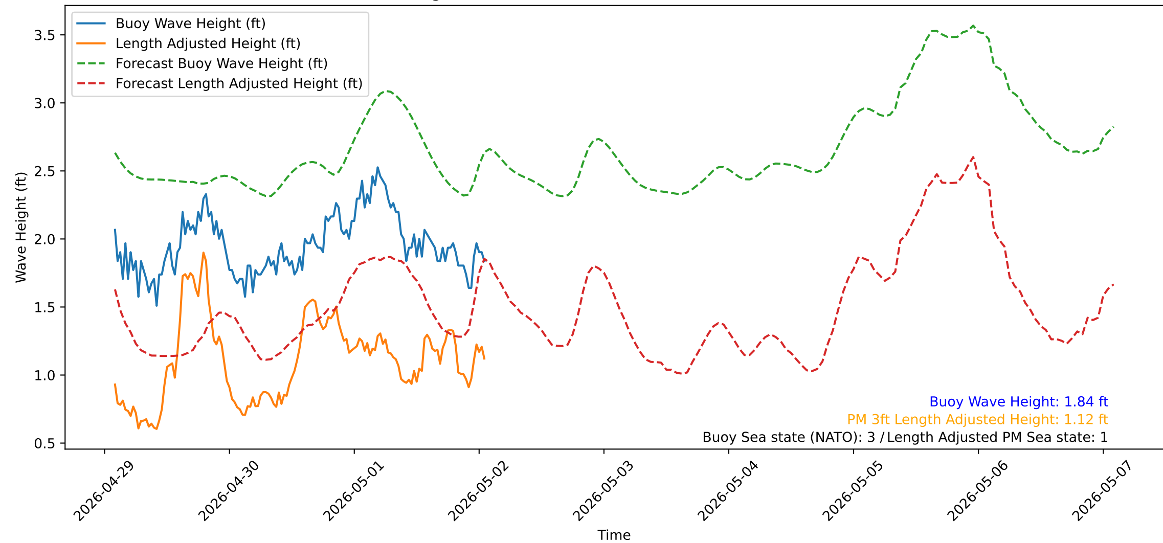
Wave Heights over Time for Red Beach at 2026-05-02 01:40:51
