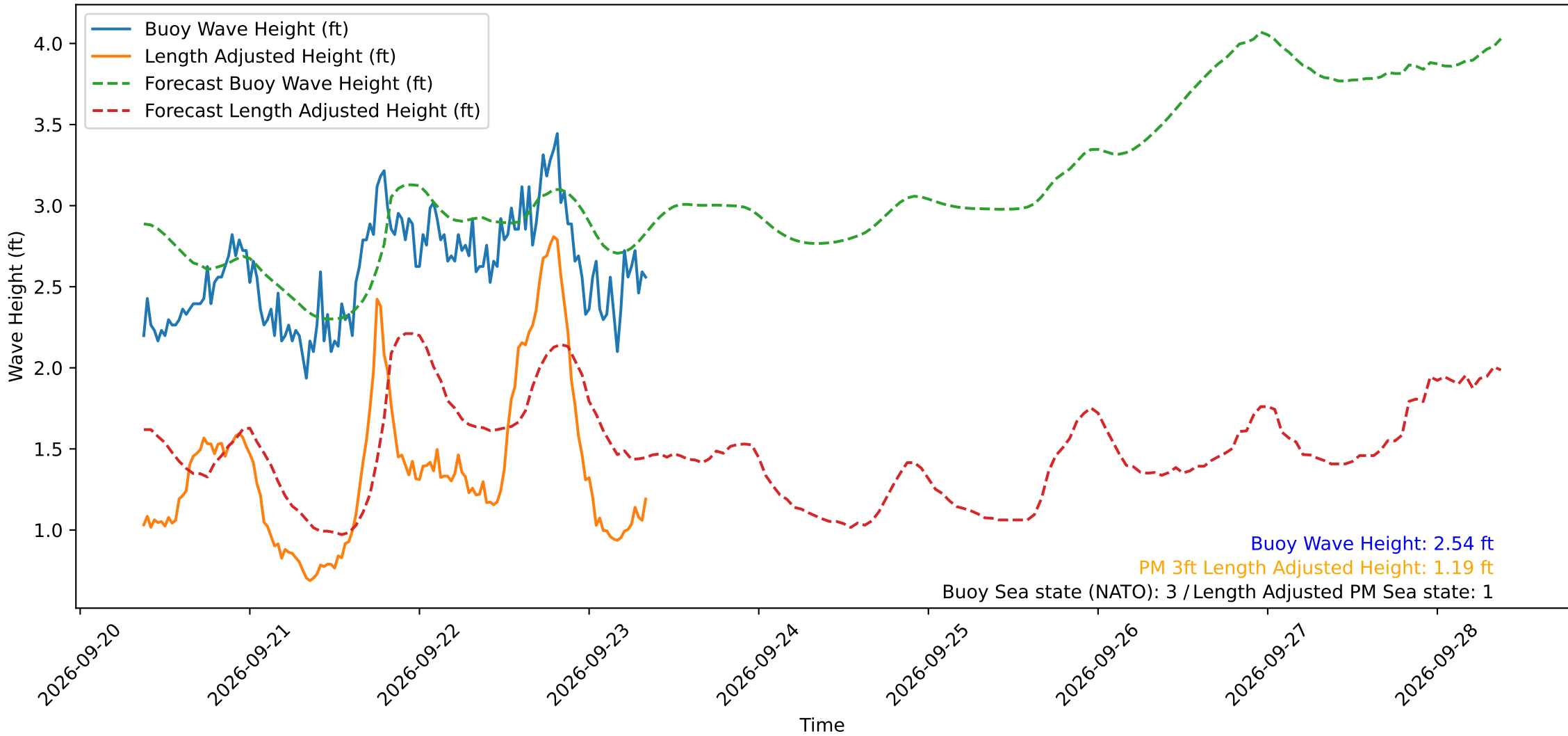
Wave Heights over Time for Green Beach at 2026-09-23 08:51:38
