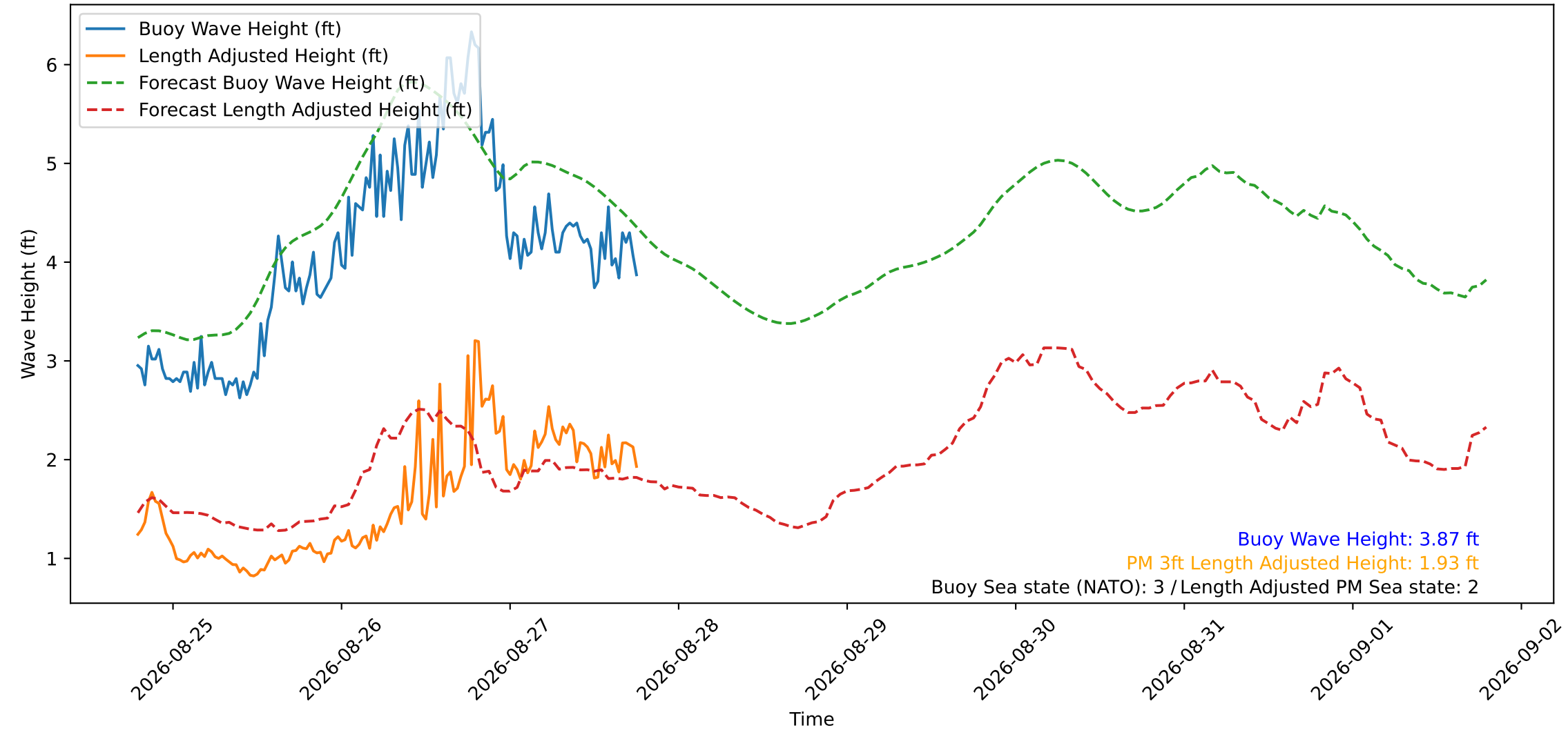
Wave Heights over Time for Green Beach at 2026-08-27 18:41:13
