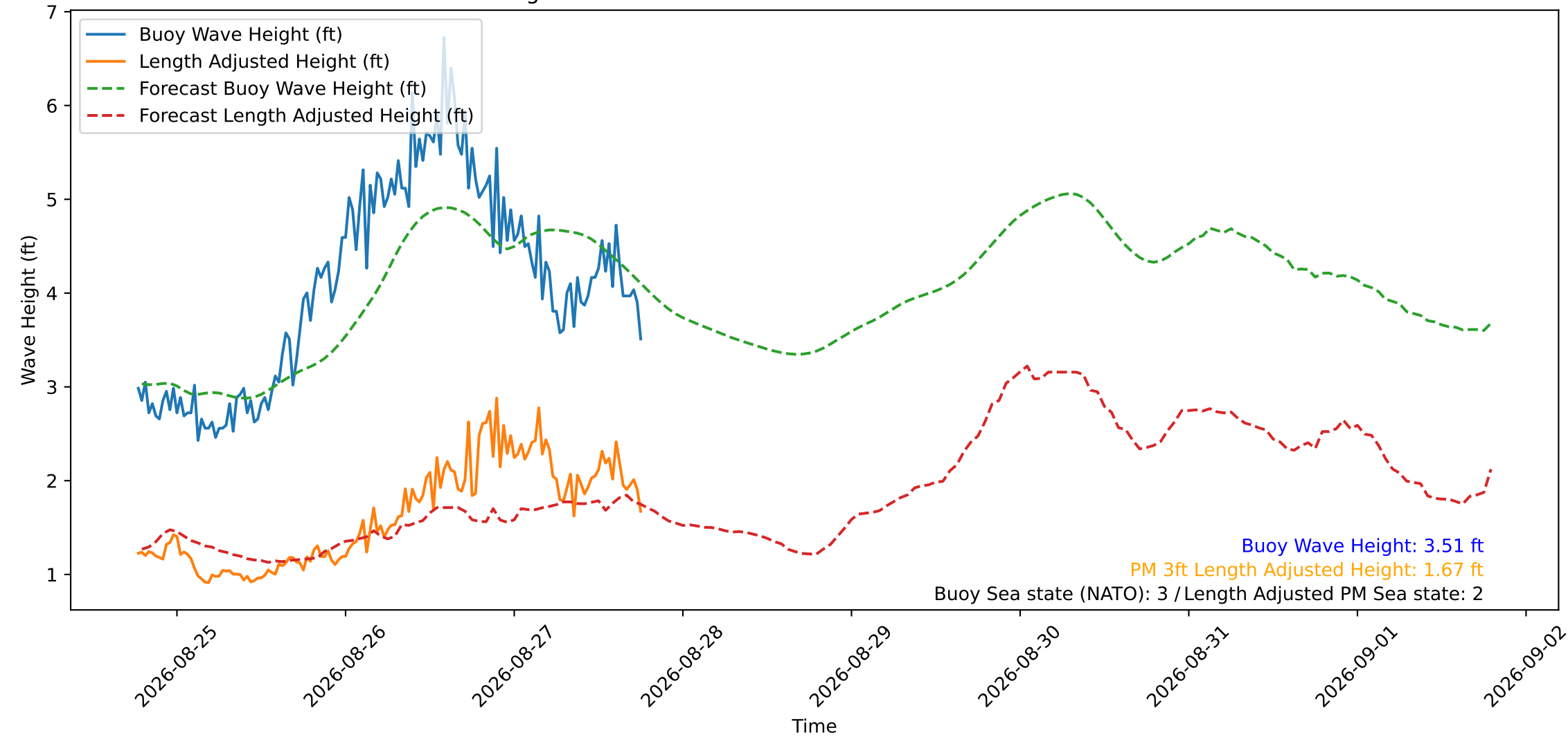
Wave Heights over Time for Oceanside Harbor at 2026-08-27 18:40:30
