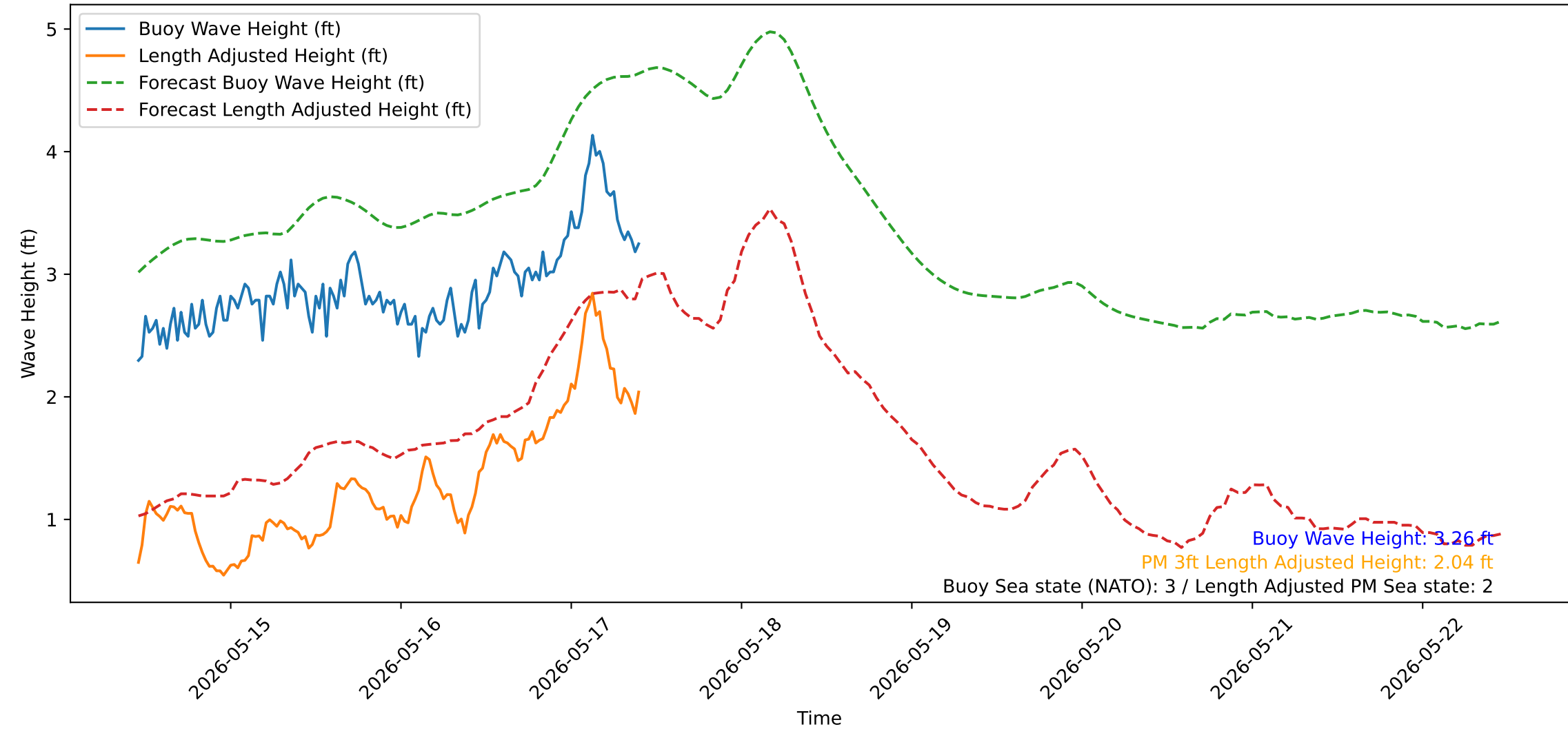
Wave Heights over Time for Red Beach at 2026-05-17 10:30:51
