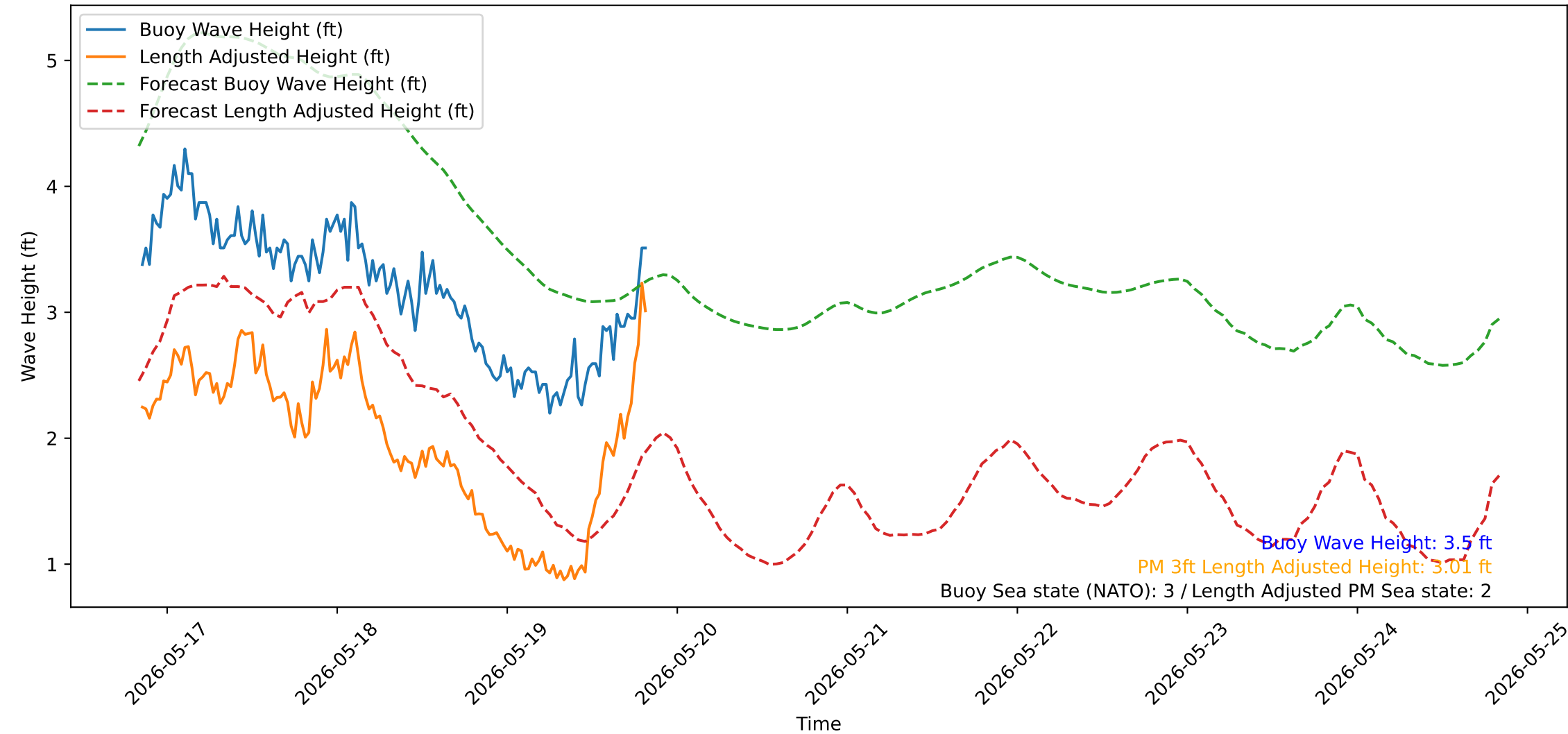
Wave Heights over Time for Oceanside Harbor at 2026-05-19 20:20:32
