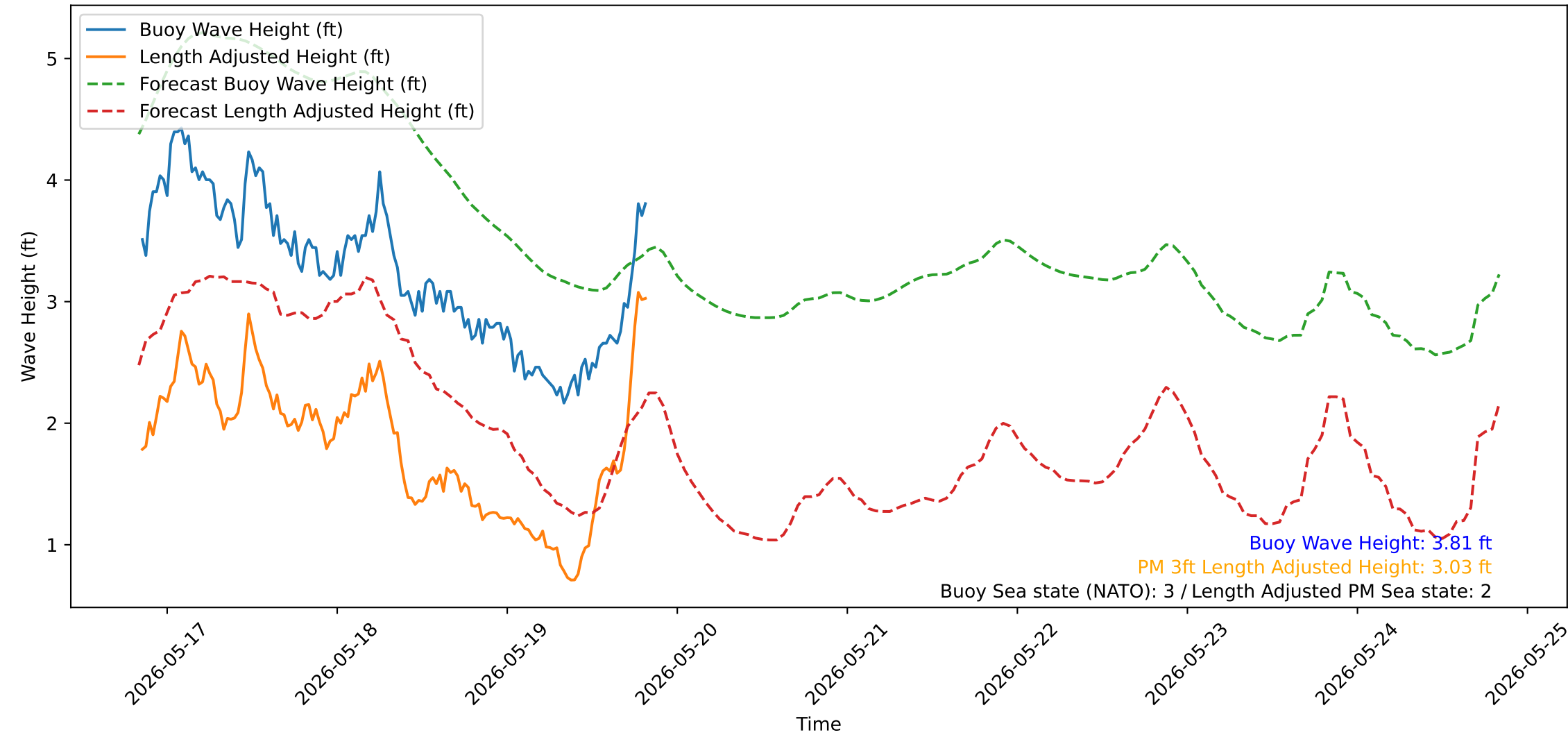
Wave Heights over Time for Green Beach at 2026-05-19 20:21:16
