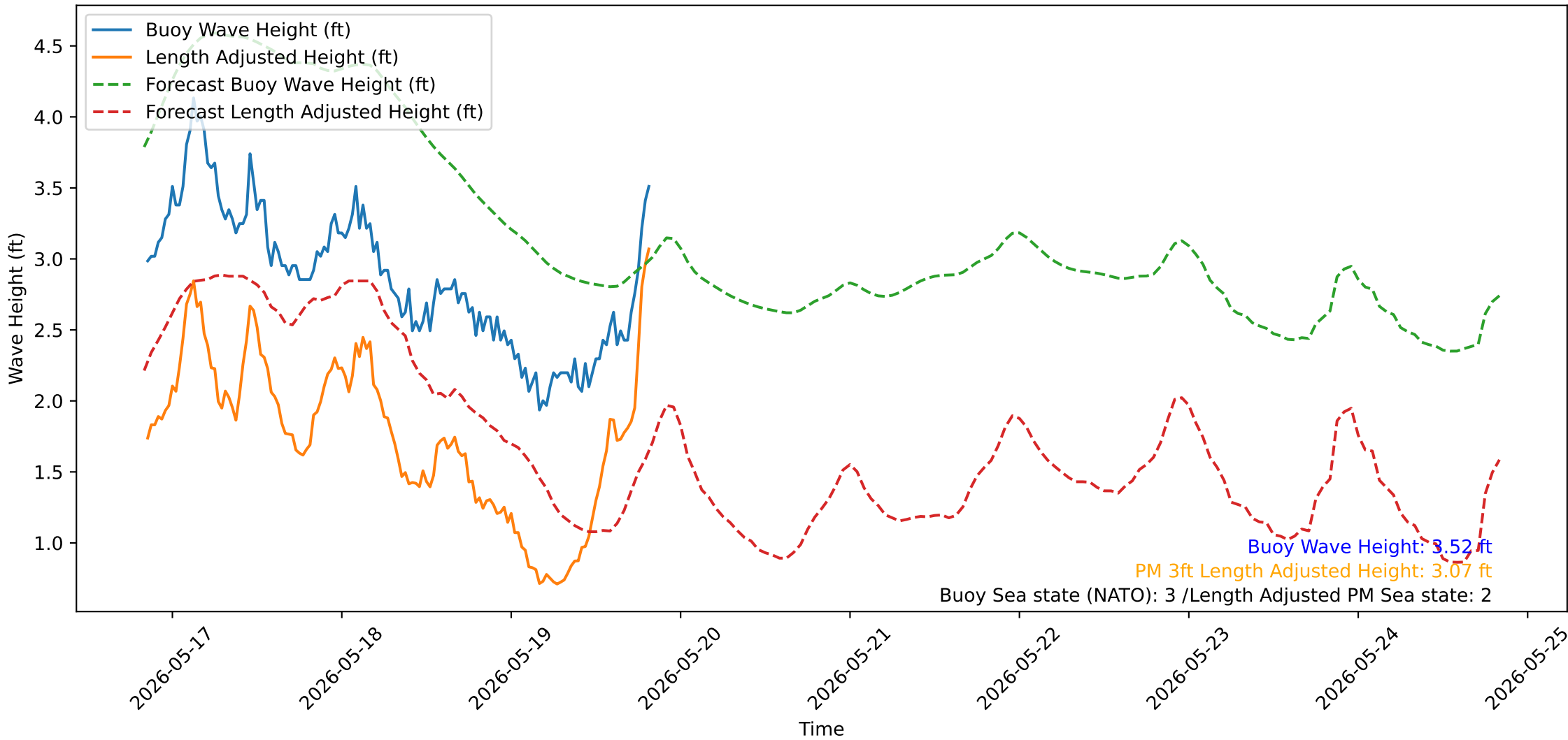
Wave Heights over Time for Red Beach at 2026-05-19 20:20:53
