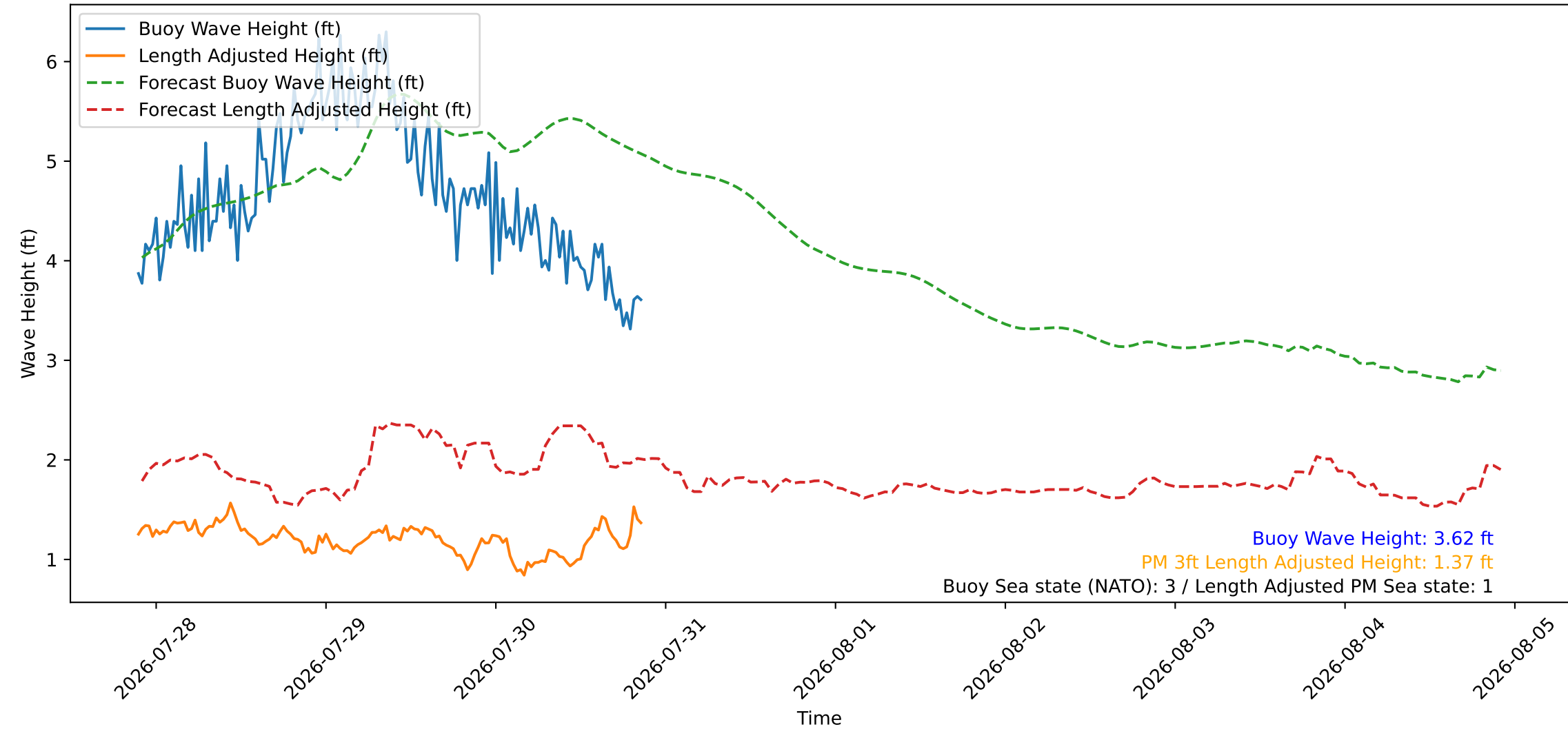
Wave Heights over Time for Green Beach at 2026-07-30 21:31:08
