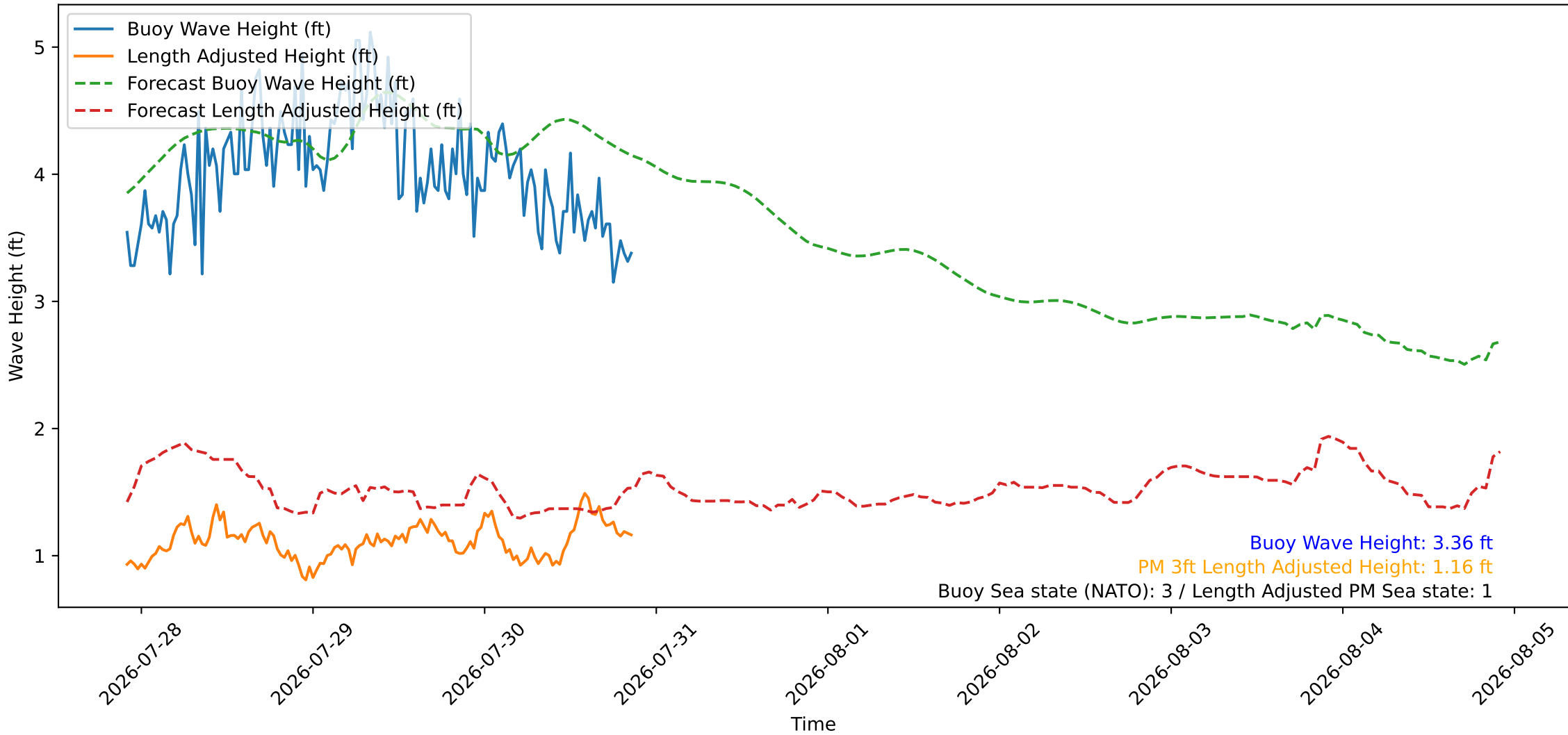
Wave Heights over Time for Red Beach at 2026-07-30 21:30:45
