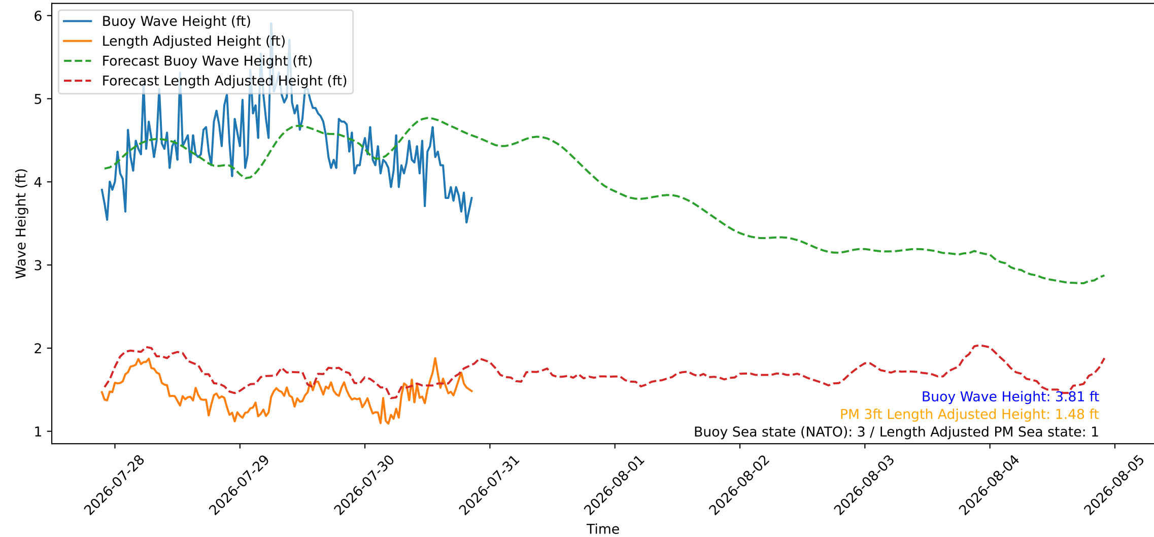
Wave Heights over Time for Oceanside Harbor at 2026-07-30 21:30:26
