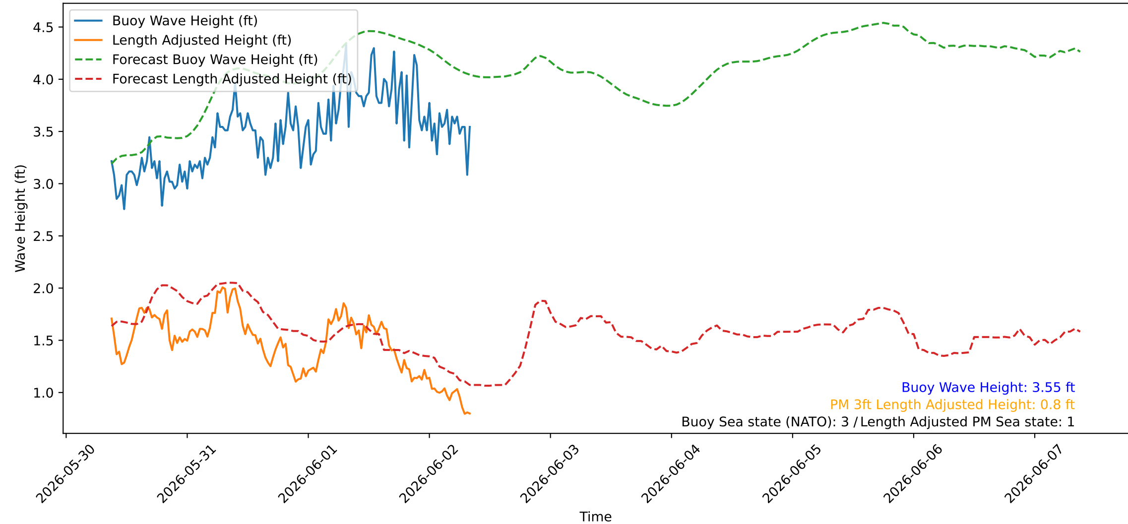
Wave Heights over Time for Green Beach at 2026-06-02 08:51:11
