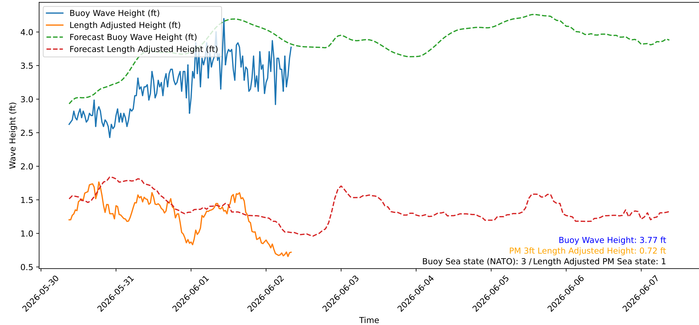
Wave Heights over Time for Red Beach at 2026-06-02 08:50:48
