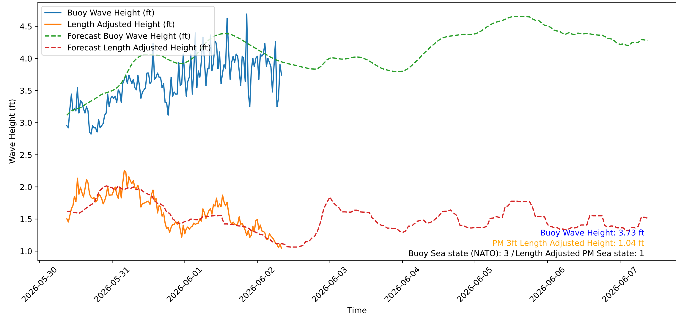
Wave Heights over Time for Oceanside Harbor at 2026-06-02 08:50:27
