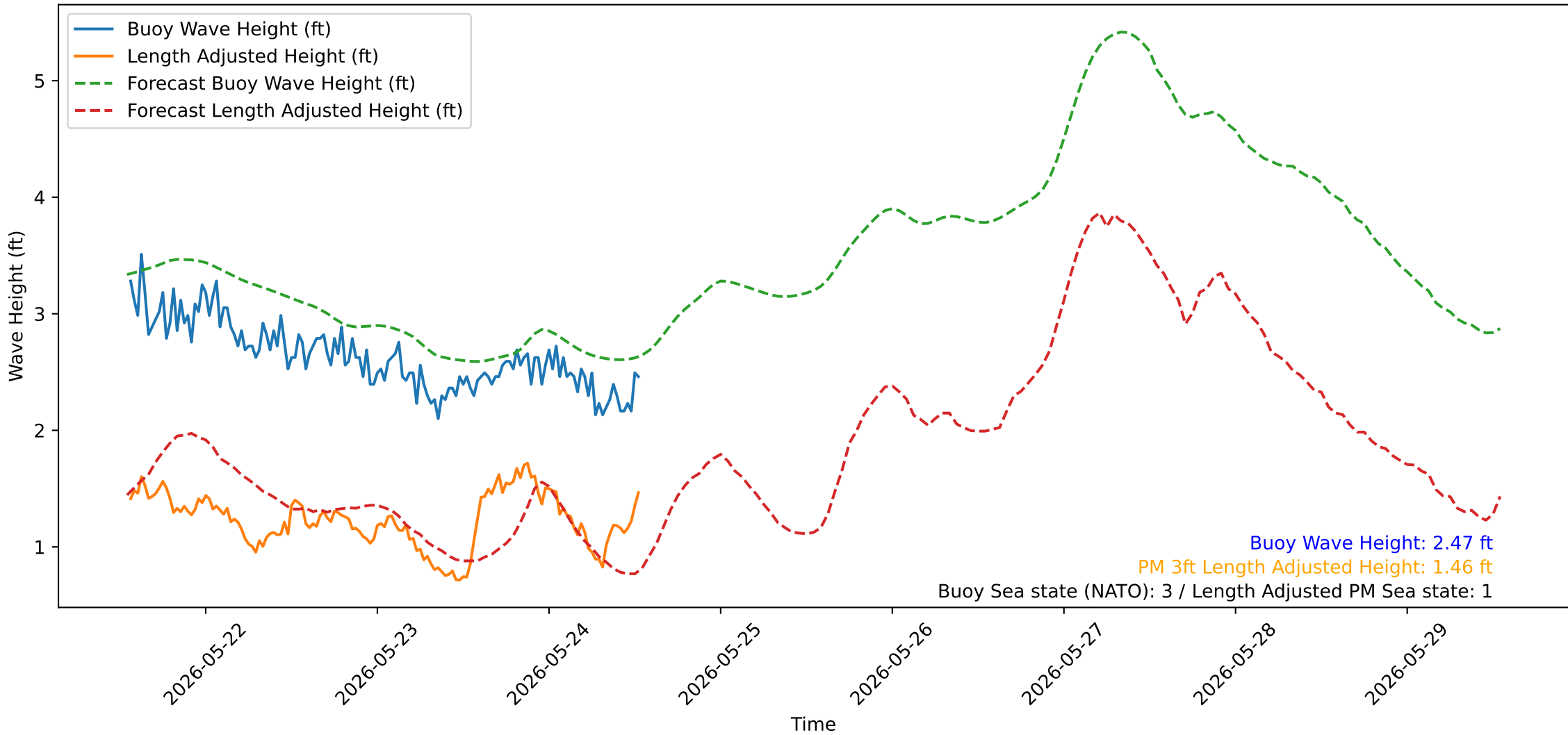
Wave Heights over Time for Oceanside Harbor at 2026-05-24 13:20:31
