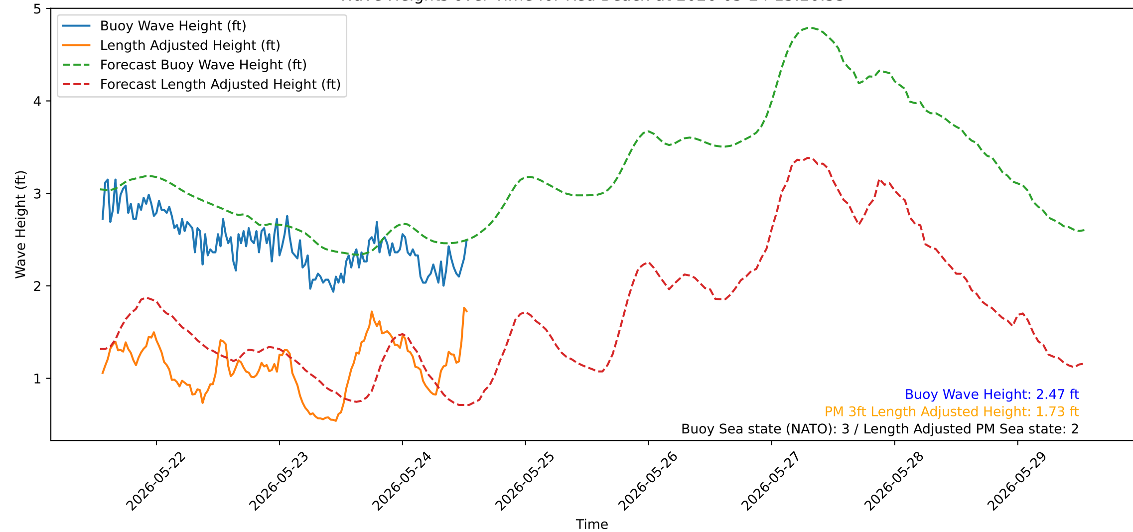
Wave Heights over Time for Red Beach at 2026-05-24 13:20:53
