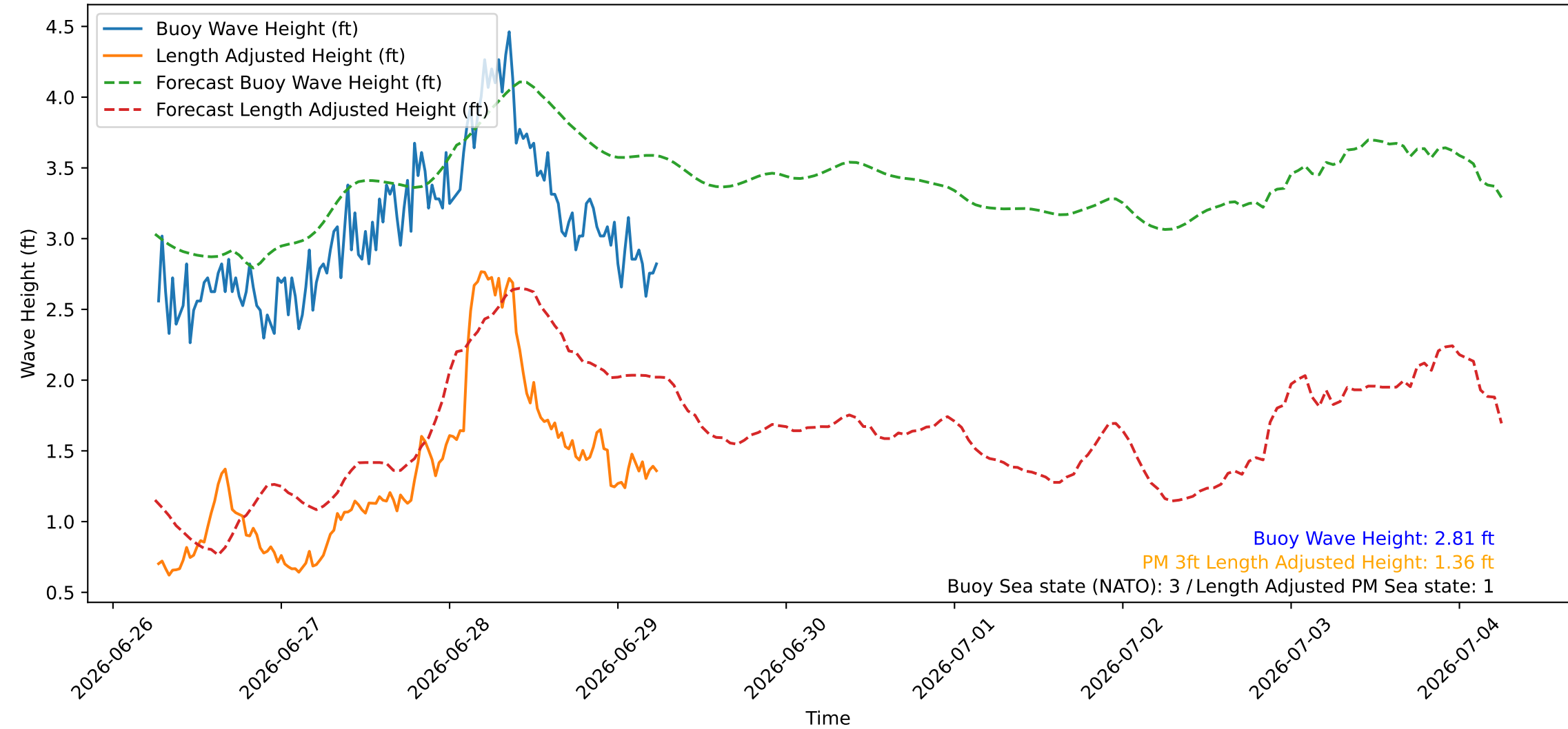
Wave Heights over Time for Red Beach at 2026-06-29 06:20:46
