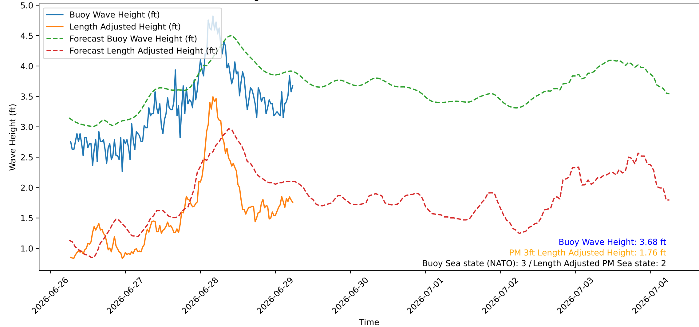
Wave Heights over Time for Green Beach at 2026-06-29 06:21:08
