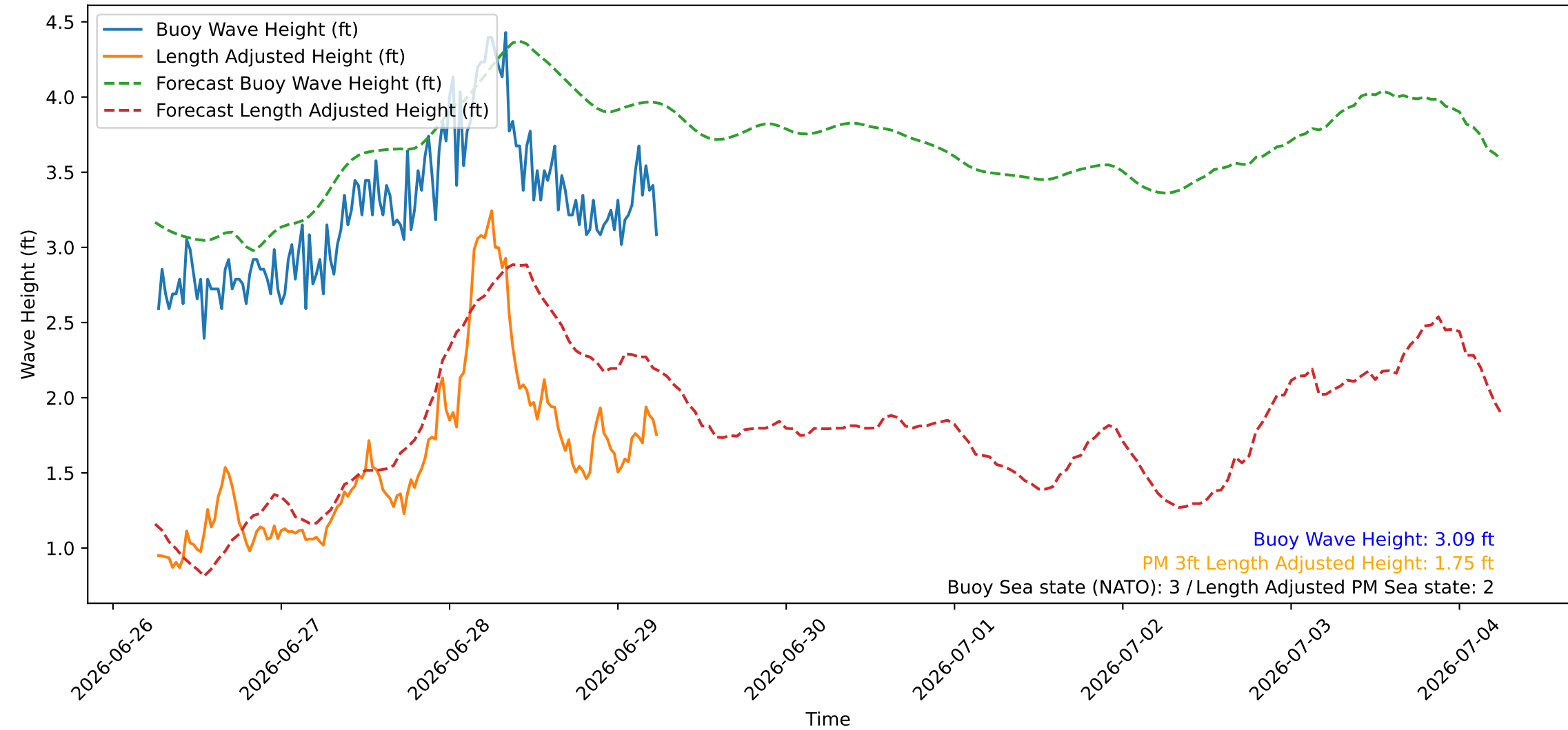
Wave Heights over Time for Oceanside Harbor at 2026-06-29 06:20:26
