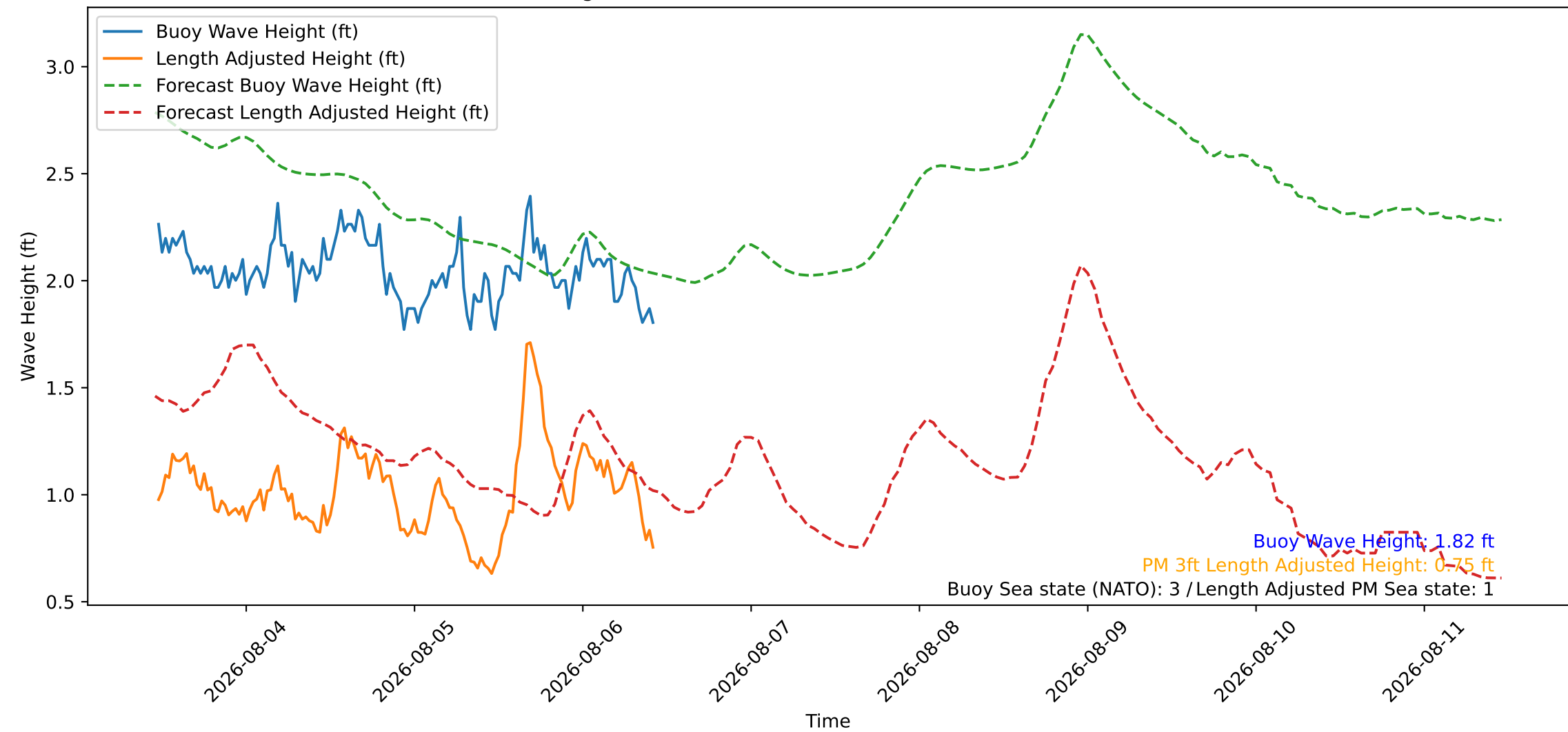
Wave Heights over Time for Red Beach at 2026-08-06 11:10:45
