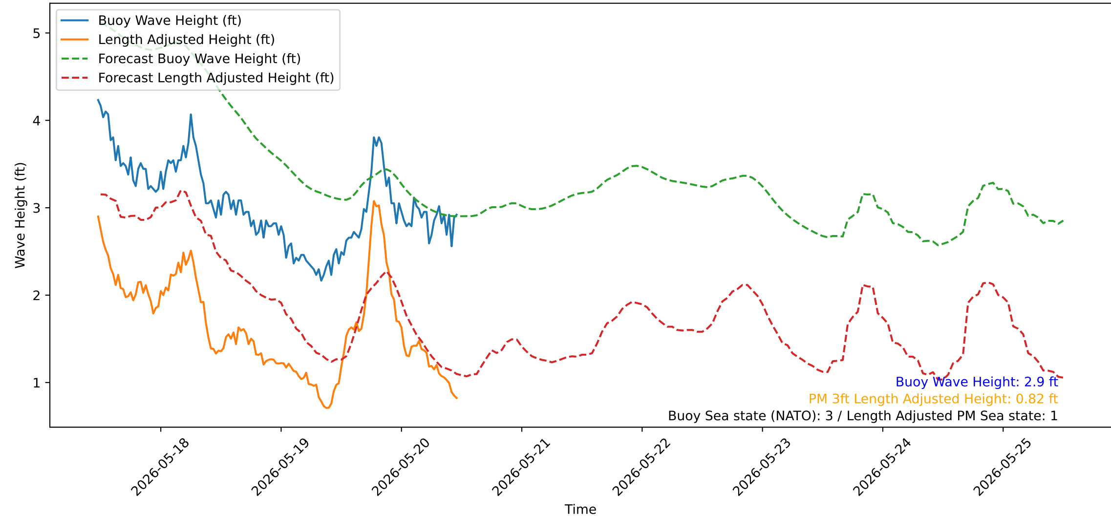
Wave Heights over Time for Green Beach at 2026-05-20 11:41:13
