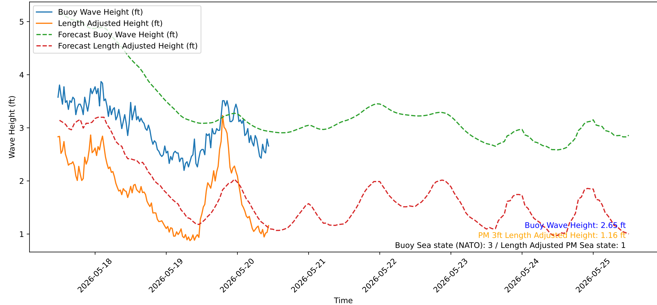
Wave Heights over Time for Oceanside Harbor at 2026-05-20 11:40:31
