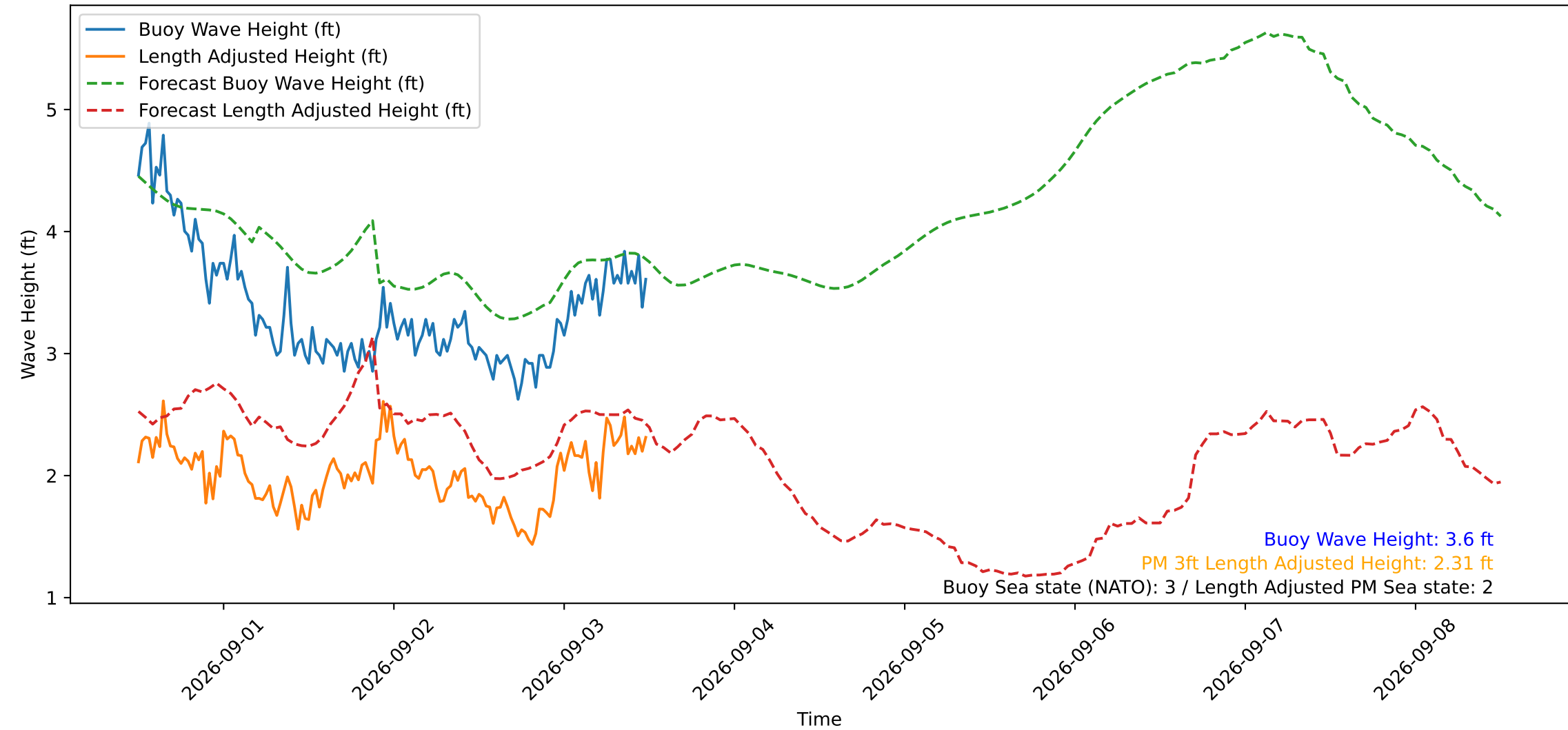
Wave Heights over Time for Oceanside Harbor at 2026-09-03 12:10:30
