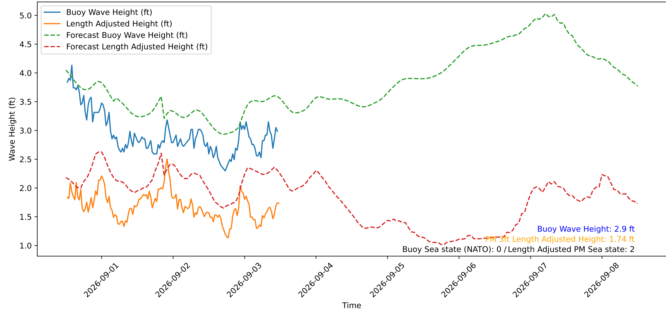
Wave Heights over Time for Red Beach at 2026-09-03 12:10:50
