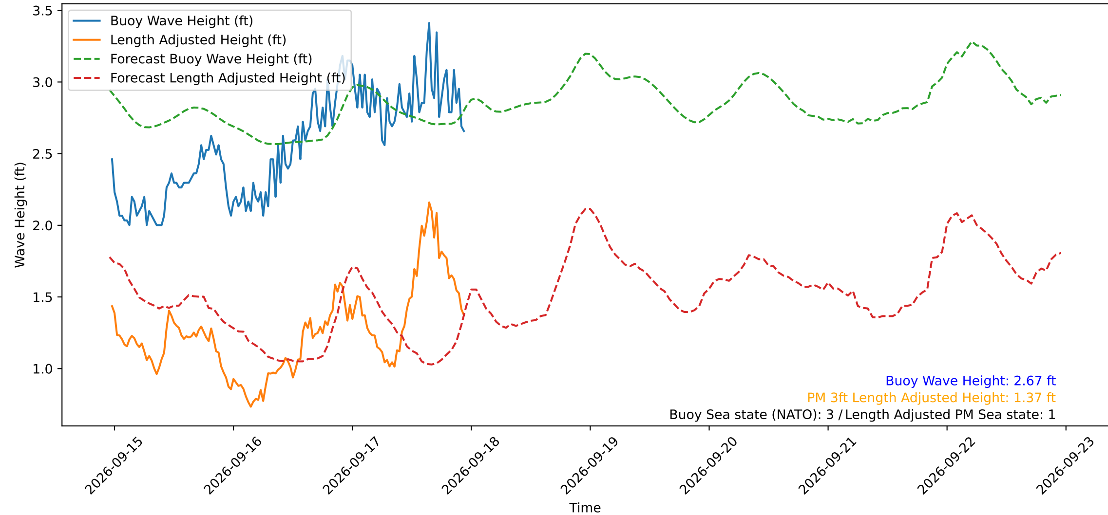
Wave Heights over Time for Red Beach at 2026-09-17 23:20:51
