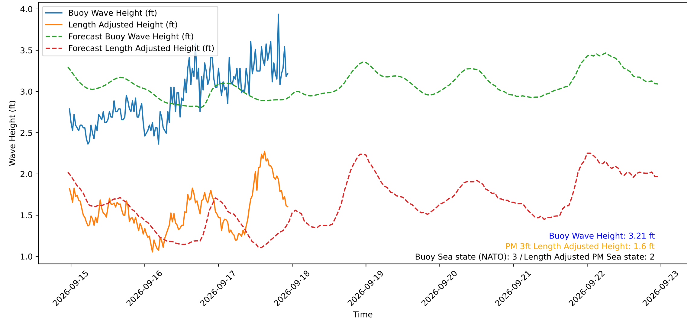
Wave Heights over Time for Oceanside Harbor at 2026-09-17 23:20:30
