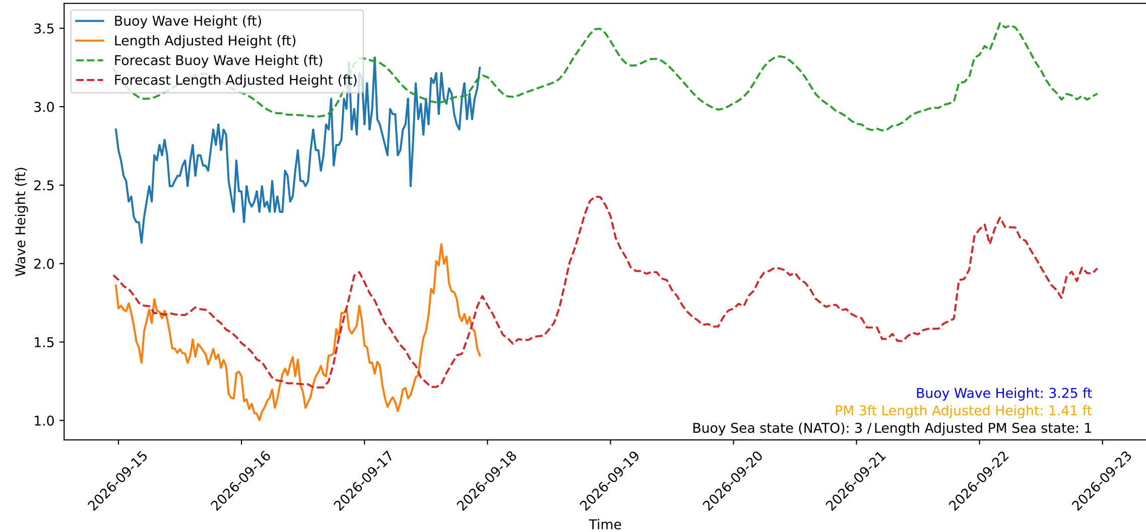
Wave Heights over Time for Green Beach at 2026-09-17 23:21:15
