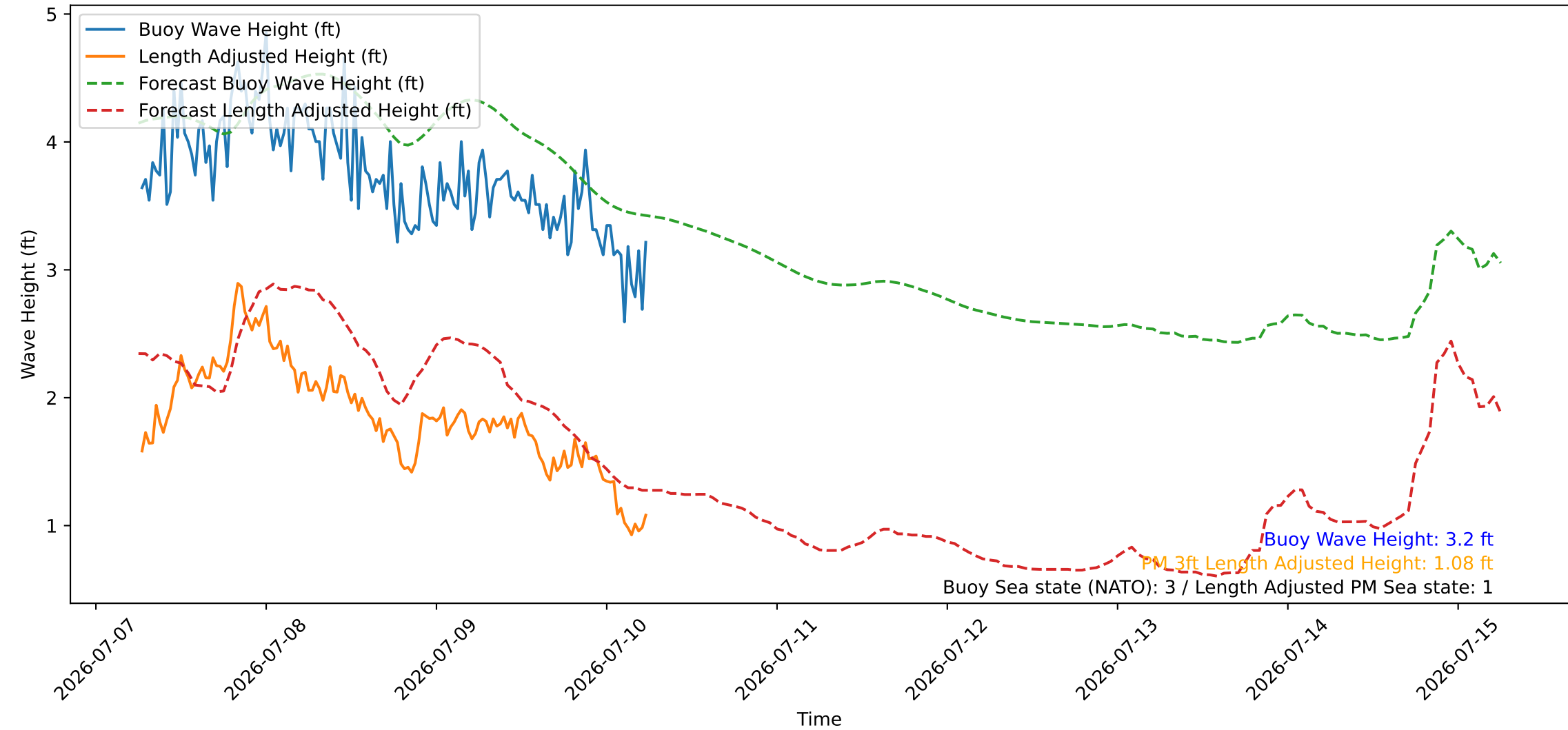
Wave Heights over Time for Red Beach at 2026-07-10 06:20:46
