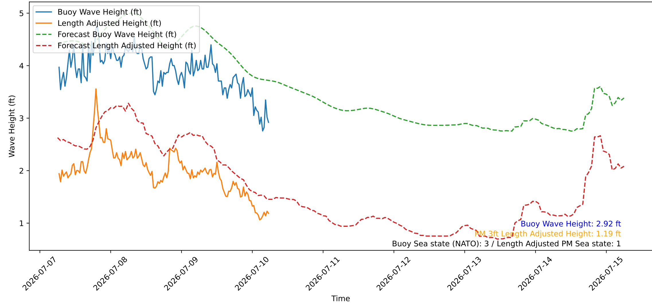
Wave Heights over Time for Green Beach at 2026-07-10 06:21:08
