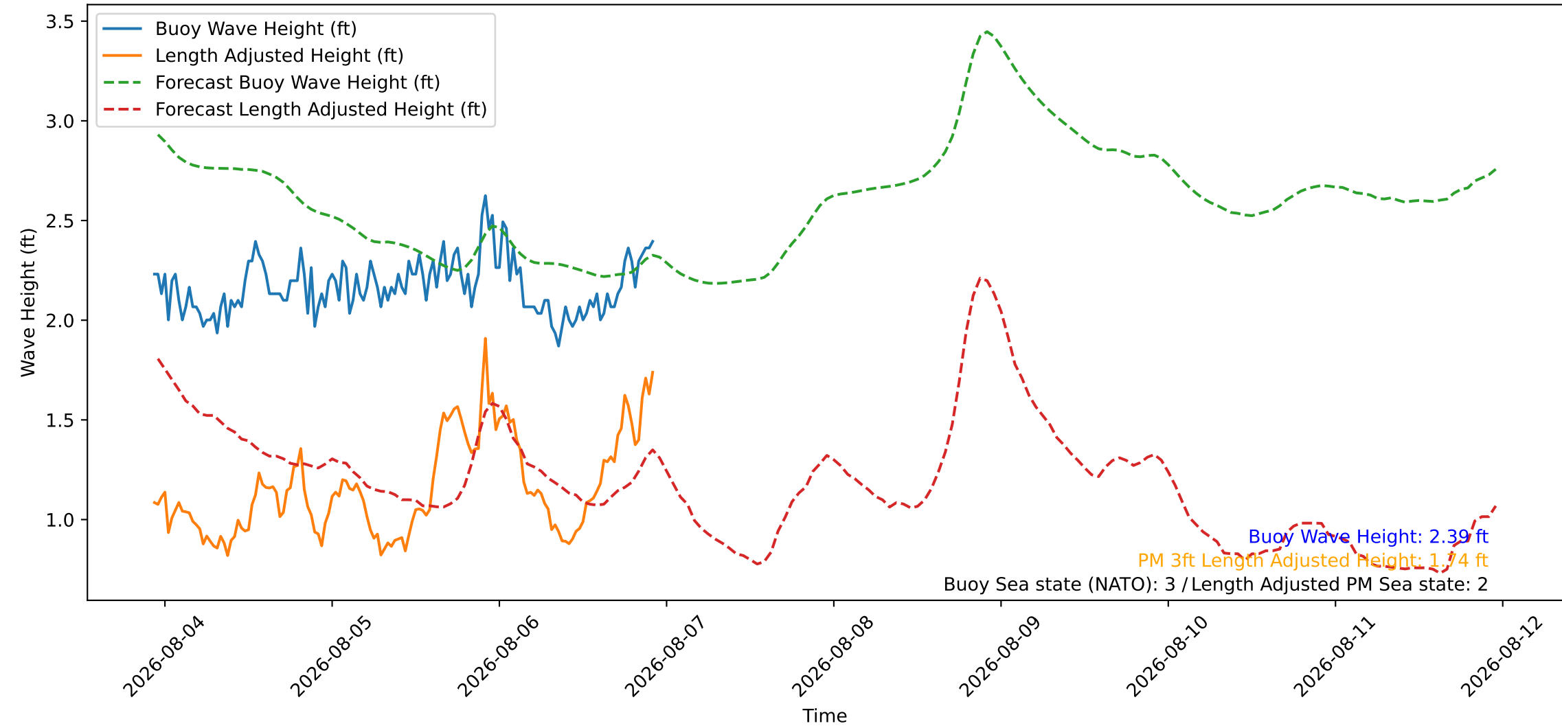
Wave Heights over Time for Green Beach at 2026-08-06 22:41:08
