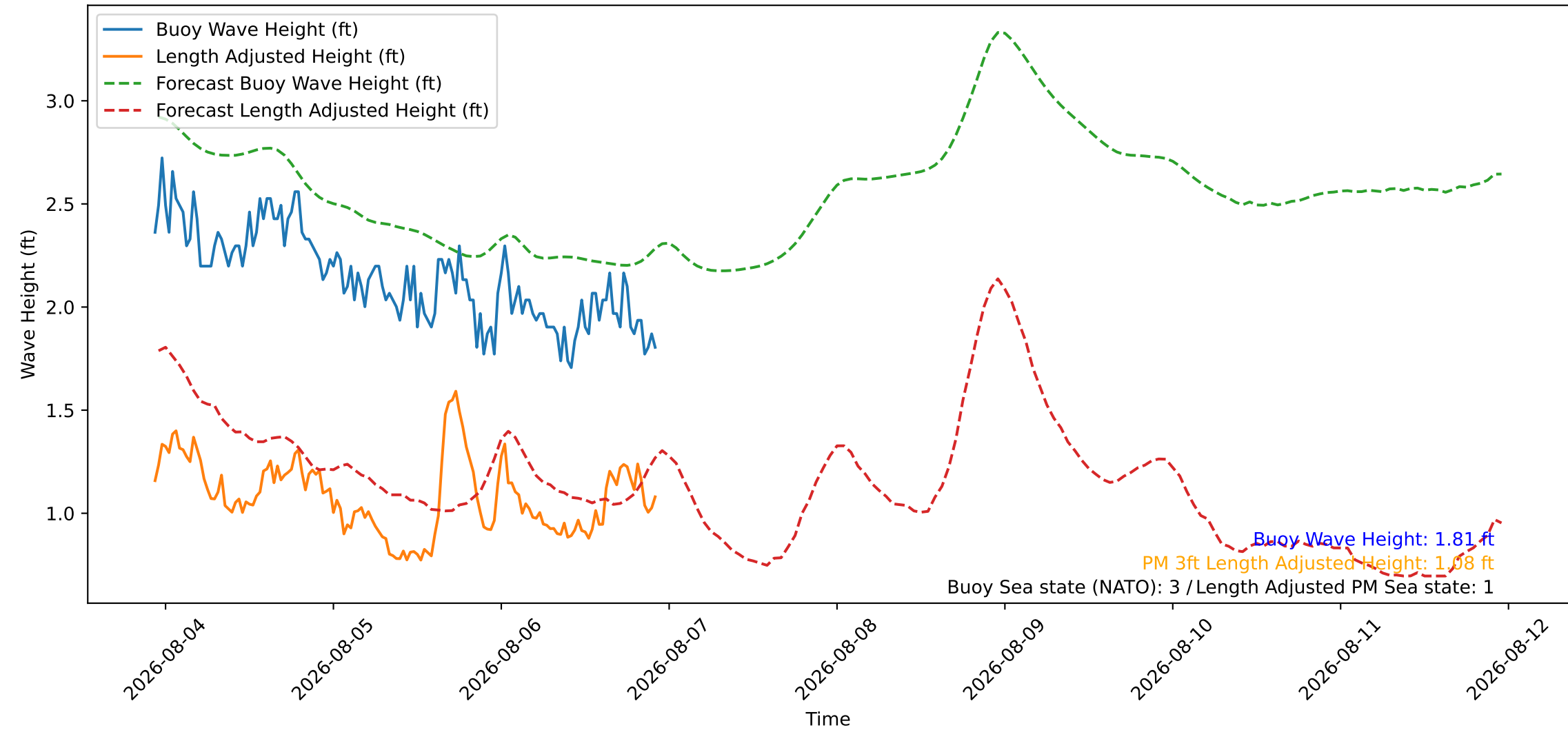
Wave Heights over Time for Oceanside Harbor at 2026-08-06 22:40:26
