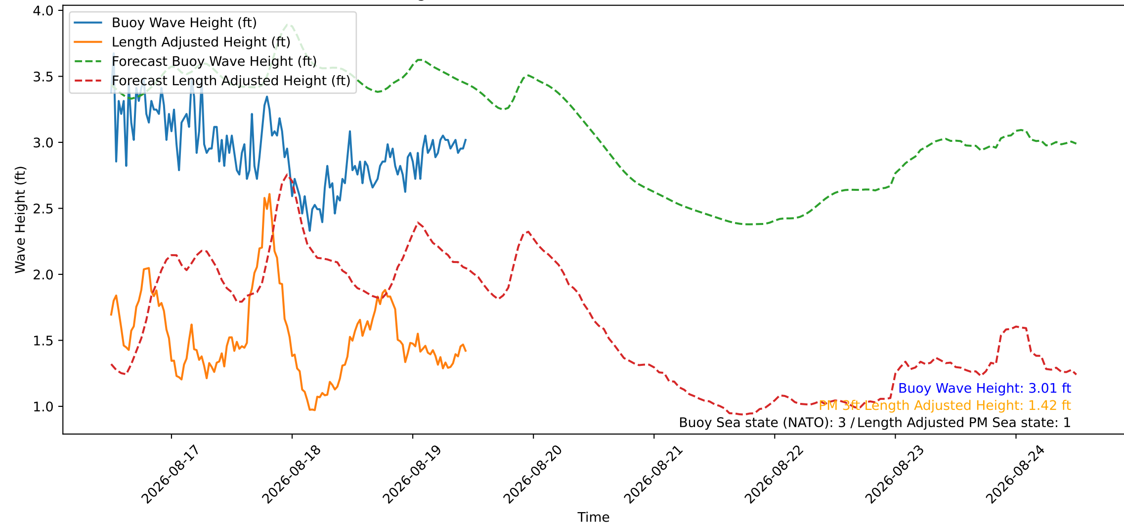
Wave Heights over Time for Red Beach at 2026-08-19 11:50:48
