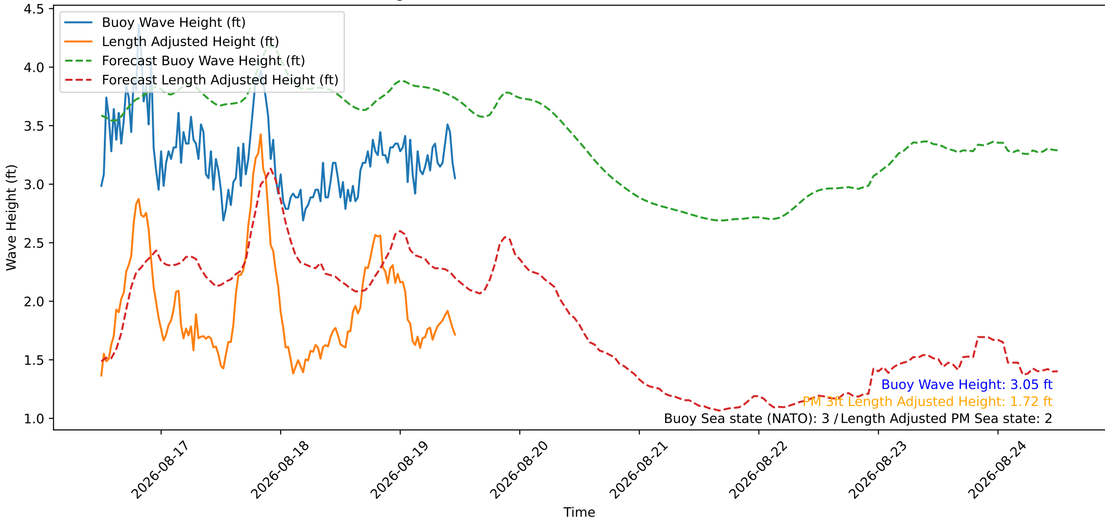
Wave Heights over Time for Green Beach at 2026-08-19 11:51:11
