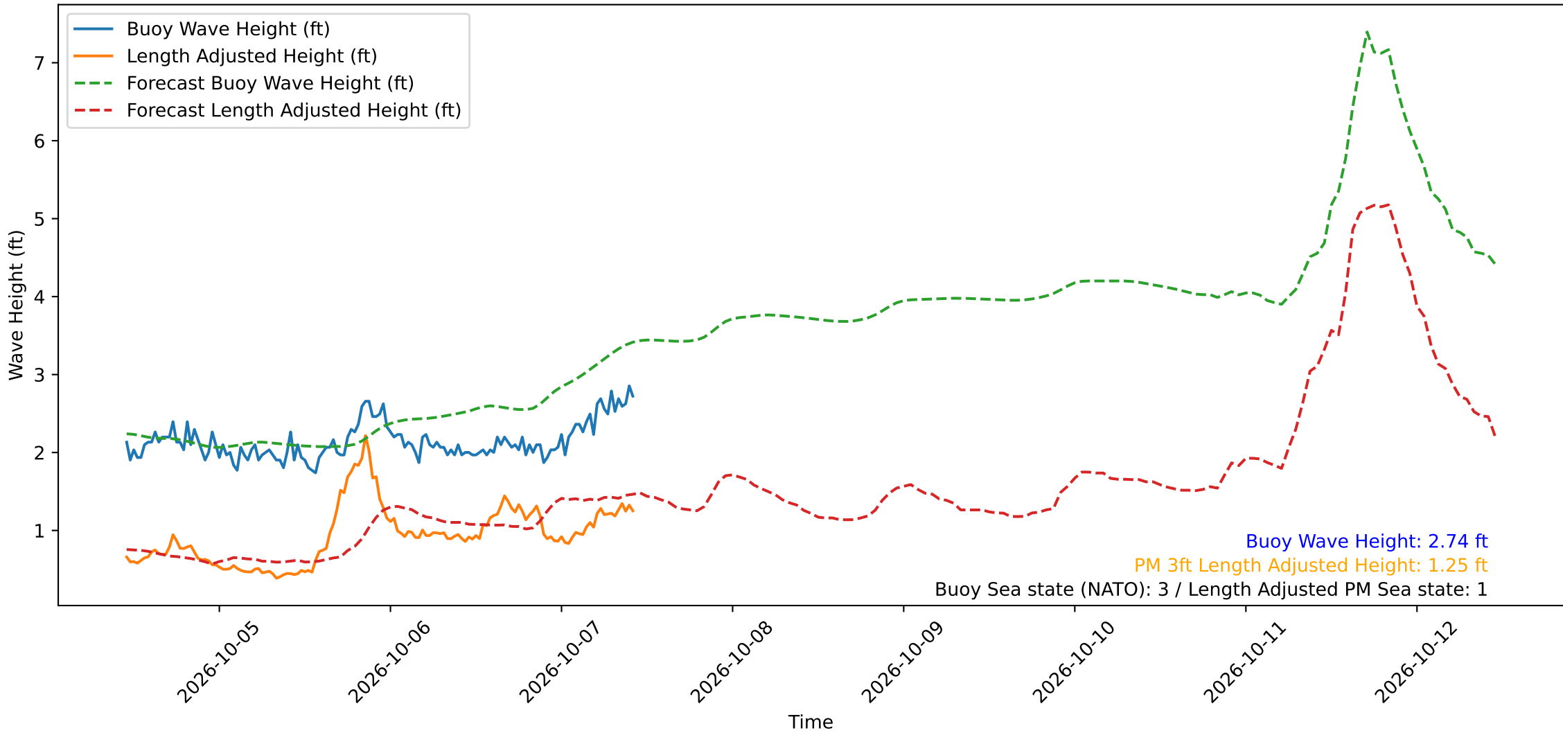
Wave Heights over Time for Red Beach at 2026-10-07 10:50:50
