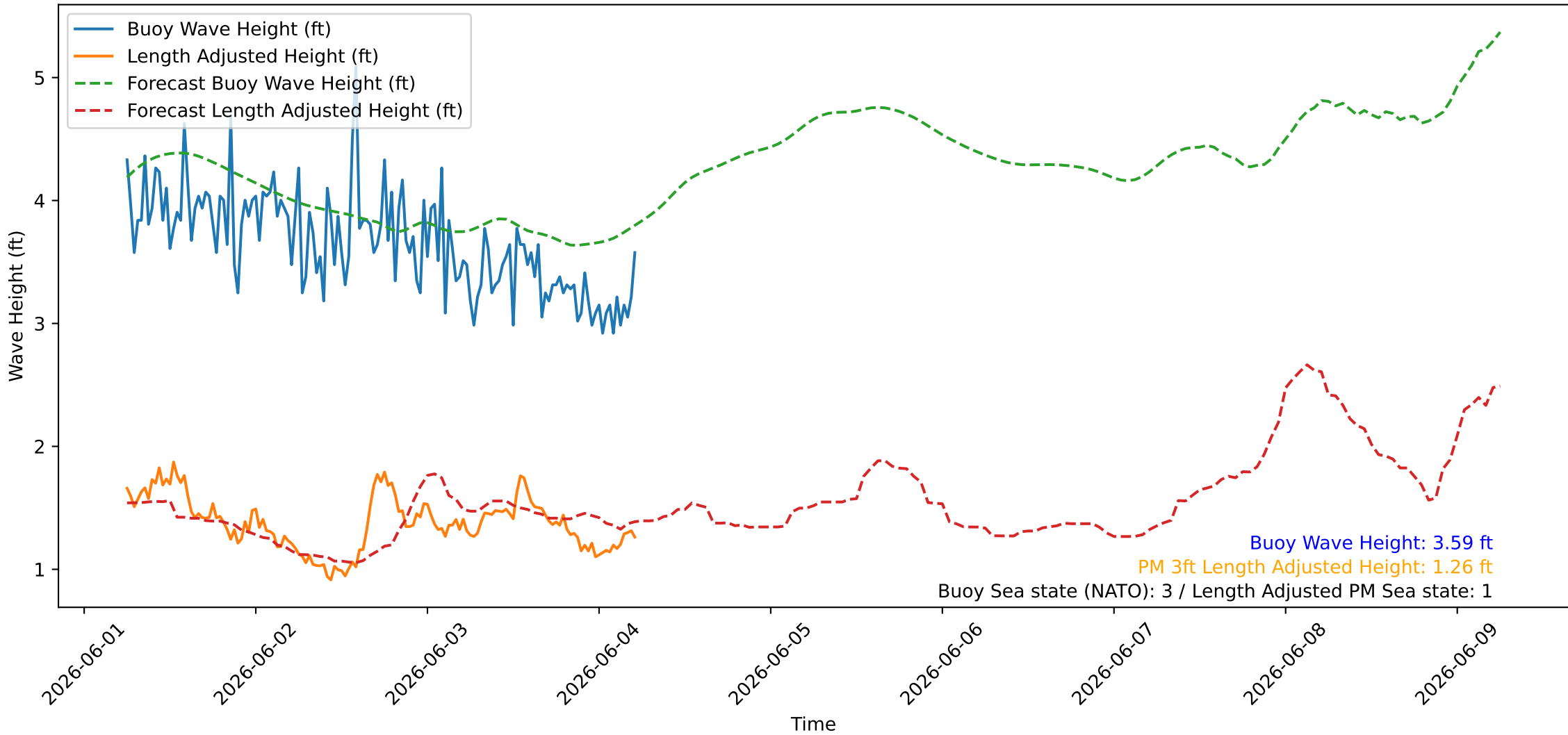
Wave Heights over Time for Oceanside Harbor at 2026-06-04 06:00:26
