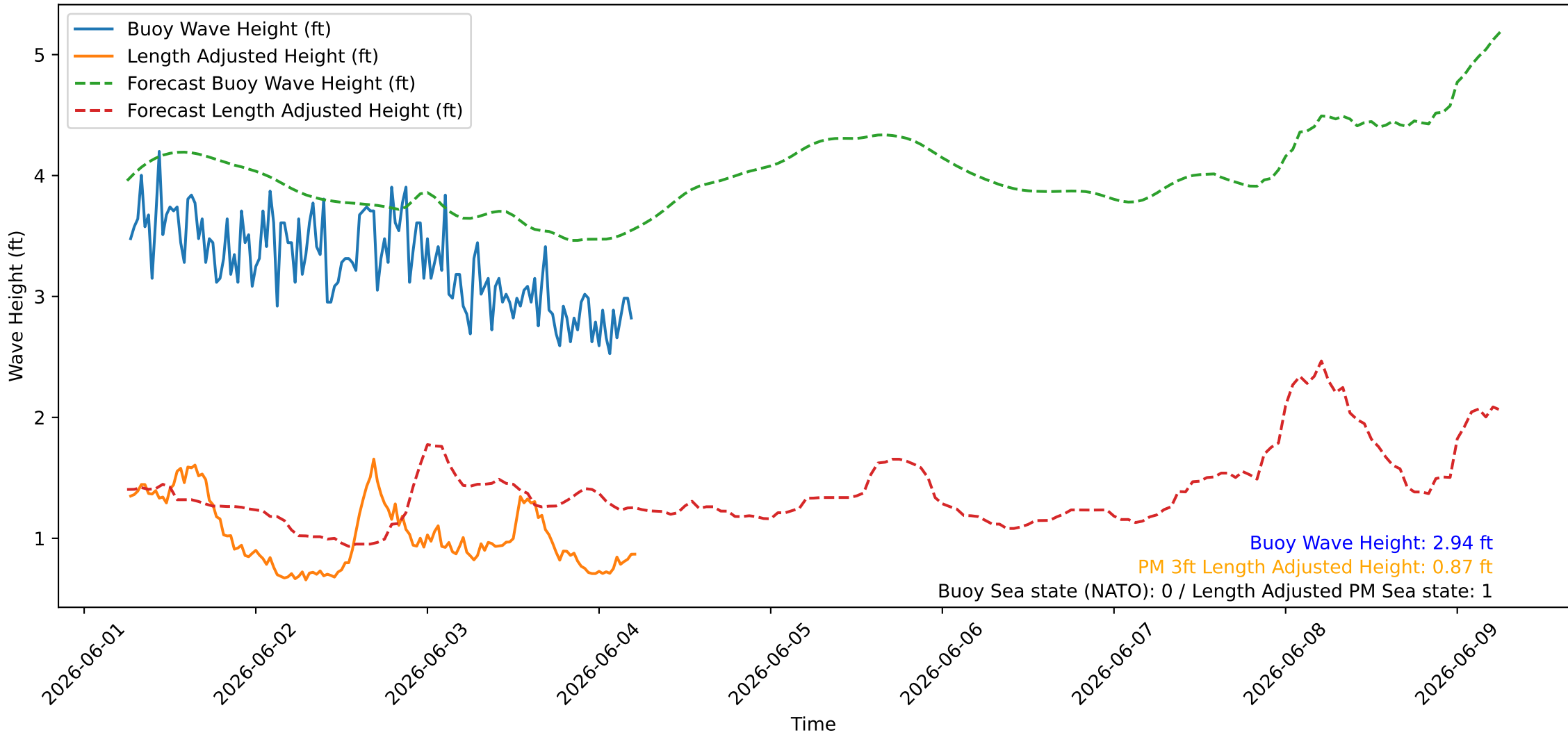
Wave Heights over Time for Red Beach at 2026-06-04 06:00:45
