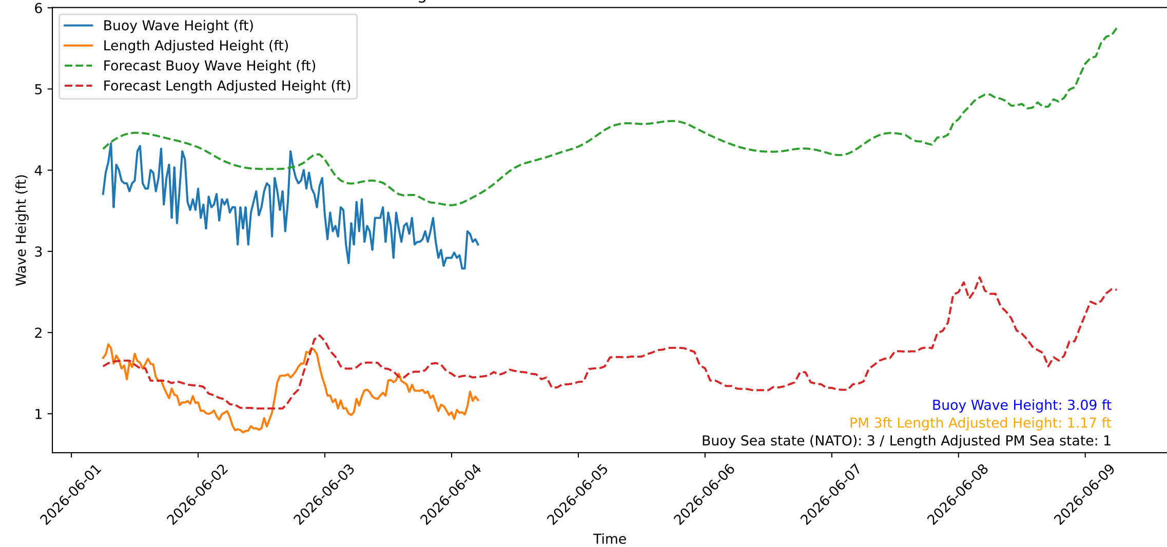
Wave Heights over Time for Green Beach at 2026-06-04 06:01:08
