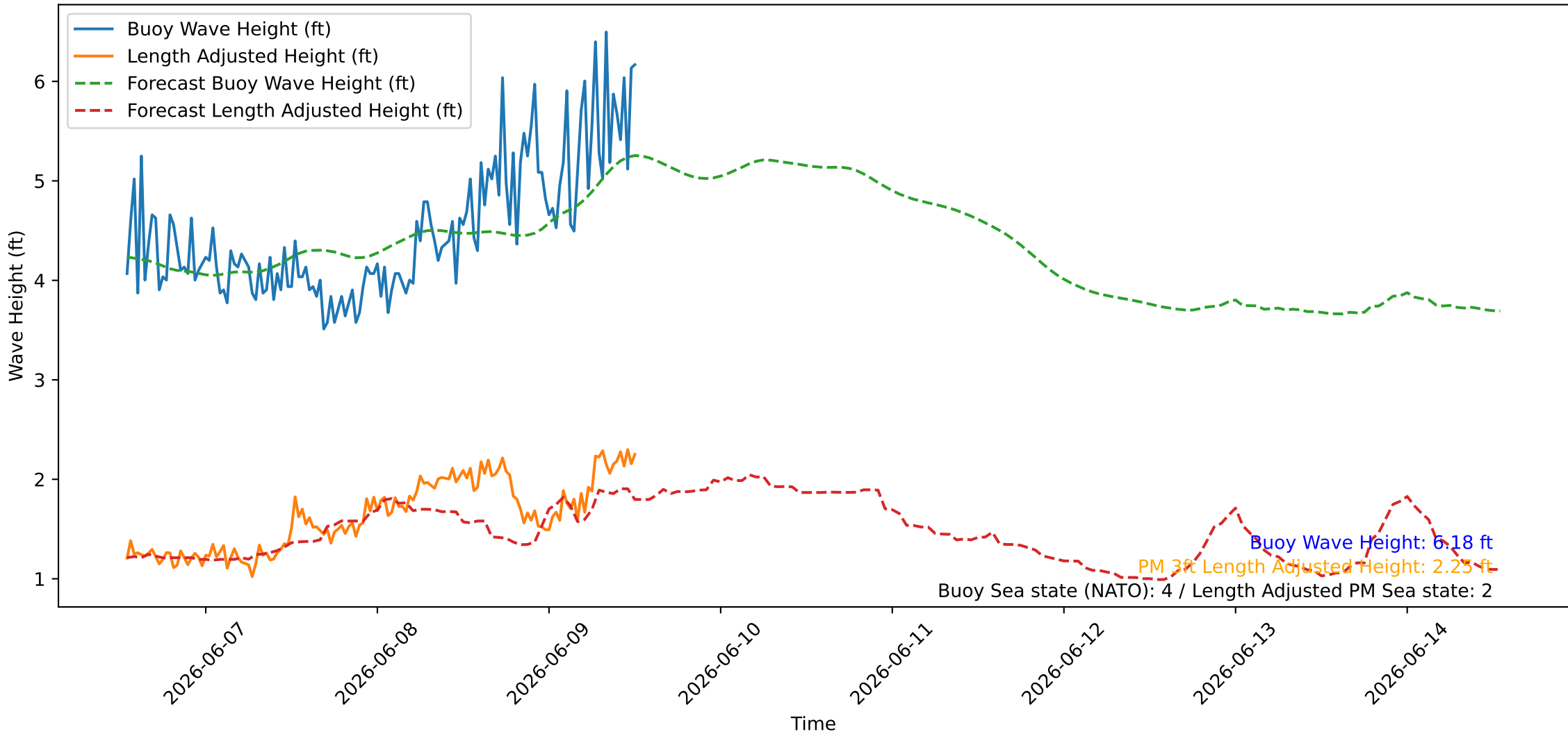
Wave Heights over Time for Oceanside Harbor at 2026-06-09 13:00:26
