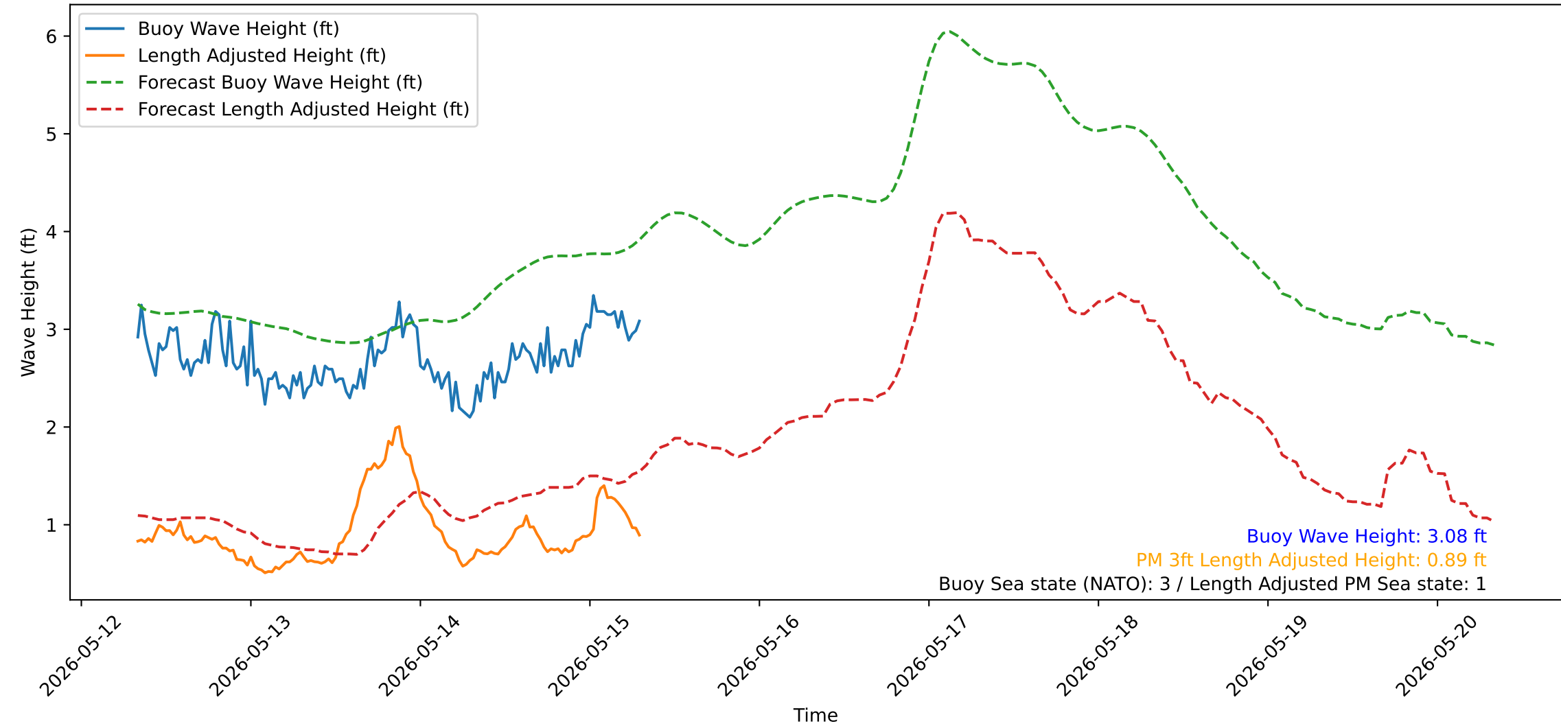
Wave Heights over Time for Green Beach at 2026-05-15 08:01:13
