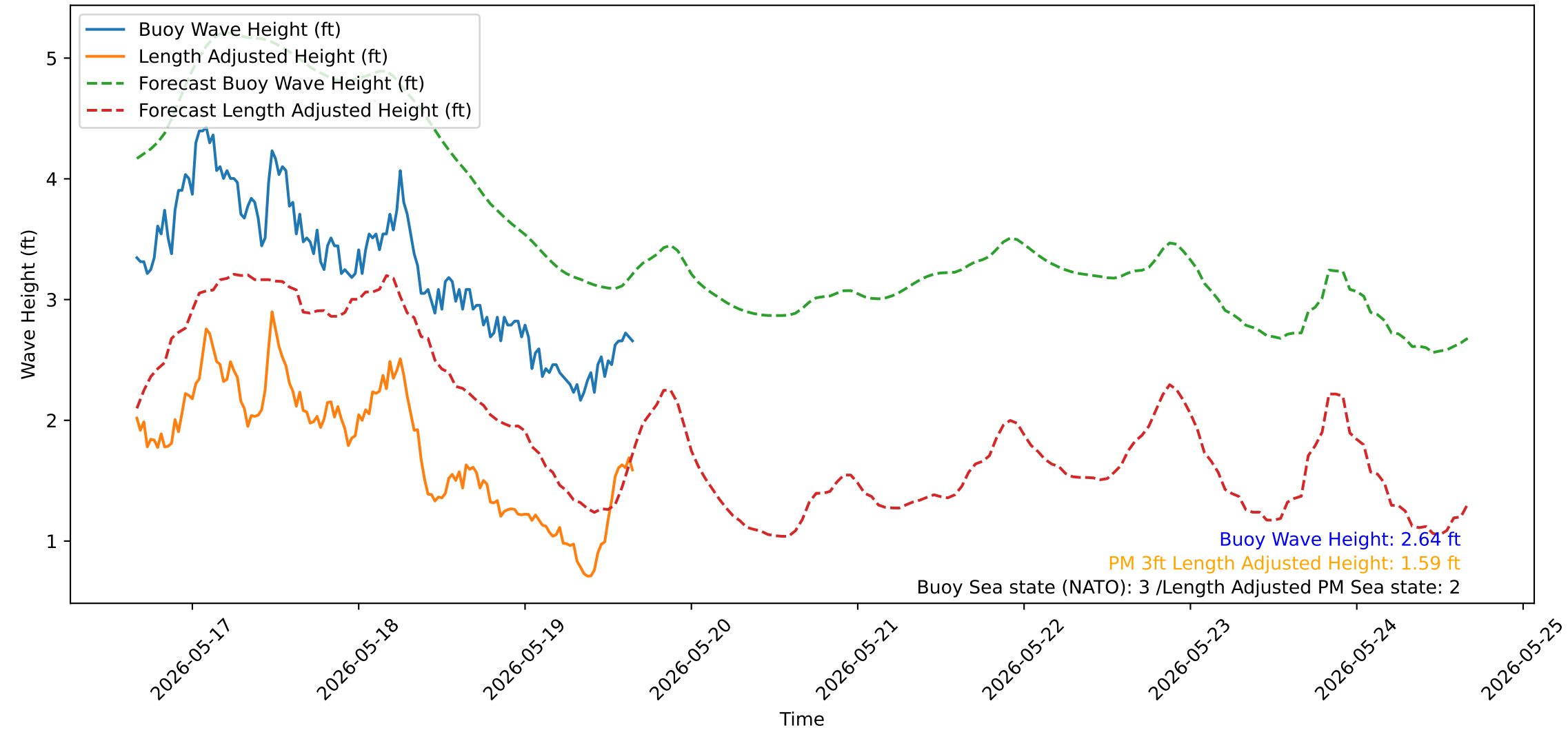
Wave Heights over Time for Green Beach at 2026-05-19 16:11:13
