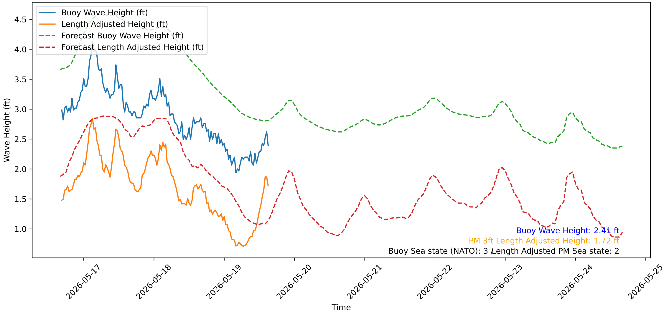
Wave Heights over Time for Red Beach at 2026-05-19 16:10:50
