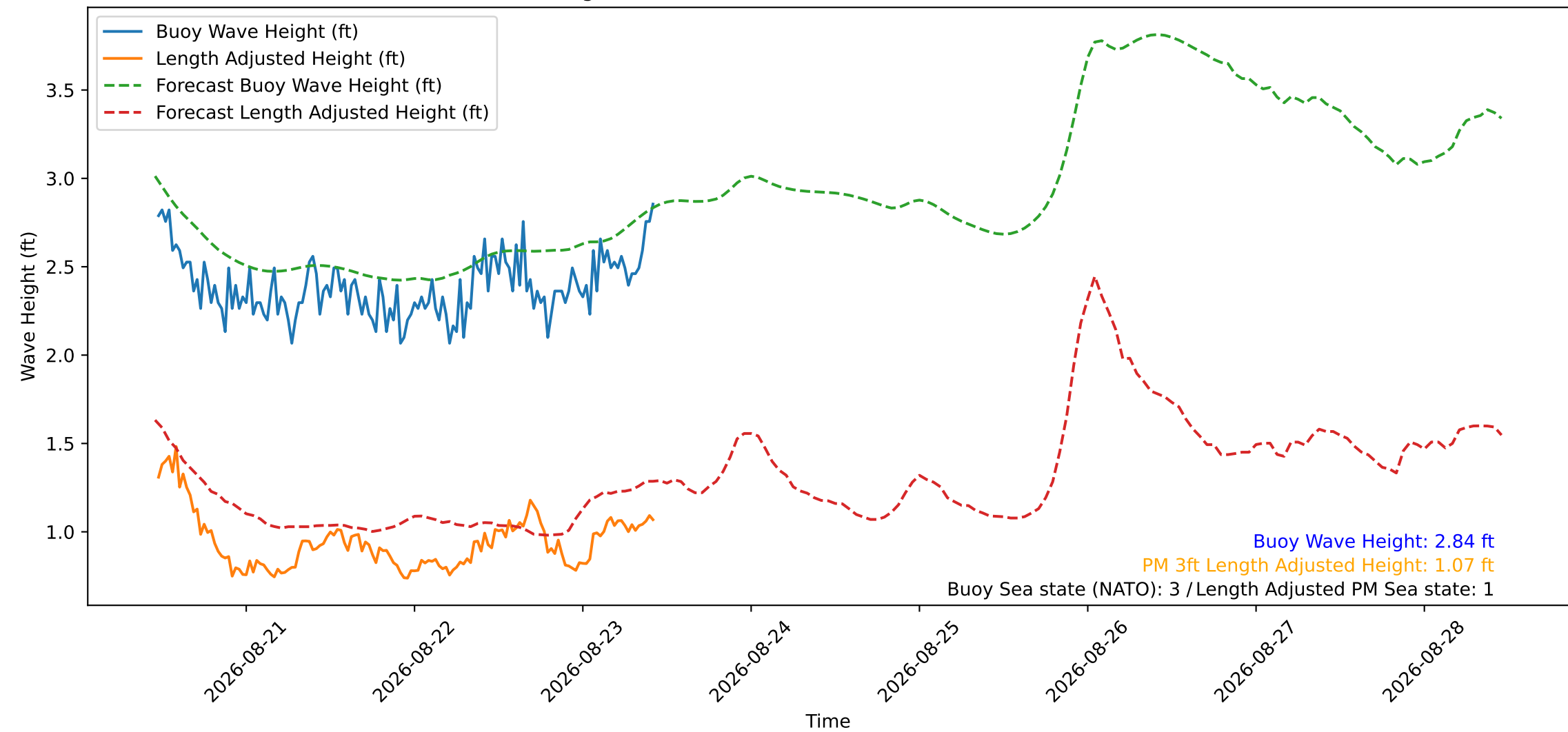
Wave Heights over Time for Red Beach at 2026-08-23 11:00:49
