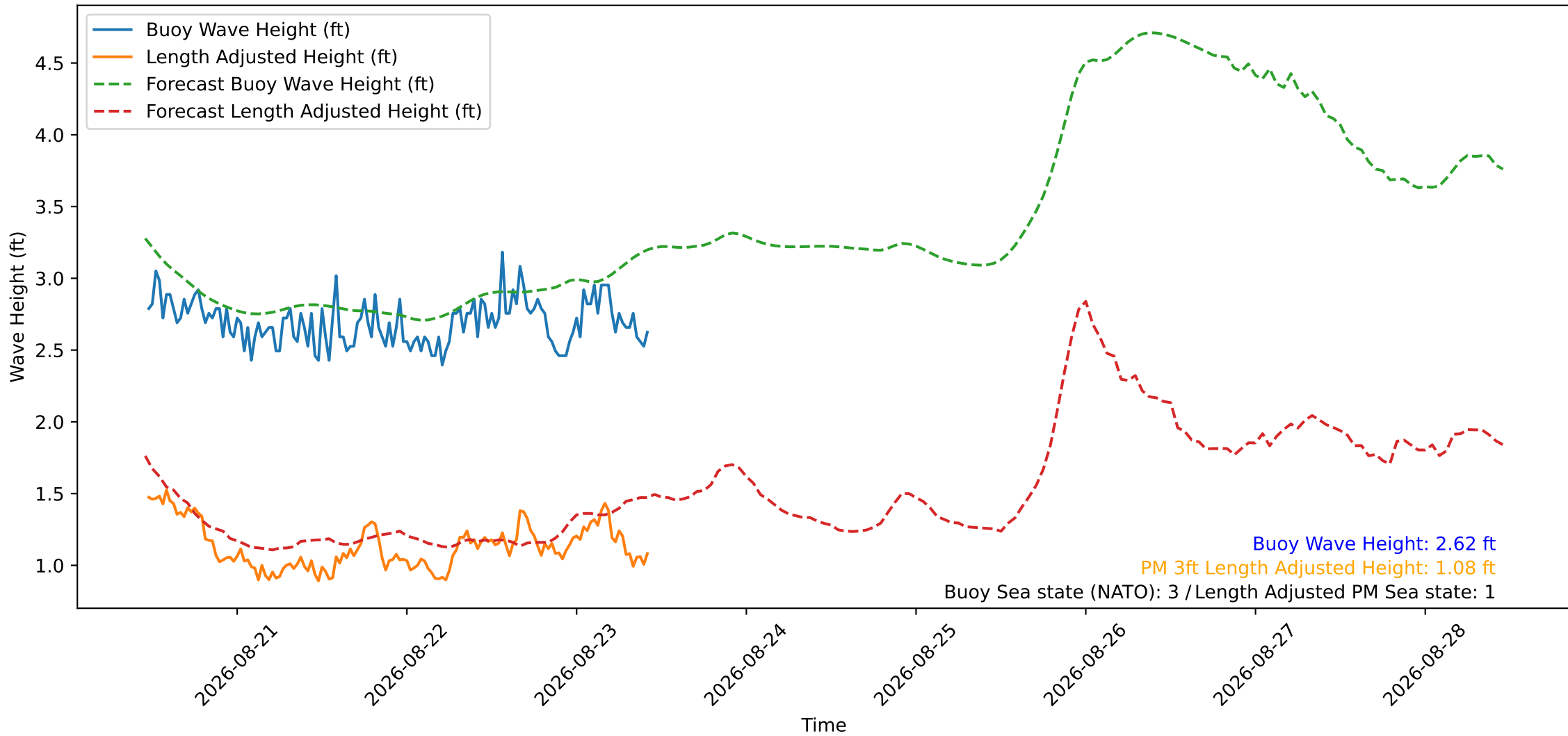
Wave Heights over Time for Green Beach at 2026-08-23 11:01:12
