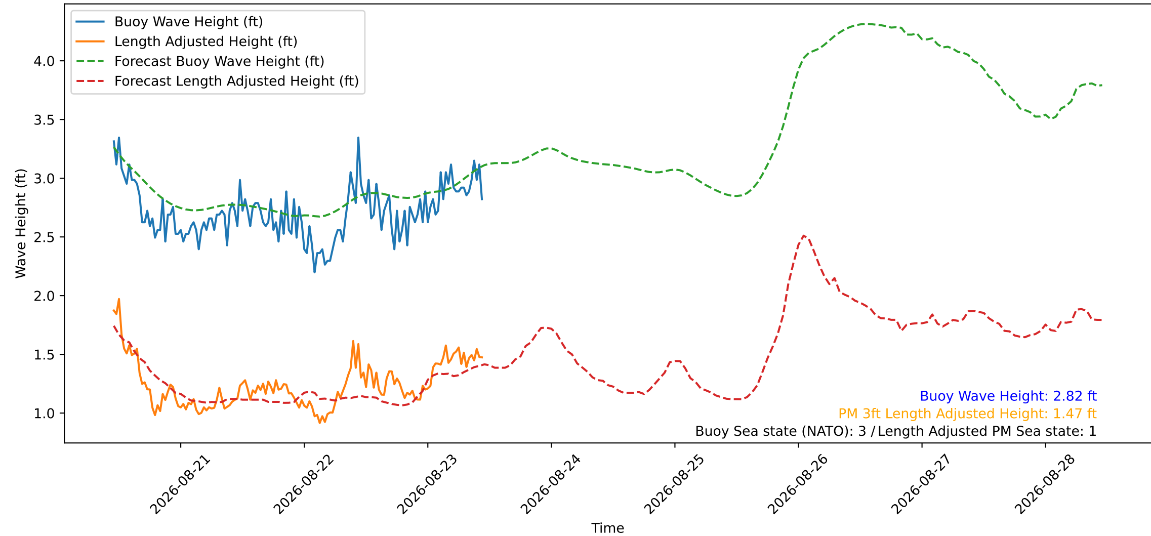
Wave Heights over Time for Oceanside Harbor at 2026-08-23 11:00:30
