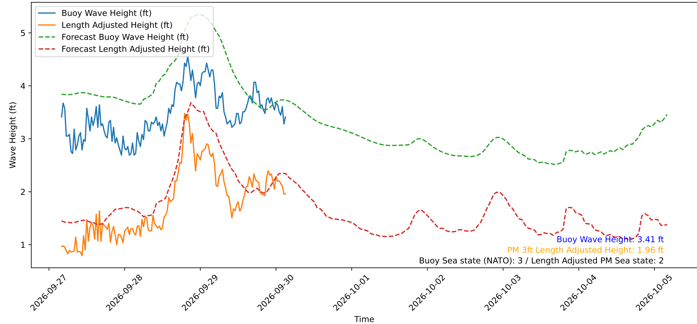
Wave Heights over Time for Green Beach at 2026-09-30 03:51:15
